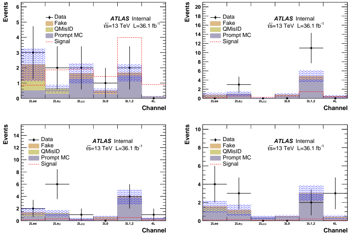
Fig. 6.1: The yields obtained in all analysis channels of the analysis for the signal regions m_{H^{++}} = 200, 300, 400 and 500 \text{ GeV} . Data is represented as point with errors, while the prediction of various components are represented as histograms. The error band represent the full uncertainty (statistic and systematic) of the total prediction. The signal prediction normalized to the luminosity of the analyzed data sample is represented as well.
