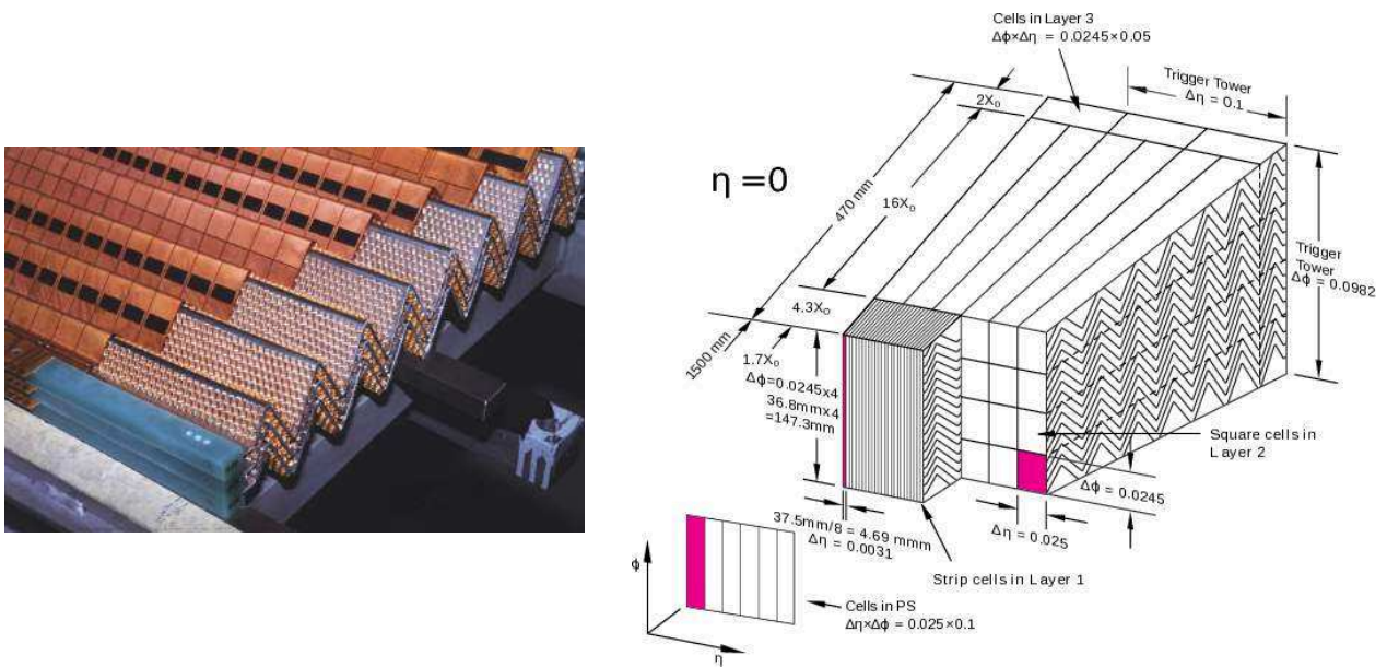
Fig. 3.12: The photographed accordion shape of LAr calorimeter (left), the honey-comb structured spacers are also visible. Sketch of a barrel module where the different layers are clearly visible with the ganging of electrodes in \phi (right). The granularity in \eta and \phi of the cells of each of the three layers and of the trigger towers is also shown.
