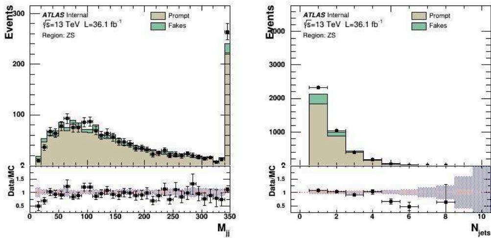
Fig. 5.20: Data compared to prediction for the di-jet invariant mass M_{jj} (left) and jet multiplicity N_{jet} (right) distributions in the Z -enriched (ZS) sample
