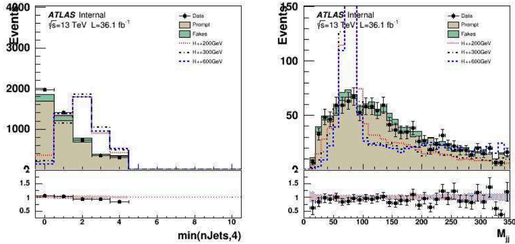
Fig. 5.14: Distributions in the WZ control region.
