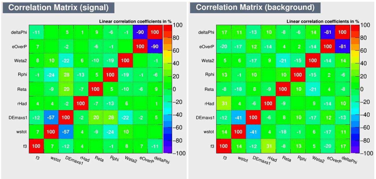
Fig. B.2: Correlation between the variables for the signal simulation (left) and the background simulation (right).
