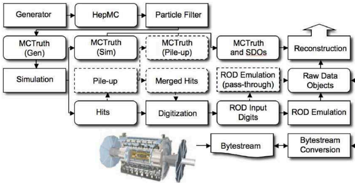
Fig. 3.17: The flow of the ATLAS simulation software, from event generators (top left) to reconstruction (top right). Algorithms are placed in square-cornered boxes and persistent data objects are placed in rounded boxes. The optional pileup portion of the chain, used only when events are overlaid, is dashed. Generators are used to produce data in HepMC format. Monte Carlo truth is saved in addition to energy depositions in the detector (hits). This truth is merged into Simulated Data Objects (SDOs) during the digitization. Also, during the digitization stage, Read Out Driver (ROD) electronics are simulated.
