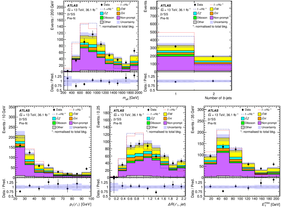
Figure 4.3.: Pre-fit distributions at \mathcal{B}(t \rightarrow Hq) = 0 for the five input variables to the 2\ell SS BDTs with highest separation of signal versus background. The distribution of the signal of t \rightarrow Hu and t \rightarrow Hc is shown normalised to the total background in red and blue, respectively [9].
