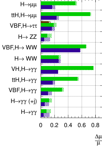
Figure 5.2.: (Left) ATLAS projection of relative uncertainty on the signal strength for different Higgs boson production and decay modes for L = 300 and 3,000 \text{ fb}^{-1} [143]. (Right) observed 95% CL limits on branching ratios of different top quark decays involving FCNC [130]. The projection to HL-LHC is added in pink following the references [141, 144] for t \rightarrow Hc and t \rightarrow Zc and [145] for t \rightarrow \gamma c . No extrapolation studies for t \rightarrow gc have been published so far.
