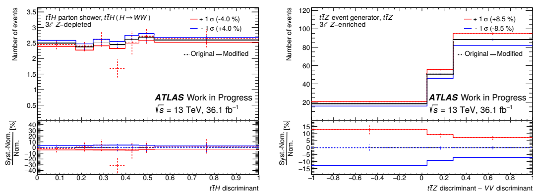
Figure 3.14.: Distribution of (left) the t\bar{t}H parton shower and hadronisation model systematic on t\bar{t}H sample with the H boson decaying to WW in the 3\ell Z -depleted SR and (right) the t\bar{t}Z event generator uncertainty on the t\bar{t}Z sample in the 3\ell Z -enriched CR. The black line indicates the nominal shape of the concerned sample and the red (blue) the 1\sigma up-(down-)variation of the systematic. The dotted lines show the distributions before the application of the smoothing procedure.
