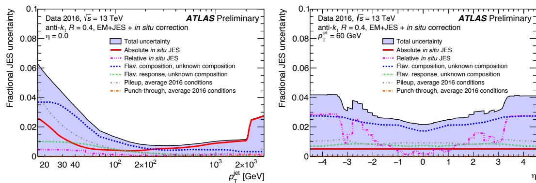
Figure 2.22.: Relative jet energy scale uncertainty in dependency of (left) p_T for jets at \eta = 0 and (right) \eta for jets at p_T = 60 \text{ GeV} in 2016 data for unknown flavour composition [97].
