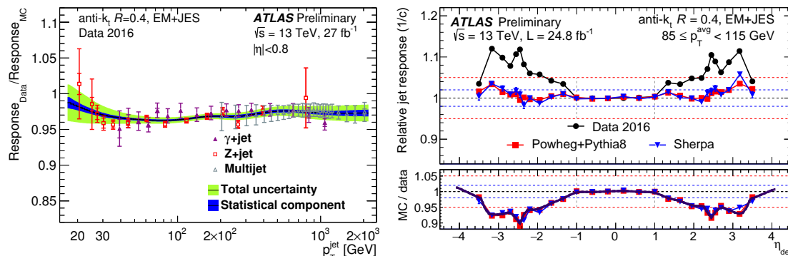
Figure 2.21.: Final residual in-situ jet energy calibration in 2016 data: (left) ratio of response in data to MC simulation in dependence of p_T and (right) relative jet response in dependence on \eta , measured with L = 27 \text{ fb}^{-1} and 24.8 \text{ fb}^{-1} respectively [97].
