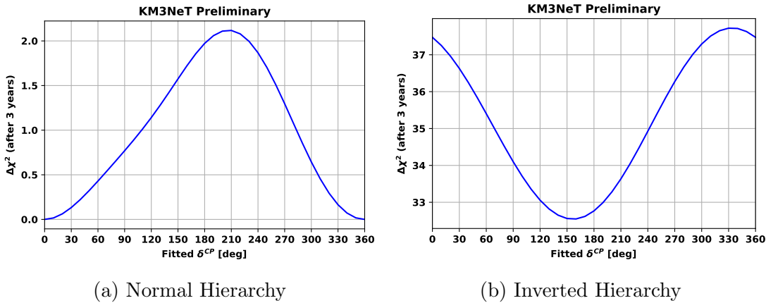
Figure 5.19: The \Delta\chi^2 after 3 years as a function of \delta^{CP} , with all other variables kept fixed, with respect to the assumed true values of \theta_{23} = 45^\circ , \delta^{CP} = 0^\circ and a normal hierarchy. Both the correct and opposite NMHs are shown, in order to show the sensitivity to \delta^{CP} when the NMH is correctly identified and its behaviour when the wrong hierarchy is fitted. It can be seen that ORCA is not able to measure the CP phase with a competitive significance, but that the uncertainty on \delta^{CP} does reduce the sensitivity to the NMH.
