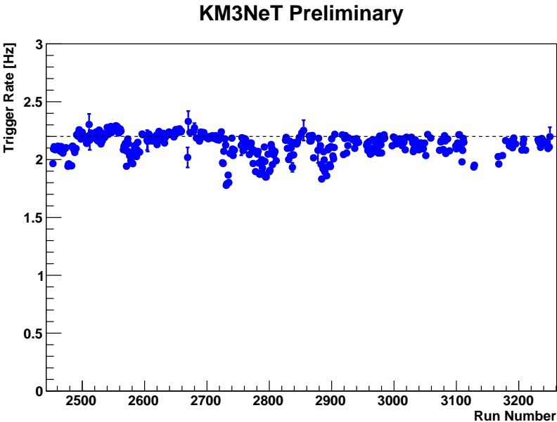
Figure 4.2: The triggered event rate as a function of run number for selected physics runs taken between September and December of 2017. The dotted line shows the expected average rate from atmospheric muons.
