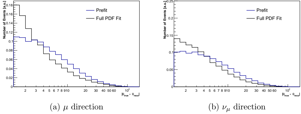
Figure 3.9: The zenith uncertainty in degrees for \nu_{\mu} -CC interactions, weighted with the unoscillated Honda flux, reconstructed with the full ORCA detector, where the reconstructed track begins inside the detector volume. It is shown with respect to both the neutrino direction and outgoing muon direction for the prefit and full PDF fit stages of the reconstruction chain.
