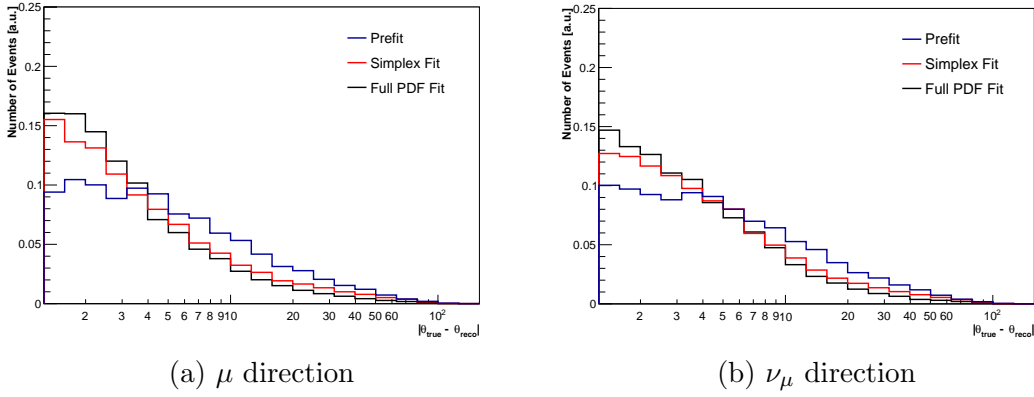
Figure 3.7: The zenith uncertainty in degrees for \nu_{\mu} -CC interactions, weighted with the unoscillated Honda flux, reconstructed with a single ORCA line. It is shown with respect to both the neutrino direction and the outgoing muon direction for the first three stages of the reconstruction chain.
