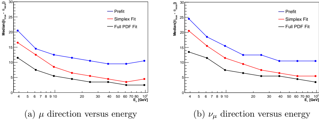
Figure 3.8: The median zenith uncertainty in degrees for \nu_{\mu} -CC interactions, weighted with the unoscillated Honda Flux, reconstructed using a single ORCA line. It is shown with respect to both the neutrino direction and the outgoing muon direction for the first three stages of the reconstruction chain.
