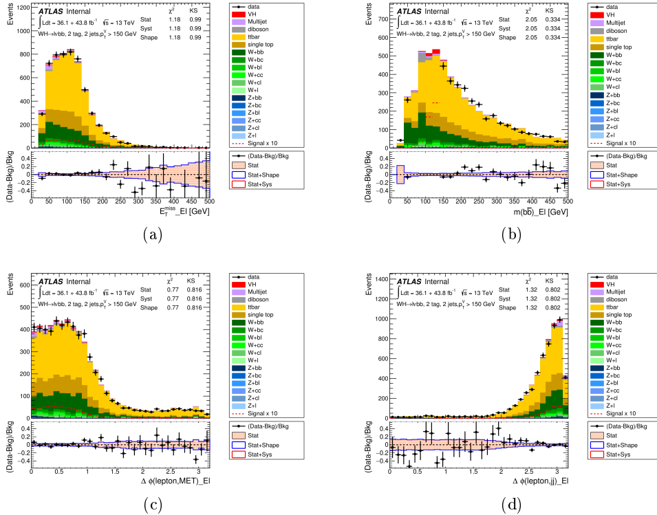
Figure 12.5: The distributions, for the 2-tag 2-jet p_T^W > 150 \text{ GeV} category in electron channel W+HF signal region, of (a) E_T^{miss} (b) m_{bb} (c) \Delta\phi(lepton, E_T^{miss}) and (d) \Delta\phi(lepton, bb) are shown.
