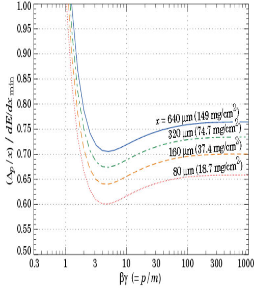
Figure 4.8: Most probable energy loss in silicon \delta p per unit thickness ( x ), scaled to the mean loss of a minimum ionizing particle, 388 \text{ eV}/\mu\text{m} ( 1.66 \text{ MeV } g^{-1} \text{cm}^2 )[55].
