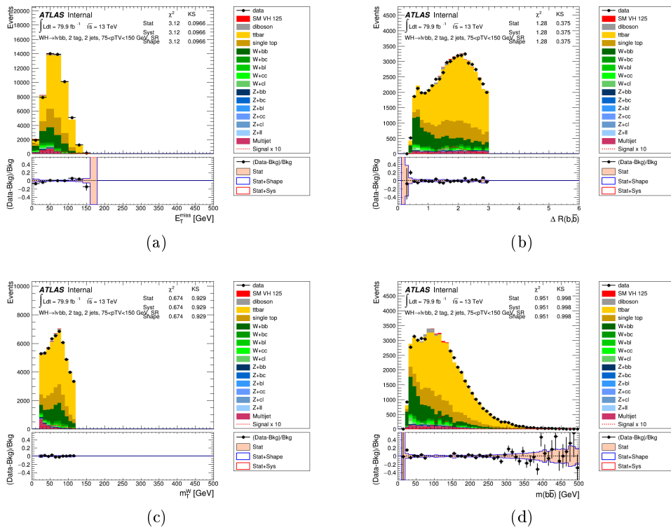
Figure 12.12: The distributions, for the 2-tag 2-jet 75 \text{ GeV} < p_T^W < 150 \text{ GeV} category, of (a) E_T^{miss} (b) \Delta R(b\bar{b}) (c) m_T^W and (d) m_{b\bar{b}} are shown. The electron and muon channels are combined.
