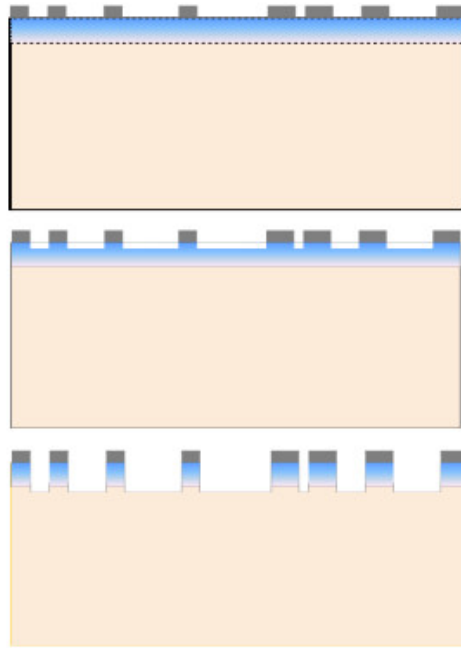
Figure 6.20: Schematic cross section of TLM sample illustrating the etching process for n-times of doped layers (blue region) until reaching the silicon substrate (beige region).
