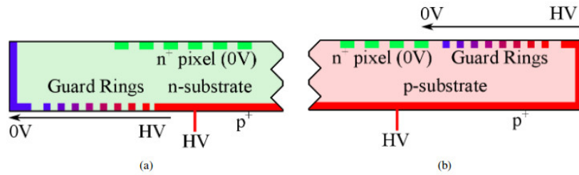
Figure 5.2: (a) n^+ -in- n sensor design with an n-type bulk and n^+ implants. The guard rings are located on the backside. (b) n^+ -in- p sensor design with a p-type bulk and n^+ implants [73]. The guard rings are on the topside.
