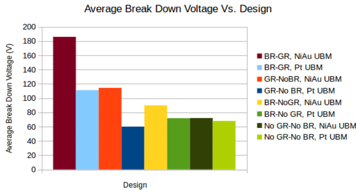
Figure 5.23: Average breakdown voltage for different design, comparing NiAu UBM and Pt UBM.
