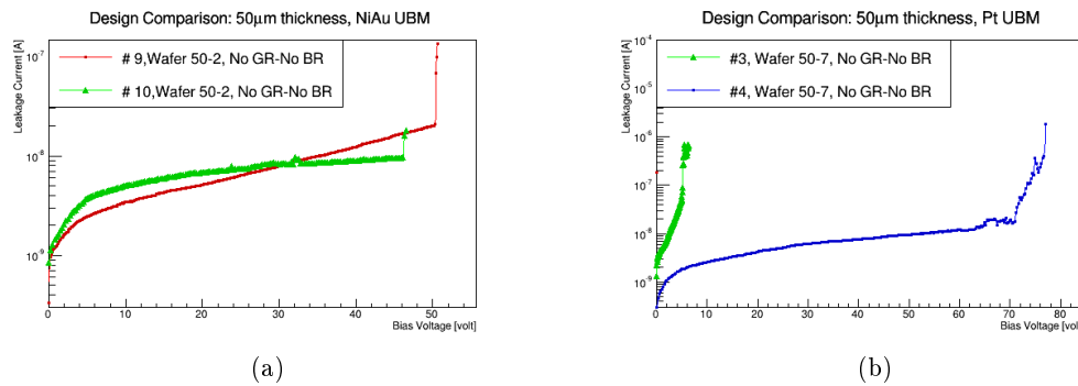
Figure 5.17: IV-measurement for different design variations for all the structures with 50 \mu\text{m} thickness and NiAu UBM (a), Pt UBM (b). Semi-logarithmic scale is used.
