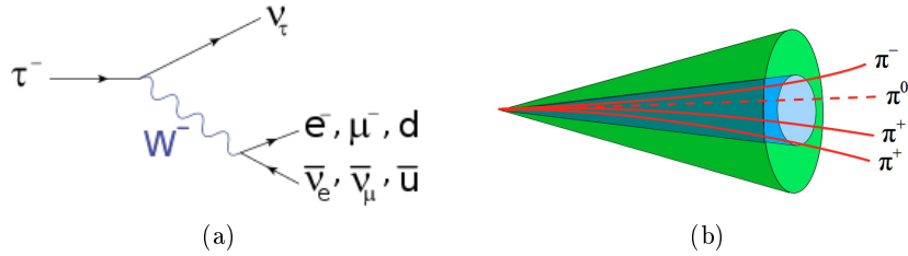
Figure 11.4: (a) Feynman diagram of the tau leptonic decay by the emission of an off-shell W boson. (b) Typical signature of a hadronic tau decay.
