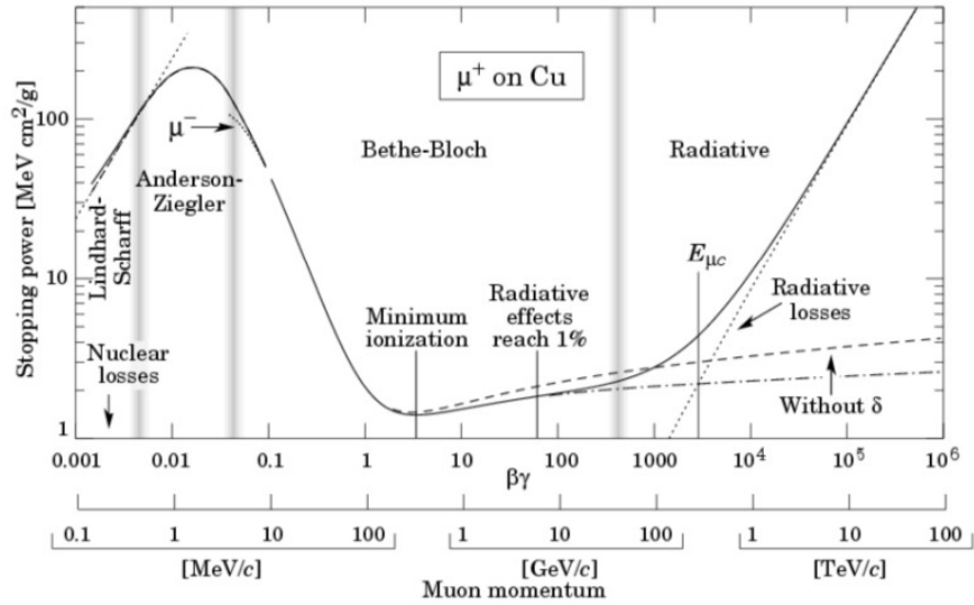
Figure 4.5: The stopping power for positive muons in copper as a function of the muon momentum [54]. The solid line is the total stopping power of the muon. [55]
