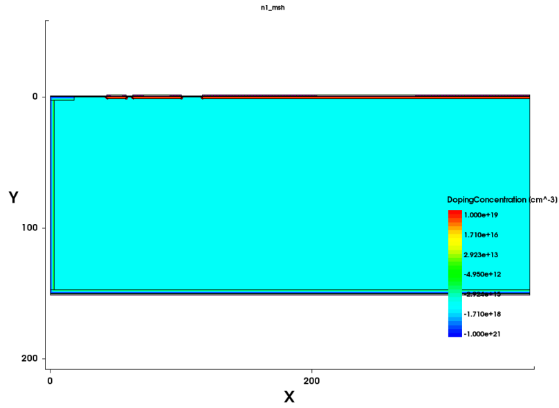
Figure 6.9: Overall view of the simulated n^+ -in-p active edge pixel structure showing dopant concentration profile. Sensor geometrical size is 400\mu\text{m} in the x-direction and 150\mu\text{m} in the y-direction.
