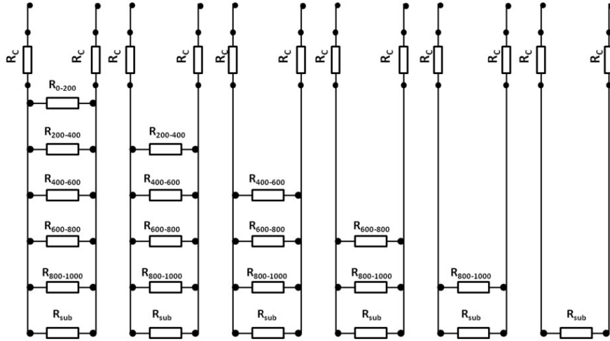
Figure 6.23: Resistance in-depth measurement used in this study. Repetively, a small layer of implant is etched, using Reactive Ion Etching (RIE), and the resistance at different depths is measured until reaching the substrate.
