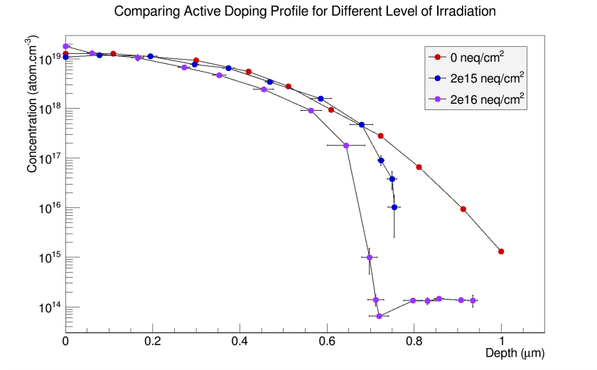
Figure 6.30: TLM measurement of the active carrier concentration as a function of depth for non irradiated sample (red curve) compared to two irradiated samples of 2 \times 10^{15} \text{ neq/cm}^2 (blue curve) 2 \times 10^{16} \text{ neq/cm}^2 (Violet curve) neutrons irradiation fluences.
