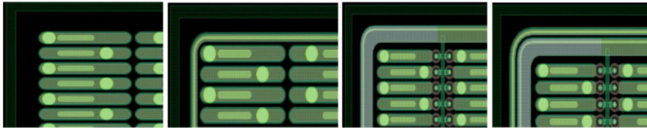
Figure 5.14: The four design variations of the active edge production. From left to right: no Guard Ring - no Bias Rail design, no Bias Rail - one Guard Ring design, no Guard Ring - one Bias Rail design and one Guard Ring - one Bias Rail design.
