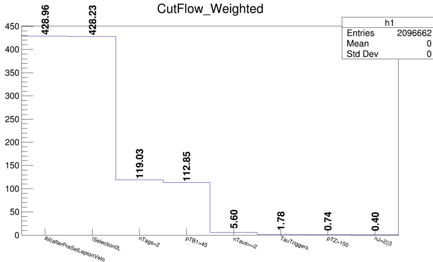
Figure 11.9: Weighted Cutflow for the event selected in the ThadThad channel.
