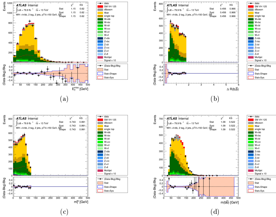
Figure 12.11: The distributions, for the 2-tag 2-jet p_T^W > 150 GeV category, of (a) E_T^{miss} (b) \Delta R(b, \bar{b}) (c) m_T^W and (d) m_{b\bar{b}} are shown. The electron and muon channels are combined.
