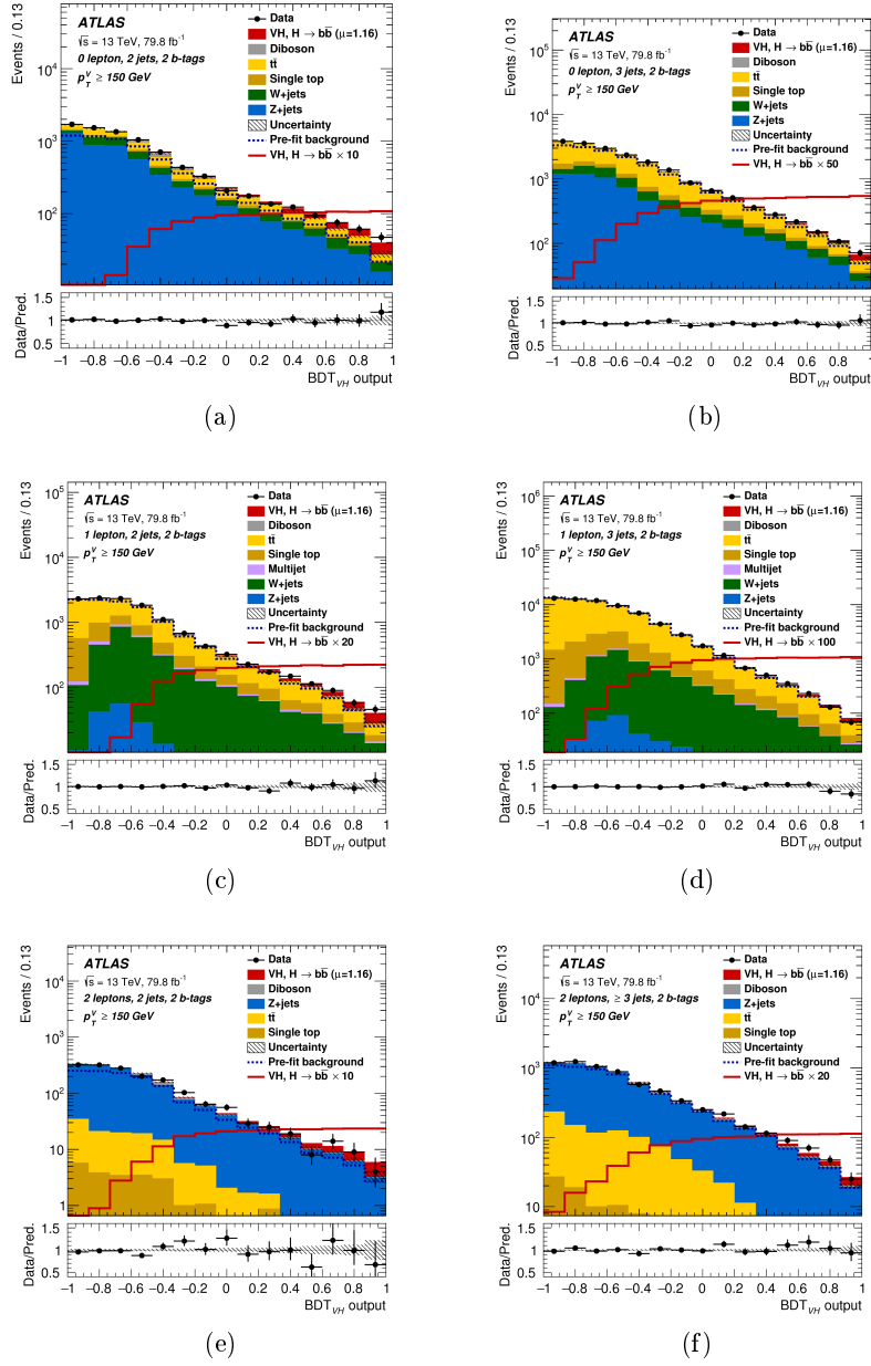
Figure 10.3: The \text{BDT}_{\text{VH}} output post-fit distributions in the 0-lepton (top), 1-lepton (middle) and 2-lepton (bottom) channels for 2-b-tag events, in the 2-jet (left) and exactly 3-jet (or \geq 3 jets for the 2-lepton case) (right) categories in the high- p_T^V region. The background contributions after the global likelihood fit are shown as filled histograms. The Higgs boson signal ( m_H = 125 GeV) is shown as a filled histogram on top of the fitted backgrounds normalised to the signal yield extracted from data ( \mu = 1.16 ), and unstacked as an unfilled histogram, scaled by the factor indicated in the legend. The dashed histogram shows the total pre-fit background. The size of the combined statistical and systematic uncertainty for the sum of the fitted signal and background is indicated by the hatched band. The ratio of the data to the sum of the fitted signal ( \mu = 1.16 ) and background is shown in the lower panel. The \text{BDT}_{\text{VH}} output distributions are shown with the binning used in the global likelihood fit.
