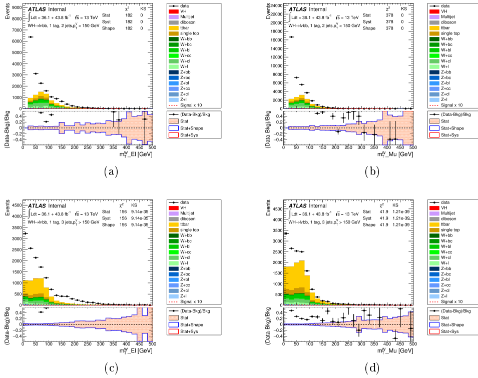
Figure 12.2: The m_T^W distribution in the inverted isolation 1-lepton 75 \text{ GeV} < p_T^W < 150 \text{ GeV} region, requiring exactly 1 b-tag with 2 signal jets in e channel(a), 2 signal jets in \mu channel(b), 3 signal jets in e channel(c), 3 signal jets \mu channel(d).
