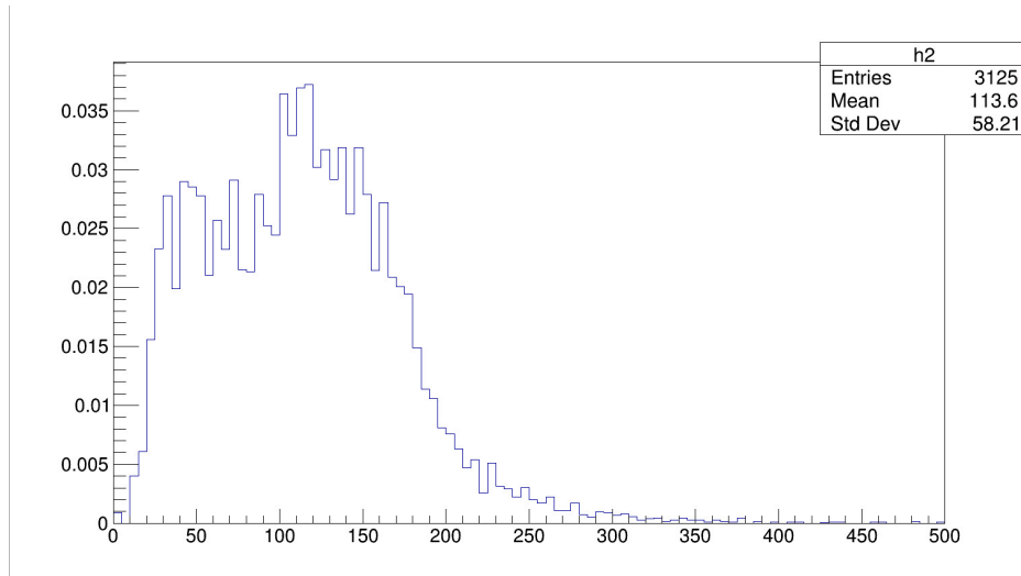
Figure 11.15: The transverse momentum distribution of the Z boson ( p_T^Z ) in the selected events in the \tau_{lep}\tau_{had} channel for nJets=2
