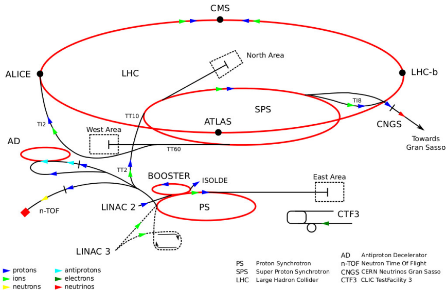
Figure 2.3: The CERN Accelerator Complex showing all experiments around the LHC.
