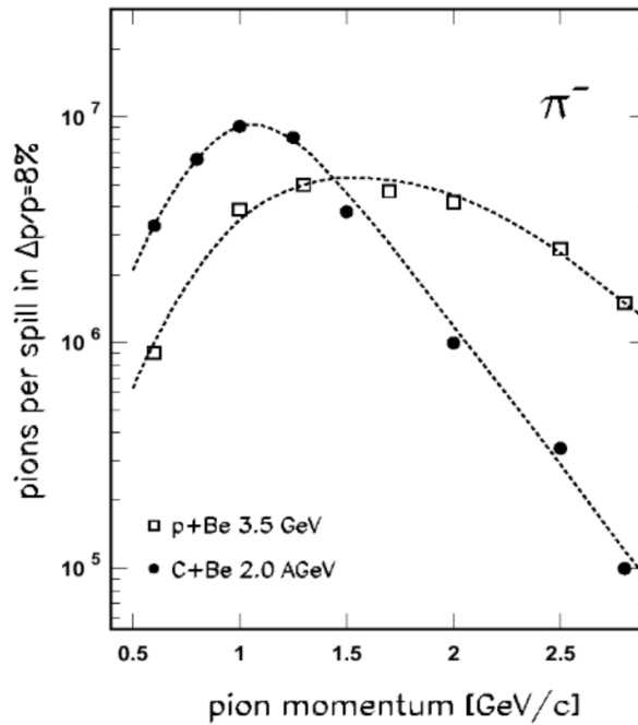
Figure 72: Pion beam intensities available at GSI for production by the reaction p+Be at 3.5 GeV and C+Be at 2 GeV.
