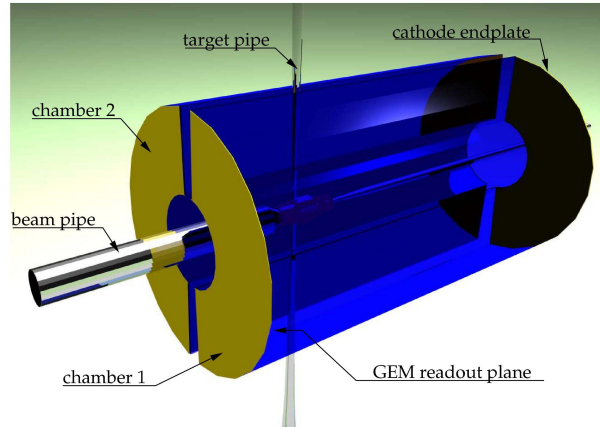
Figure 80: The Time Projection Chamber.
