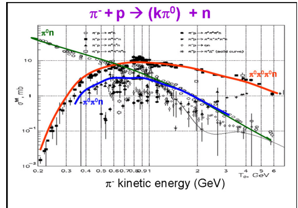
Figure 117: Cross sections for different \pi^0 production channels of the \pi^-p reaction.
