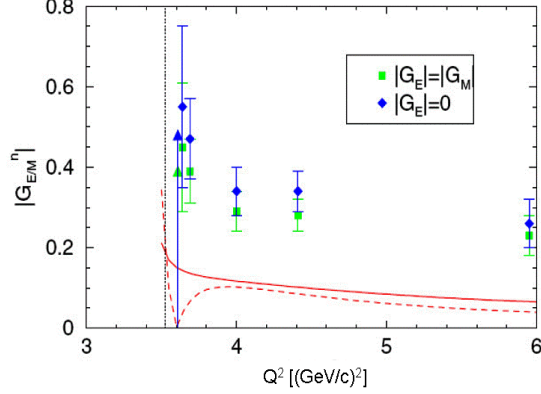
Figure 102: Neutron magnetic form-factor derived from the FENICE experiment [198] using the hypothesis |G_E|=|G_M| (squares) and |G_E|=0 (diamonds). The dotted vertical line shows the n-\bar{n} threshold. The curves are Chiral Perturbative Theory calculations [199] for |G_M| (solid line) and |G_E| (dashed line).
