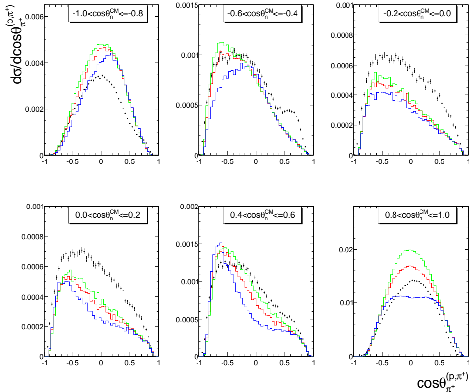
Figure 56: \pi^+ angular distribution in the (\pi^+, p) system for different neutron angle bins. the curves correspond to PLUTO simulations with different anisotropy parameters B of the decay angular distribution 1+B \cos^2\theta (green: B=0 , red: B=0.65 and blue: B=3 )
