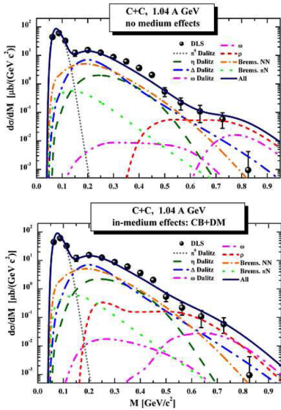
Figure 42: HSD calculations [80] compared to DLS experimental spectra measured in C+C system at 1 AGeV. Top: vacuum calculation. Bottom: in-medium calculation.
