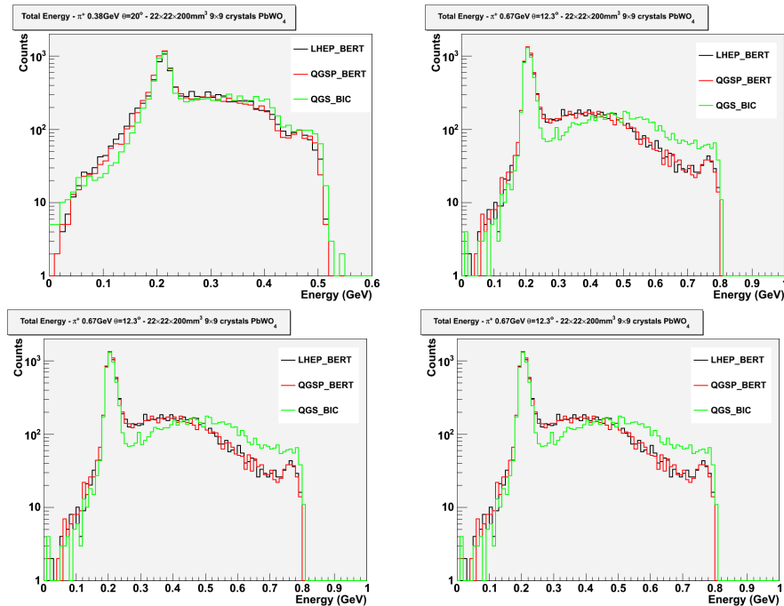
Figure 123: Same condition as fig.121, with comparison of \pi^+ fot LHEP (black), QGSP-BERT (red), QGSP-BIC (green) physics lists.
