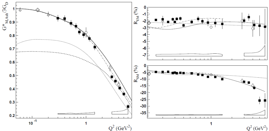
Figure 20: Left panel: the form-factor G_M for the N- \Delta(1232) transition normalized by the dipole form-factor ( G_D(Q^2)=1/(1+Q^2/0.71)^2 ). Right panel: the ratios R_{EM} and R_{SM} of respectively the electric and charge amplitudes to the magnetic amplitudes. The data points are from MAMI, MIT/Bates and Jlab [78]. The curves represent different models.
