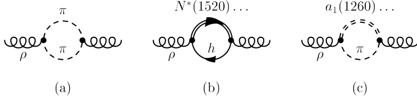
Figure 9: Dressing of the \rho in the nuclear medium via 2\pi propagator (a), coupling to baryonic resonances (b), coupling to mesonic resonances (c).
