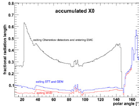
Figure 125: Distribution of material budget measured in radiation length units, as a function of polar angle.
