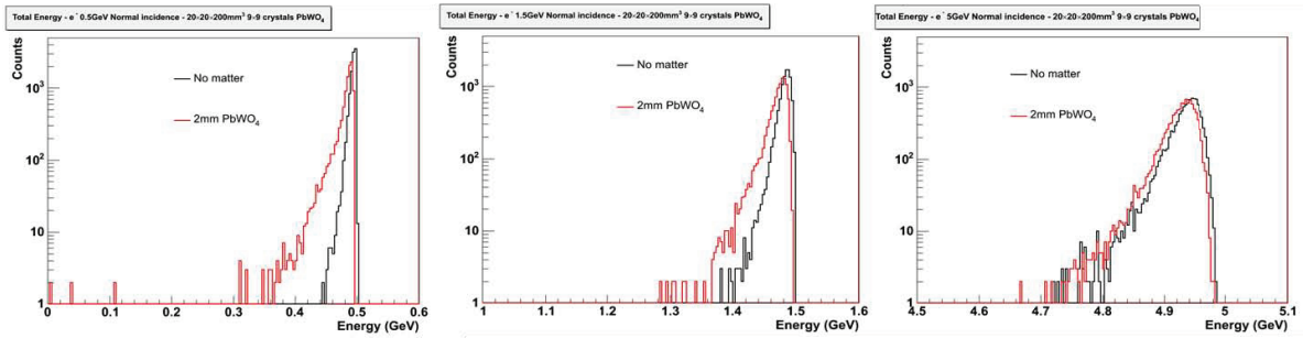
Figure 124: Effect of a 2 mm \text{PbWO}_4 slab ( X/X_0=0.2 ) on the energy deposit of an electron at different momenta
