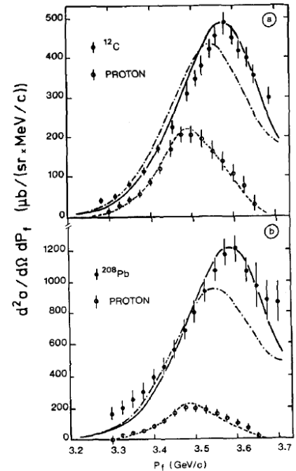
Figure 8: Comparison of theory [20] to experiment [21] for \Delta excitation in ^{12}\text{C} and ^{208}\text{Pb} by the (^3\text{He},t) reaction at 2 GeV and 0^\circ triton angle. The full and dot-dashed curves correspond respectively to calculations with and without \Delta -hole correlations.
