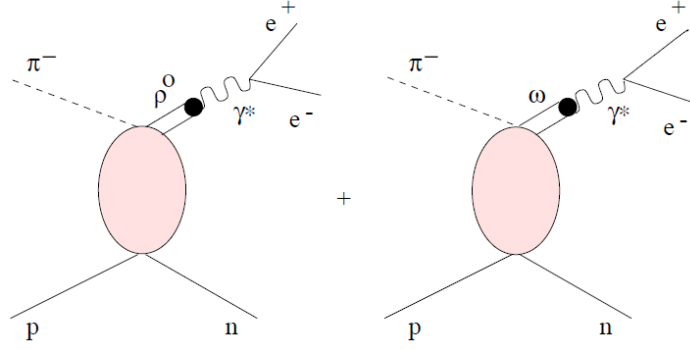
Figure 68: Sketch for the \pi N \rightarrow \rho(\omega) N amplitude.
