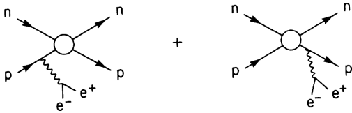
Figure 27: Sketch for the Soft Photon Approximation
