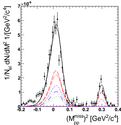
Figure 58: Missing mass spectrum of two protons for the pp e^+ e^- events after subtraction of a multipion background. The lines show the predictions from the PLUTO event generator using the resonance model [58]. The solid black lines are the sum of all contributions. For the \pi^0 , the short-dashed line (green) is the N^*(1520) , the long dot-dashed (blue) line is the N^*(1440) , the short-dot-dashed (violet) is the non-resonant production and the long dashed red line is the \Delta(1232) contribution. For the \Delta(1232) , the thin line corresponds to a decay angular distribution in 1+3\cos^2\theta and the thick line to the standard PLUTO option (see sec.2.5.2). For the \eta , the short dot-dashed (violet) line is the non-resonant production and the long dashed (red) line corresponds to the N^*(1535) .
