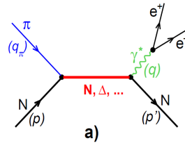
Figure 67: s-channel graphs for \pi -N reactions
