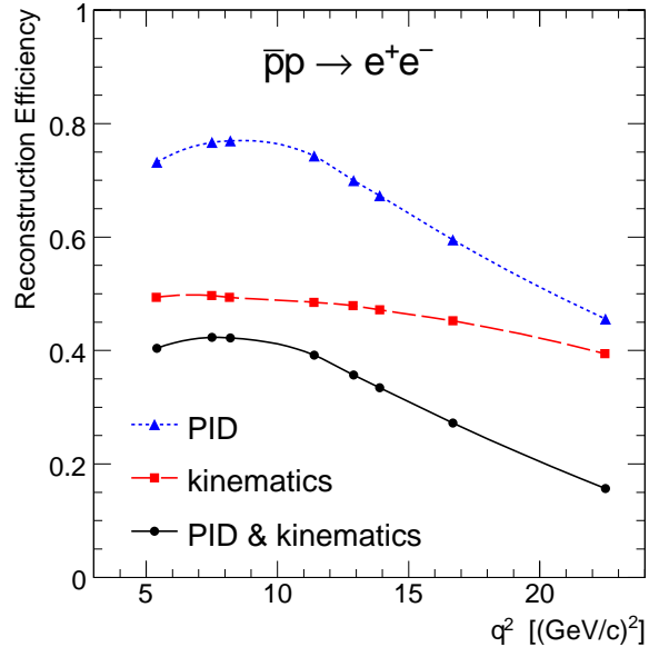
Figure 134: Average reconstruction efficiency as a function of q^2 (black solid line). The effect of applying kinematical constraints (red dashed line) and PID cuts (blue dotted line) are shown separately.
