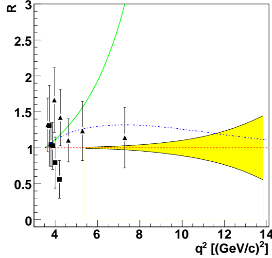
Figure 135: The yellow band shows the expected statistical precision on the determination of the ratio R, in the case R=1, as a function of q^2 , compared with the existing data from Curves are theoretical predictions, as described in the text.
