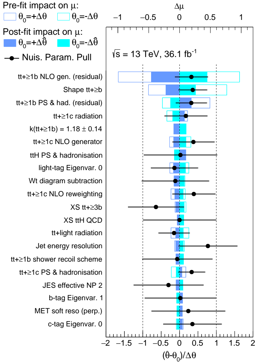
Figure 5.37.: Ranking of the nuisance parameters used in the fit according to their impact on sensitivity. Only the 20 first ones are shown. The filled (open) blue rectangles correspond to the post(pre)-fit contribution of the systematic to the uncertainty on the signal strength and is read on the upper axis. The horizontal bar on the black points show the post-fit uncertainties after applying the constraints from the fit and can be read on the bottom axis. The post(pre)-fit impact on sensitivity is computed performing the fit fixing the nuisance parameter at the post(pre)-fit \pm 1\sigma variation and taking the difference in the fitted \mu with the default fit.
