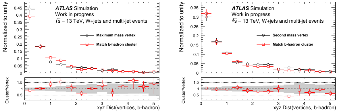
Figure 3.17.: Distance of the maximum mass (left) and second highest mass (right) clusters/vertices to the truth- b -hadron in the (x, y, z) volume. The black distribution is obtained using only the two highest mass vertices while red points are obtained from vertex clusters.
