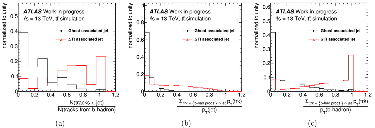
Figure 3.8.: Association of the b -hadron tracks to b -jets for \Delta R -associated-truth-jet and the ghost-associated-truth-jet in case of close-by-jets. In this case the same b -hadron is associated to two jets depending on the association scheme. (a) number of tracks originating from the b -hadrons associated to the jet divided by the number of b -hadron tracks. (b) ratio of the fraction of b -hadron track p_T in the jet to the jet p_T . (c) ratio of the fraction of b -hadron track p_T in the jet to the b -hadron p_T .
