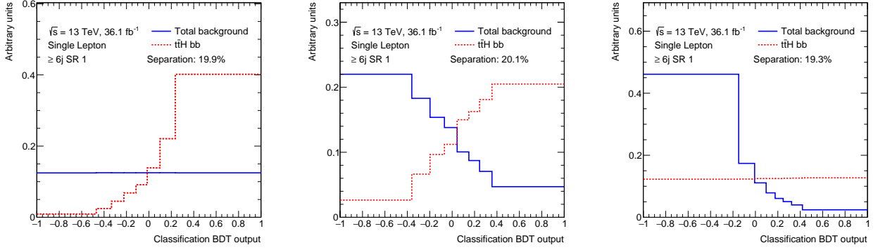
Figure 5.5.: Normalized distributions of the classification BDT output distributions for the total background (blue line) and t\bar{t}H(H \rightarrow b\bar{b}) signal (dashed red line) in the \geq 6j SR1 category. The binning is computed with the automatic binning function Z for 8 bins with z_s = 0 and z_b = 8 (left), z_s = z_b = 4 (middle), z_s = 8 and z_b = 0 (right).
