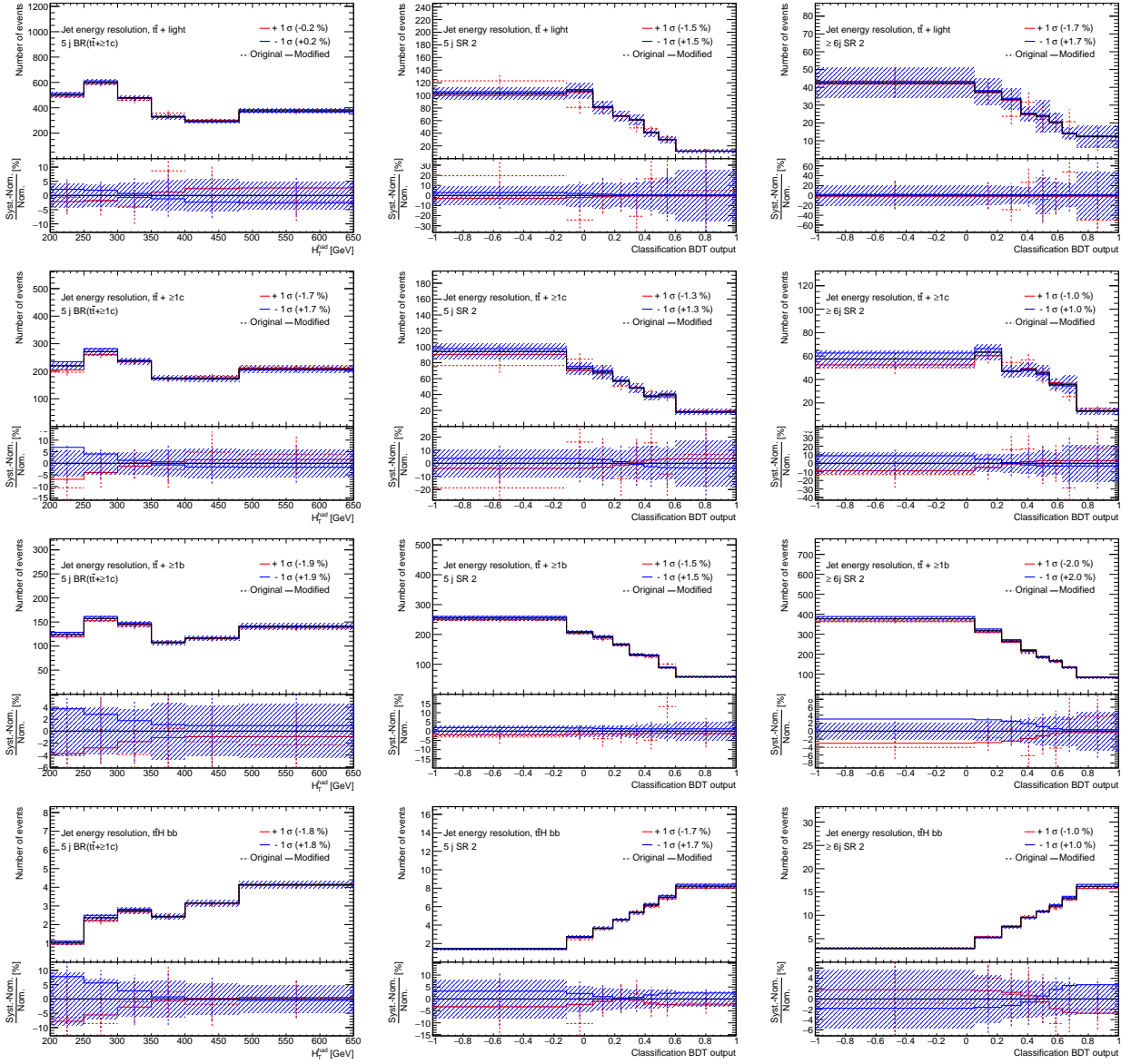
Figure 5.33.: Monte Carlo prediction of the t\bar{t} + light (top), t\bar{t} + \geq 1c (second row), t\bar{t} + \geq 1b (third row) backgrounds and the t\bar{t}H(H \rightarrow b\bar{b}) signal (bottom) including the \pm 1\sigma variations induced by the jet energy resolution uncertainty in the 5j BR( t\bar{t} + \geq 1c ) (left), 5j SR2 (middle) and \geq 6j SR2 (right) categories. Colored points (solid lines) display the systematic uncertainty before(after) smoothing. The main-smoothing is used in these plots.
