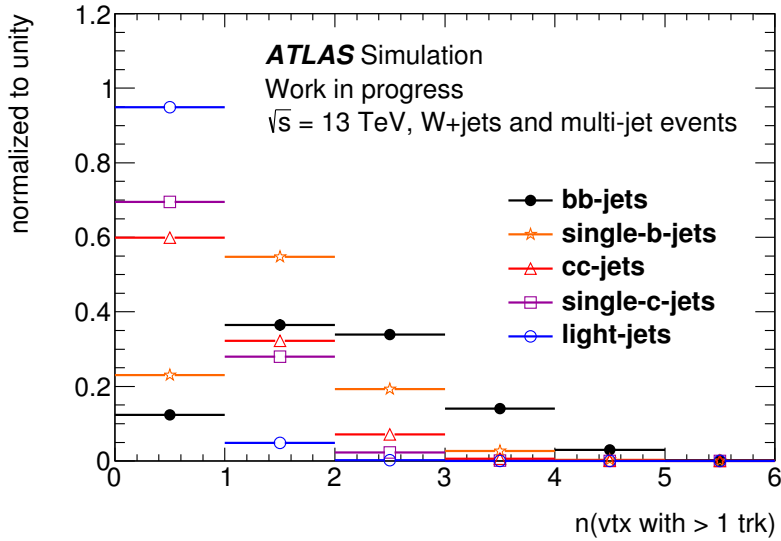
Figure 3.14.: Number of vertices for different jet flavours in a mixture of di-jet and W+jets events.
