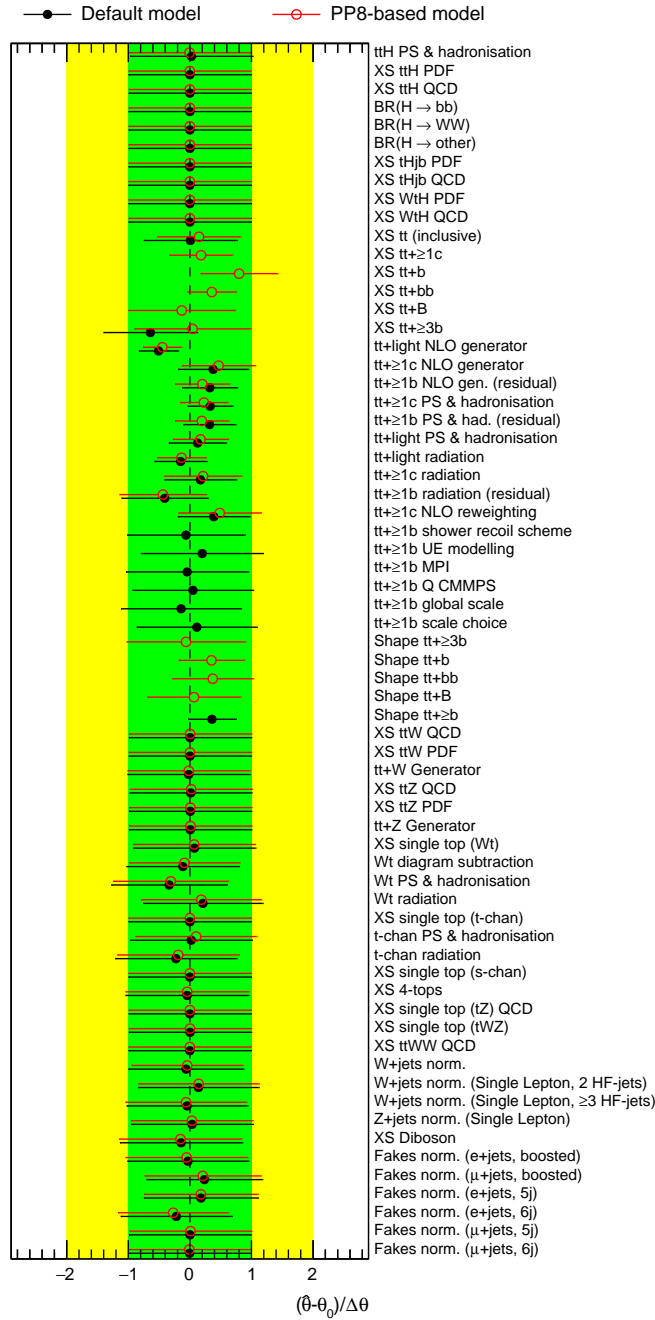
Figure 5.30.: Post-fit theoretical systematic uncertainties from the fit to data. The black points display the values obtained from the default fit. The red points are obtained from the fit to data with the alternative t\bar{t} + \geq 1b model. The green (yellow) area represent the \pm 1(2)\sigma band on the pre-fit systematic uncertainty. The position of the black points and the size of their horizontal bars give the pulls and constraints in units of standard deviation, respectively.
