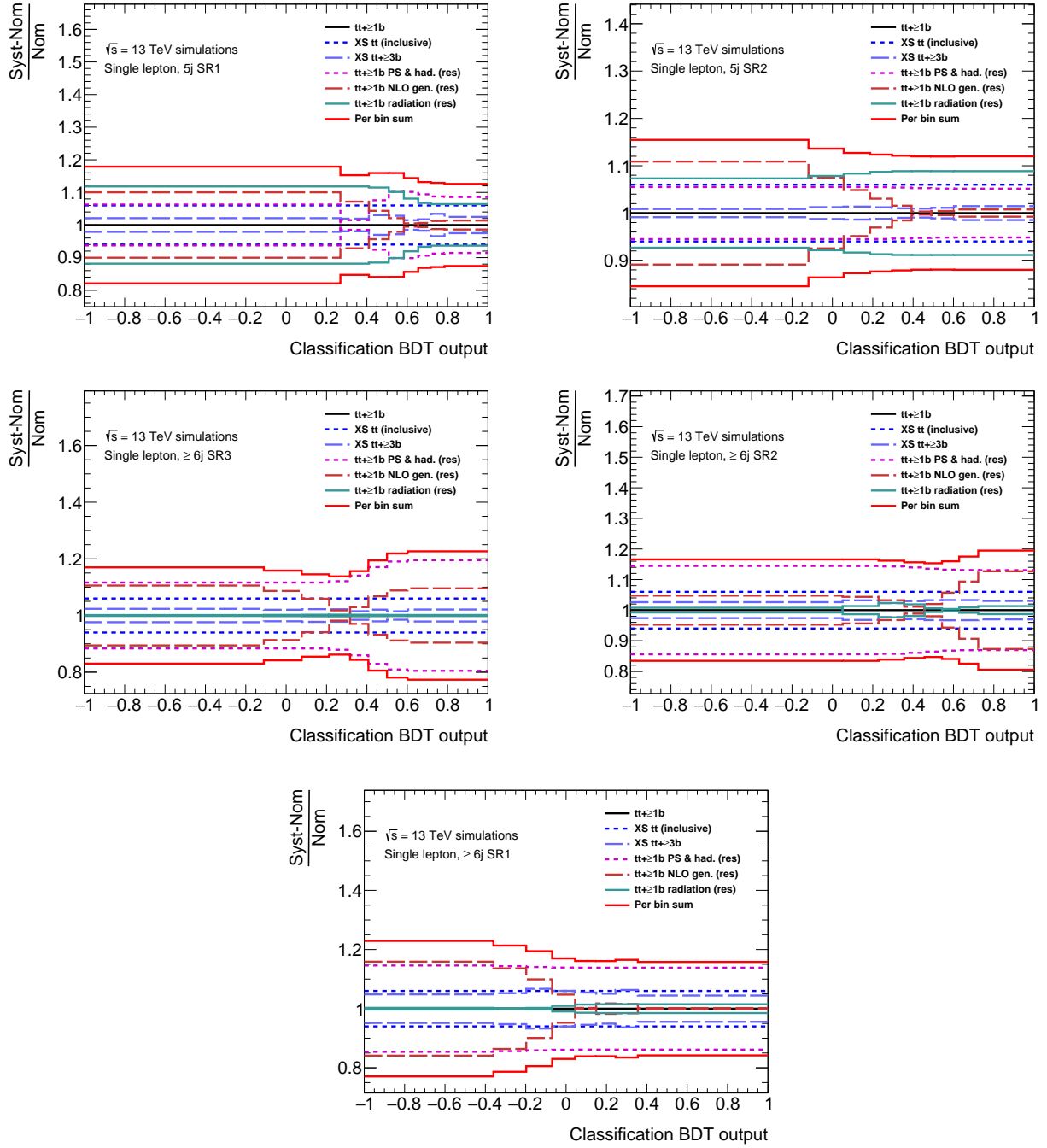
Figure .45.: Relative variations induced by the tt \geq 1b systematic uncertainties on the tt \geq 1b sample at \pm 1\sigma for the classification BDT distribution in the signal-enriched categories. The PP8-based tt \geq 1b model is used. Uncertainty on the tt cross section, the 50% normalisation uncertainty of the tt \geq 3b sub-component and various MC to MC comparison uncertainties. The red lines show the quadratic sum of the up and down effects systematic uncertainties in each bin.
