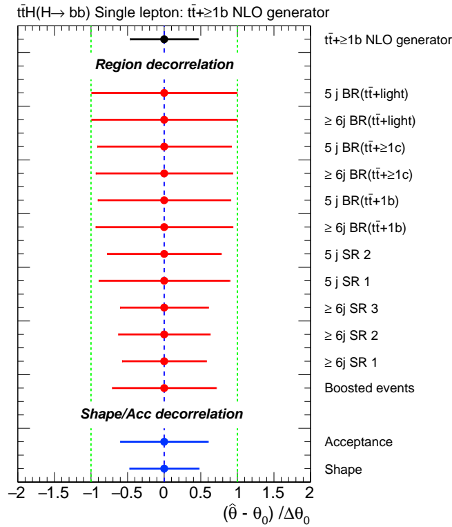
Figure 5.11.: Post-fit uncertainties on the various components of the t\bar{t}+\geq 1b NLO generator systematic. They are obtained from the fits using different decorrelation schemes: (black) default fit with all components correlated, (red) uncorrelated per process, (blue) uncorrelating the normalisation and shape components of the nuisance parameter.
