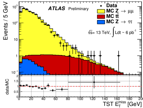
Figure 2.29.: Distribution of the reconstructed missing energy in Z \rightarrow \mu\mu selected events. Run 2 data (black points) is compared to the cumulative distribution of predictions from processes passing the selections [126].
