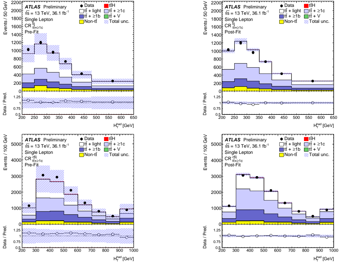
Figure 5.20.: Comparison of the predicted H_T^{\text{had}} distribution to the one observed in data in the t\bar{t}+\geq 1c -enriched categories of the single lepton channel. (left) before applying the corrections from the fit, (right) after applying the corrections from the fit. The hashed area represent the statistical and systematic uncertainties. The pre-fit uncertainties do not include the effect of the t\bar{t}+\geq 1b and t\bar{t}+\geq 1c normalisations which are free parameters of the fit. Note that the y -axis range in the lower pad (ratio plot) is twice smaller in the right plots compared to the ones on the left.
