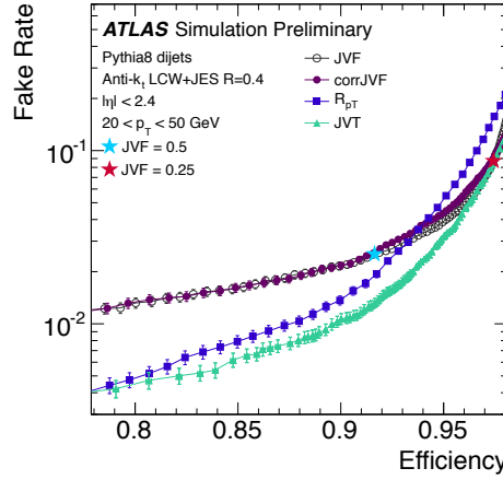
Figure 2.28.: Fake rate from pileup jets versus hard-scatter jet efficiency curves for JVF, corrJVF, R_{p_T} , and JVT. The figure and definitions of all variables are found in [124].
