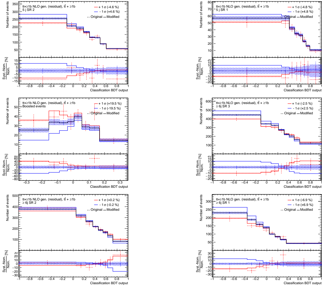
Figure 5.10.: t\bar{t} + \geq 1b templates including the \pm 1\sigma variations induced by the t\bar{t} + \geq 1b NLO generator uncertainty in the signal-enriched categories of the single lepton channel. Dashed points (solid lines) display the systematic uncertainty before (after) smoothing. The root-smoothing procedure is used in these plots. The black line represents the nominal prediction.
