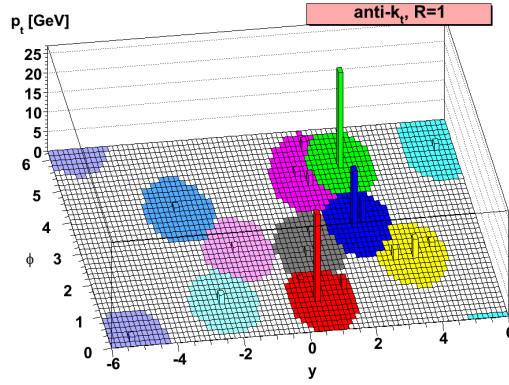
Figure 2.27.: A sample parton-level event, together with many random soft momentum particles (called ghost), clustered with the anti- k_t algorithm [122].
