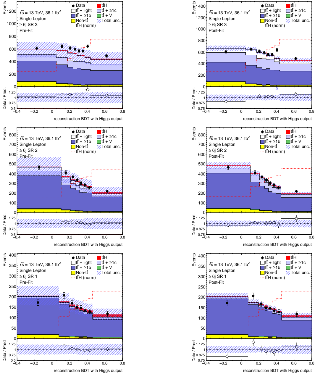
Figure 5.26.: Comparison of the predicted reconstruction BDT with Higgs output distribution to the one observed in data in the \geq 6j signal-enriched categories of the single lepton channel. (left) before applying the corrections from the fit, (right) after applying the corrections from the fit. The hashed area represent the statistical and systematic uncertainties. The pre-fit uncertainties do not include the effect of the t\bar{t} + \geq 1b and t\bar{t} + \geq 1c normalisations which are free parameters of the fit. Note that the y -axis range in the lower pad (ratio plot) is twice smaller in the right plots compared to the ones on the left.
