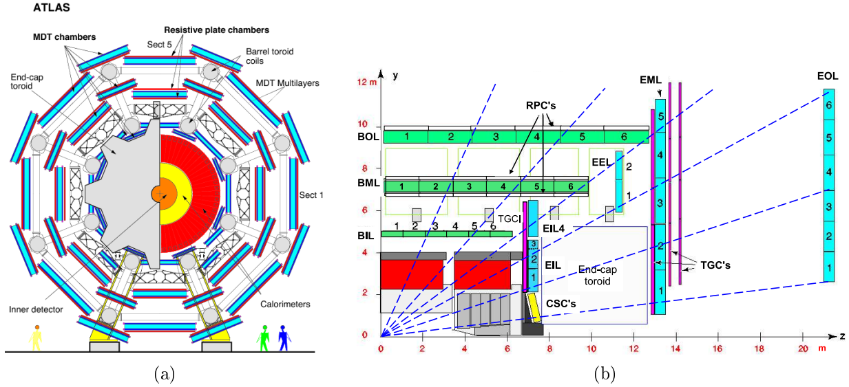
Figure 2.21.: (left) The x - y projection of the muon spectrometer [97]. (right) Cross-section of the muon system in a plane containing the beam axis (bending plane). Infinite-momentum muons would propagate along straight trajectories which are illustrated by the dashed lines and typically traverse three muon chambers [86].
