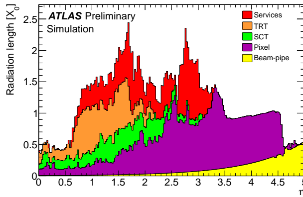
Figure 2.7.: Cumulative material thickness of the ATLAS inner detector components in terms of radiation length X_0 as a function of |\eta| and averaged over \phi [87].
