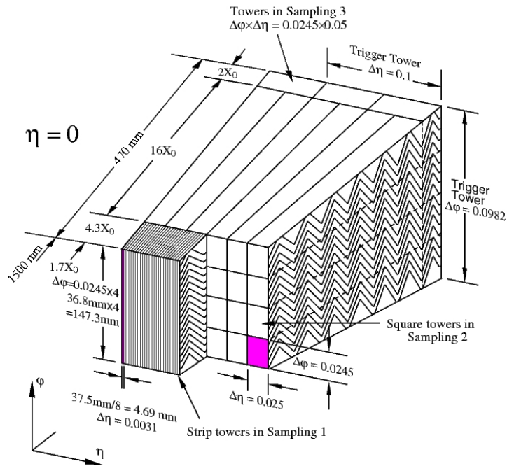
Figure 2.16.: Sketch of the barrel module divided in layers and cells [86]. The dimension of each object is also shown.
