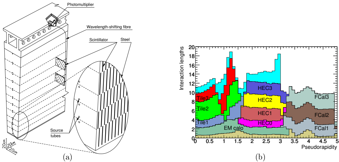
Figure 2.18.: (left) Drawing of the ATLAS hadronic calorimeter tile module. (right) Cumulative material thickness of the ATLAS calorimeter components in terms of interaction length as a function of |\eta| and averaged over \phi . Taken from [86].
