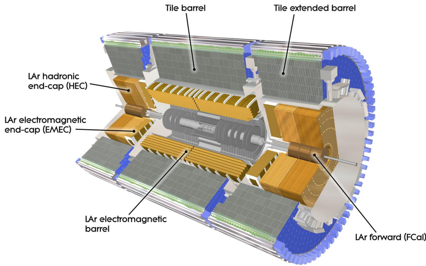
Figure 2.14.: Layout of the ATLAS calorimeters [86].
