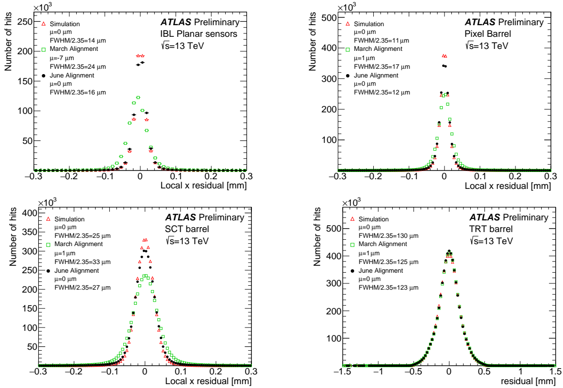
Figure 2.13.: Distance from the extrapolated track position in a given detector element to the hit recorded in the same element in the local-x-axis of the Insertable-B-Layer (top-left), pixel (top-right), SCT (bottom-left) and TRT (bottom right) detectors. The distribution obtained from simulated data with perfect alignment is compared to distribution from \sqrt{s} = 13 TeV data using the alignments performed in March and June 2015 [92].
