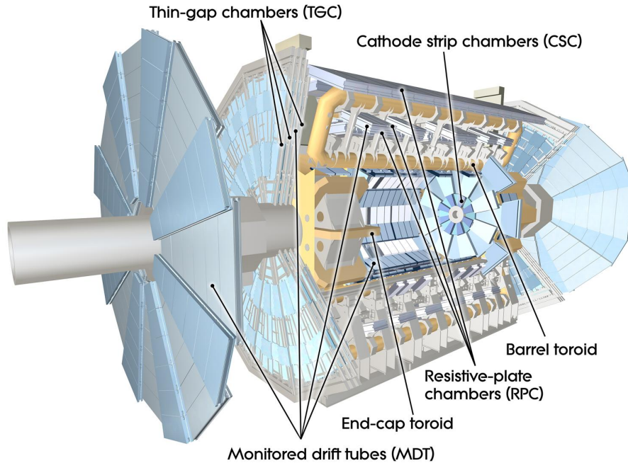
Figure 2.20.: The ATLAS muon chambers and toroidal magnets layout [86].
