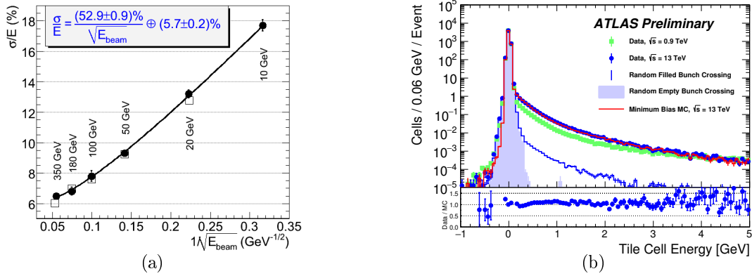
Figure 2.19.: (left) Fraction of energy for pions \sigma_E/E as a function of the beam energy. Simulated events (open squares) are compared to test beam data (full circles) [95]. (right) Distribution of the energy deposit in tile cells for \sqrt{s} = 0.9, 13 TeV data overlaid with the random filled or empty bunch crossing and the minimum bias simulation [96].
