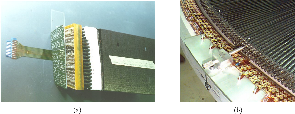
Figure 2.11.: Photography of the ATLAS TRT barrel module (left) and end-cap disk (right) showing the straw layout in these two regions [86].
