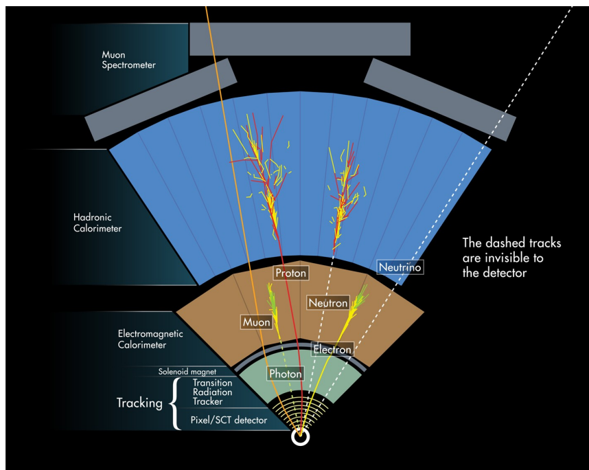
Figure 2.22.: An overview of particle identification in the ATLAS detector [88]. The solid and dashed curves show the tracks of charged and neutral particles. Arising from the interaction region (beam axis), the muon goes through the whole detector while being tracked by the Inner Detector and the Muon Spectrometer. The electron and the photon are caught by mainly the EM calorimeter and can be differentiated from the presence or absence, respectively, of a track pointing to the energy deposit in the calorimeter. The proton and the neutron are trapped by mainly the hadronic calorimeter with and without leaving a track in the ID respectively. The neutrino passes through the entire detector without leaving any signature.
