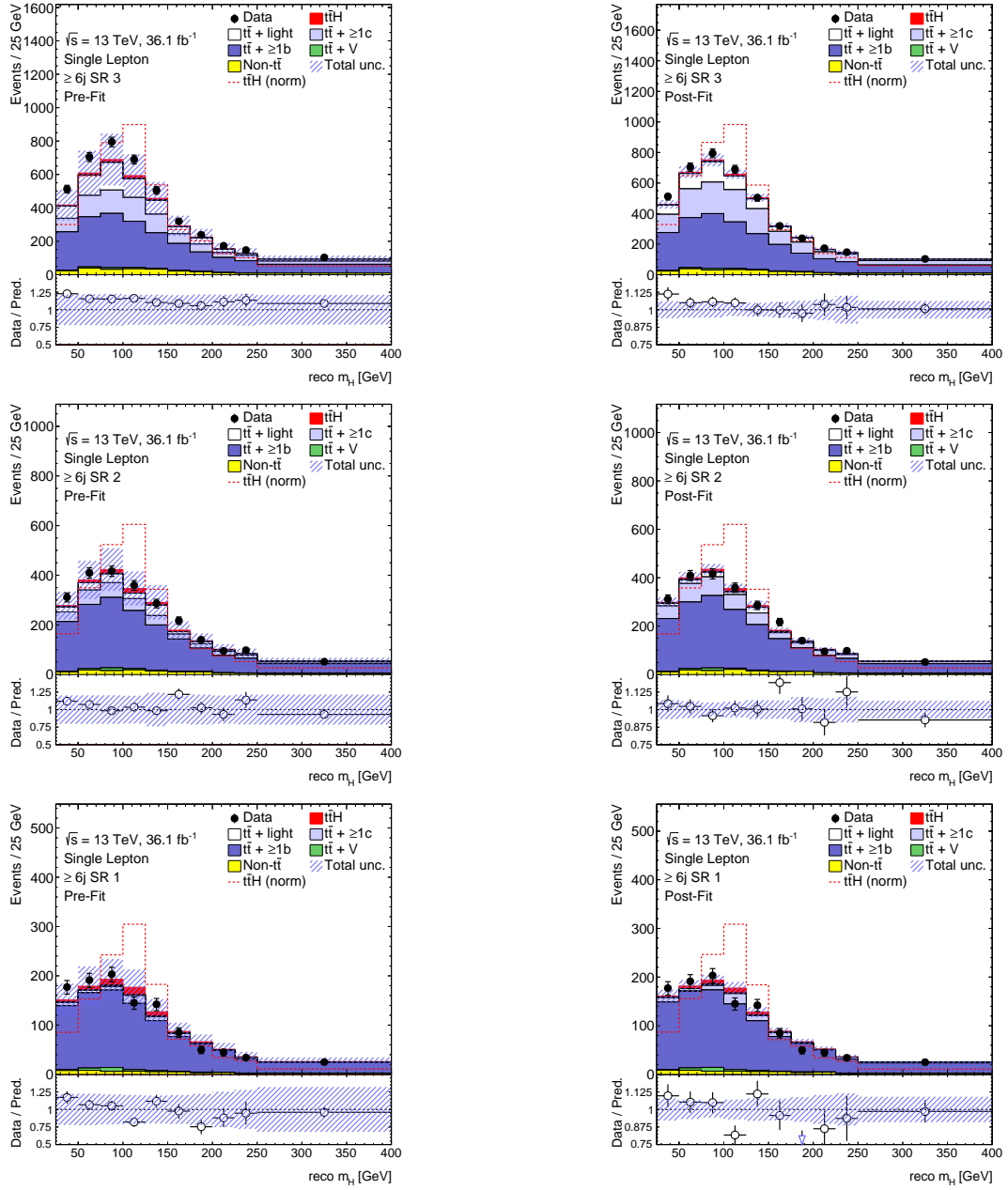
Figure 5.24.: Comparison of the predicted reconstructed Higgs boson mass distribution without to the one observed in data in the \geq 6j signal-enriched categories of the single lepton channel. (left) before applying the corrections from the fit, (right) after applying the corrections from the fit. The hashed area represent the statistical and systematic uncertainties. The pre-fit uncertainties do not include the effect of the t\bar{t} + \geq 1b and t\bar{t} + \geq 1c normalisations which are free parameters of the fit. Note that the y -axis range in the lower pad (ratio plot) is twice smaller in the right plots compared to the ones on the left.
