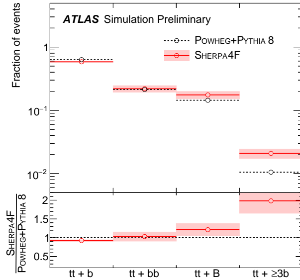
Figure 4.3.: Predicted fractions of the t\bar{t} + \geq 1b sub-components in the inclusive POWHEG+PYTHIA8 t\bar{t} sample and in the four-flavour SHERPA+OPENLOOPS NLO t\bar{t} + bb sample. The shaded area represent the SHERPA+OPENLOOPS systematic uncertainties as explained in section 5.2.2.
