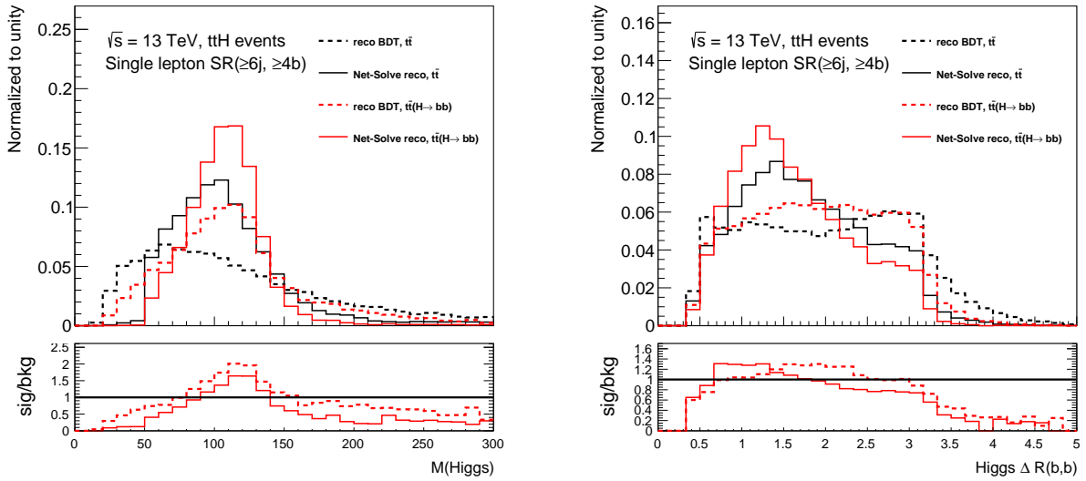
Figure 4.20.: Higgs candidate mass (left) and Higgs candidate \Delta R(b, b) (right) variables from the reconstruction BDT (dashed) or the network solving (full).
