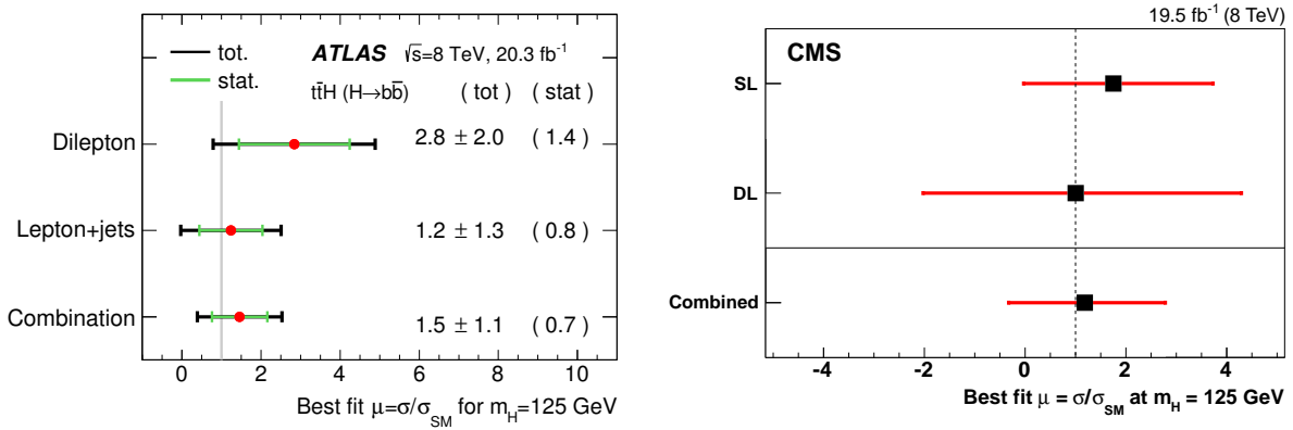
Figure 4.1.: Observed values of the t\bar{t}H(H \rightarrow b\bar{b}) signal strength \mu = \sigma/\sigma_{\text{SM}} obtained from the best fit to 20 \text{ fb}^{-1} of \sqrt{s} = 8 \text{ TeV} data within the ATLAS (left) [139] and CMS (right) [140] experiments.
