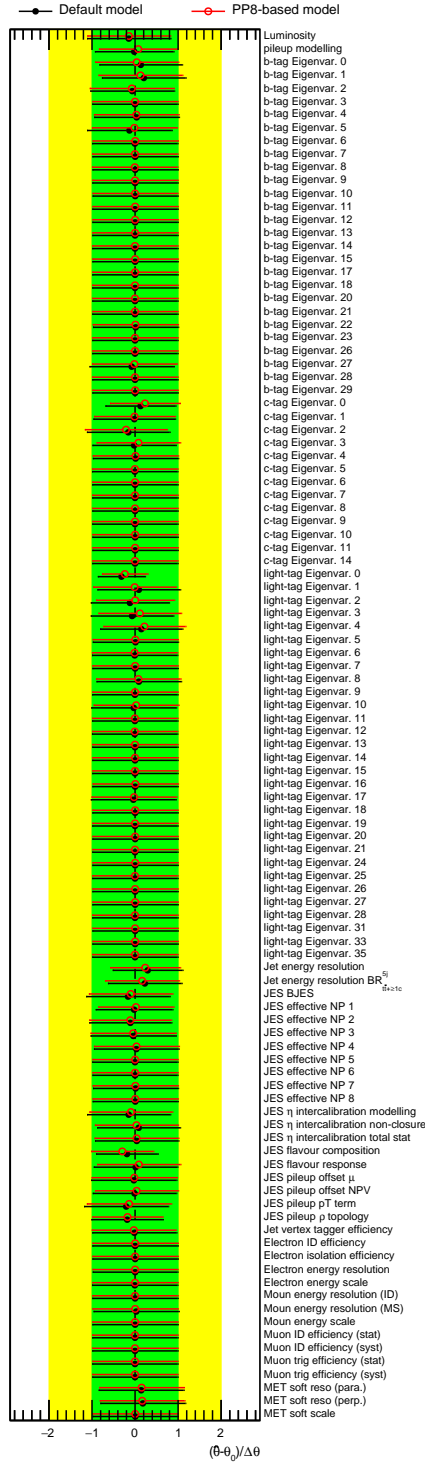
Figure 5.18.: Post-fit experimental systematic uncertainties from the fit to pseudo-data based on the POWHEG+PYTHIA6 t\bar{t} prediction. The black points display the values obtained from the default fit. The red points are obtained from the fit to data with the alternative t\bar{t} + \geq 1b model. The green (yellow) area represent the \pm 1(2)\sigma band on the pre-fit systematic uncertainty. The position of the black points and the size of their horizontal bars give the pulls and constraints in units of standard deviation, respectively.
