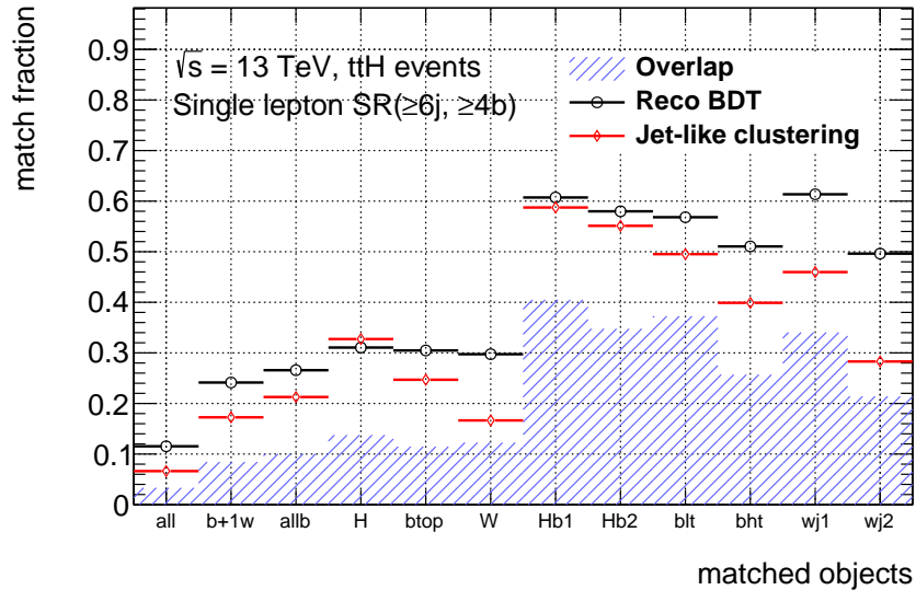
Figure 4.18.: Fraction of events with correctly assigned objects (see figure 4.17) by the reconstruction BDT without Higgs boson variables (black) and the jet-like clustering (red) algorithms. The hashed band represent the overlap between the two methods.
