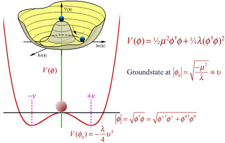
Figure 1.3.: The potential of the Higgs boson V(\phi) for a single scalar field.
