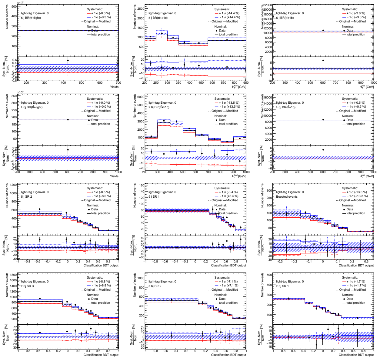
Figure 5.8.: Total prediction of all signal and background samples including the \pm 1\sigma variations induced by the l -tag e.v. 0 uncertainty in all categories compared to data. Colored points (lines) displays the systematic uncertainty before(after) smoothing. The main-smoothing is used in these plots. The black points represent data and the black solid line represent the nominal prediction. The lower pad displays the relative systematic uncertainty in percent. This relative uncertainty is compared to the relative difference between the nominal prediction and data (black points).
