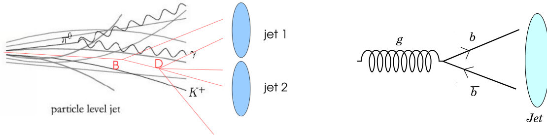
Figure 3.3.: Schematic view of a b -hadron which decay products are split in two jets (left). Schematic view of two b -hadrons merging in a single jet (right).
