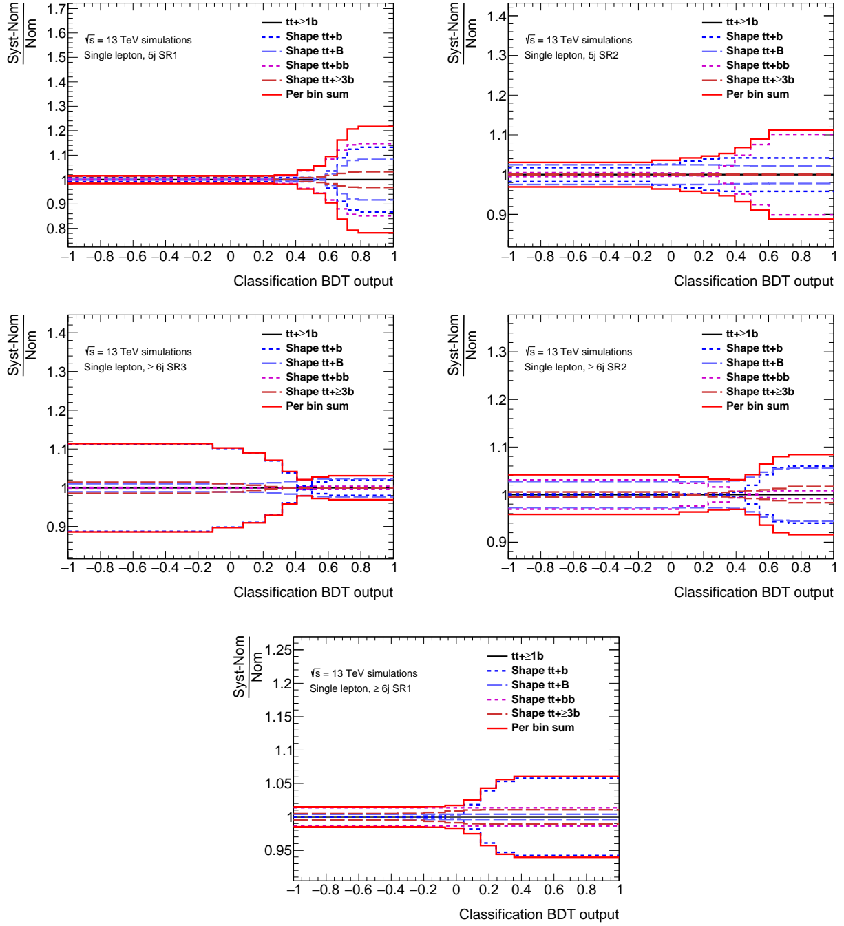
Figure .47.: Relative variations induced by the tt+\geq 1b systematic uncertainties on the tt+\geq 1b sample at \pm 1\sigma for the classification BDT distribution in the signal-enriched categories. The PP8-based tt+\geq 1b model is used. The 4FS to 5FS shape comparison uncertainties are shown. The red lines show the quadratic sum of the up and down effects systematic uncertainties in each bin.
