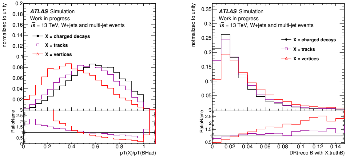
Figure 3.15.: p_T -ratio of the b -hadron evaluated using three methods (see text) over the one of the original b -hadron (left) and their \Delta R distance (right) in single- b -jets. The b -hadron momentum is evaluated using either its charged decays (black), the tracks originating from this b -hadron (magenta) or the vertices which include at least one track originating from the b -hadron (red).
