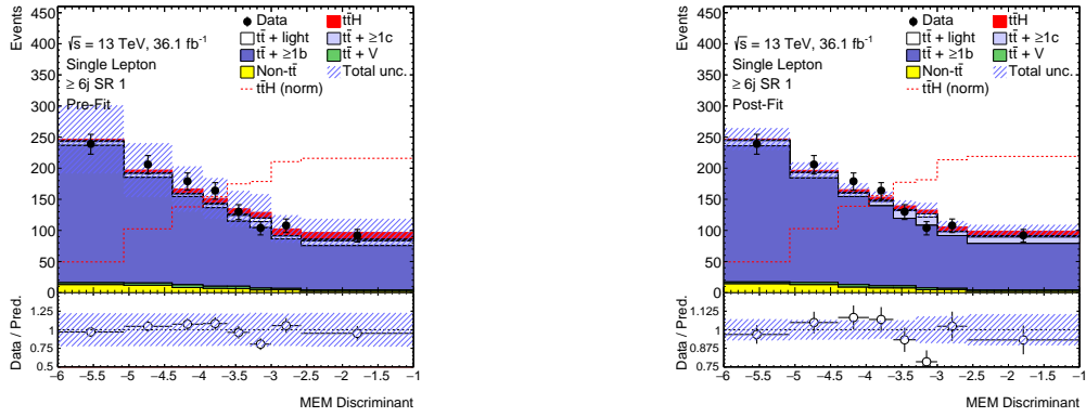
Figure 5.27.: Comparison of the predicted Matrix Element Method output distribution to the one observed in data in the \geq 6j SR1 category of the single lepton channel. (left) before applying the corrections from the fit, (right) after applying the corrections from the fit. The hashed area represent the statistical and systematic uncertainties. The pre-fit uncertainties do not include the effect of the t\bar{t} + \geq 1b and t\bar{t} + \geq 1c normalisations which are free parameters of the fit. Note that the y -axis range in the lower pad (ratio plot) is twice smaller in the right plots compared to the ones on the left.
