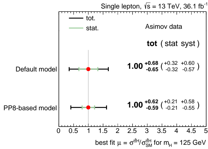
Figure 5.6.: Fitted value of the signal strength and its uncertainty from the fit with the two t\bar{t}+\geq 1b models to the Asimov data-set in the single lepton channel.
