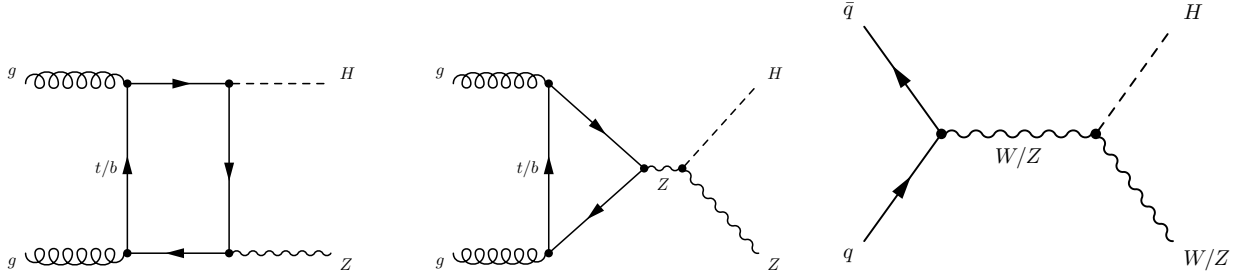
Figure 1.5.: Leading order diagrams for the production of a Higgs boson in association with a vector boson.
