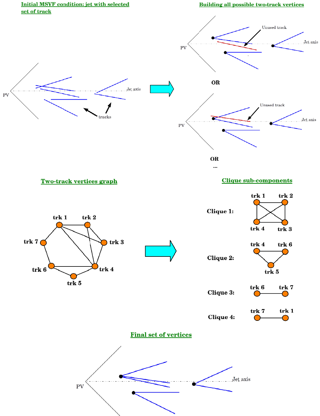
Figure 3.13.: Schematic view of the MSVF algorithm. Input tracks are selected using the same two track vertices rejection as the SSVF algorithm.
