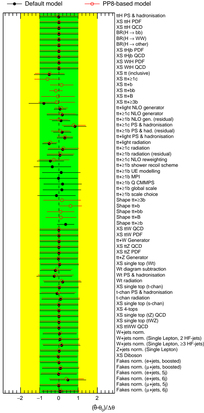
Figure 5.17.: Post-fit theoretical systematic uncertainties from the fit to pseudo-data based on the POWHEG+PYTHIA6 t\bar{t} prediction. The black points display the values obtained from the default fit. The red points are obtained from the fit to data with the alternative t\bar{t}+\geq 1b model. The green (yellow) area represent the \pm 1(2)\sigma band on the pre-fit systematic uncertainty. The position of the black points and the size of their horizontal bars give the pulls and constraints in units of standard deviation, respectively.
