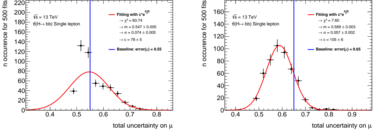
Figure 5.13.: Distribution of the signal strength uncertainties from the fits with the 500 toys of the t\bar{t} + \geq 1b NLO generator systematic (see text). (left) Toys are ran using the root-smoothing. (right) Toys are ran using the main-smoothing. The distributions are fitted with a Gaussian distribution to extract the mean signal strength uncertainty and its 1\sigma variation from the statistical uncertainty on the Sherpa sample. The blue line displays the fitted signal strength uncertainty without applying toy weights (baseline).
