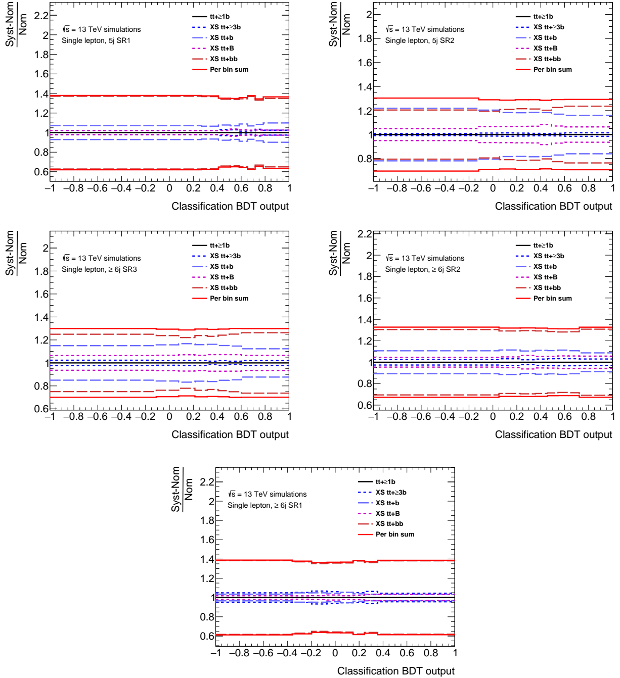
Figure .46.: Relative variations induced by the tt+\geq 1b systematic uncertainties on the tt+\geq 1b sample at \pm 1\sigma for the classification BDT distribution in the signal-enriched categories. The PP8-based tt+\geq 1b model is used. The 50% prior uncertainties on the four tt+\geq 1b sub-components are shown. The red lines show the quadratic sum of the up and down effects systematic uncertainties in each bin.
