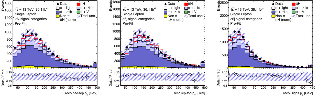
Figure 4.11.: Comparison of the predicted p_T distribution of the hadronic-top candidate (left), leptonic-top candidate (middle), and Higgs boson candidate (right) to the one observed in data for events in the signal-enriched categories. The hashed area represent the statistical and systematic uncertainties. The pre-fit uncertainties do not include the effect of the t\bar{t} + \geq 1b and t\bar{t} + \geq 1c normalisations which are free parameters of the fit.
