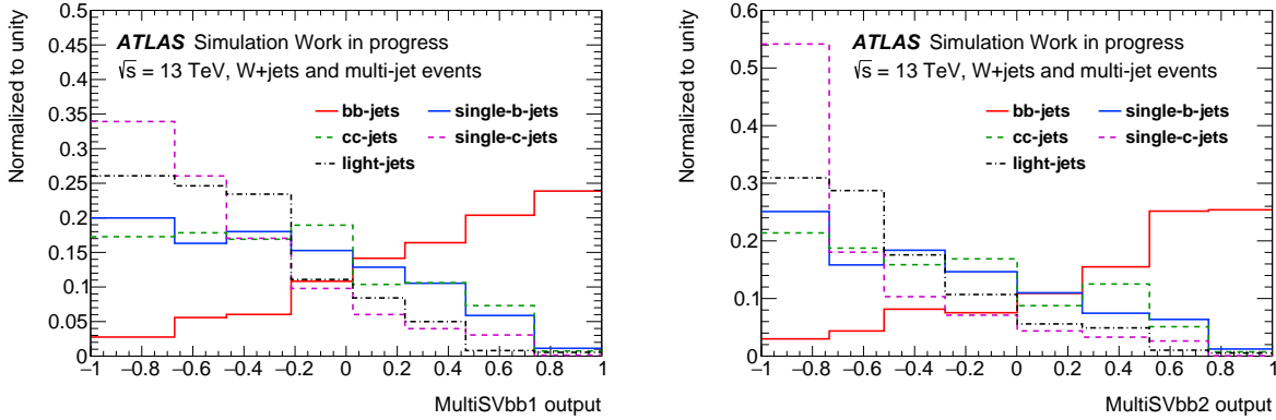
Figure 3.18.: BDT output of the MultiSVbb1 (left) and MultiSVbb2 (right) algorithms split according to the jet flavour.
