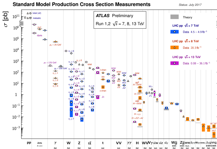
Figure 2.2.: Summary of measured cross sections for Standard Model processes confronted to expected values at \sqrt{s} = 7, 8, 13 TeV with the ATLAS detector [75].
