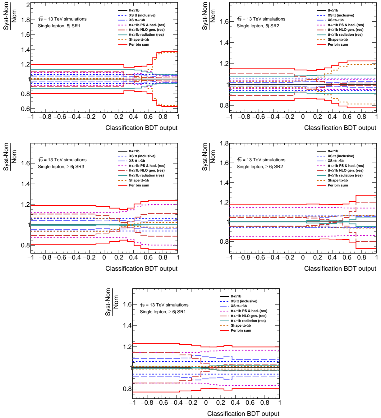
Figure .43.: Relative variations induced by the t\bar{t}+\geq 1b systematic uncertainties on the t\bar{t}+\geq 1b sample at \pm 1\sigma for the classification BDT distribution in the signal-enriched categories. The default t\bar{t}+\geq 1b model is used. The uncertainty on the t\bar{t} cross section, the 50% normalisation uncertainty of the t\bar{t}+\geq 3b sub-component and various MC to MC comparison uncertainties are shown. The red lines show the quadratic sum of the up and down effects systematic uncertainties in each bin.
