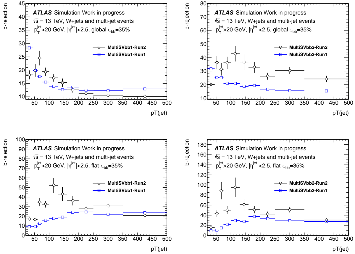
Figure 3.20.: b -jet rejection as a function of the jet p_T for a global (fixed) 35% efficiency of bb -jets for the top (bottom) row using the MultiSVbb1 (MultiSVbb2) algorithm in the left (right) column.
