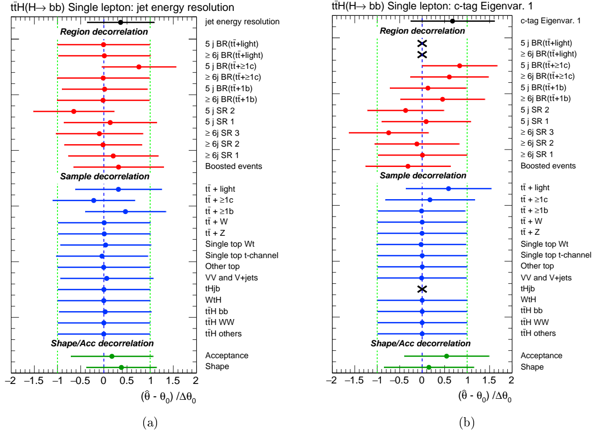
Figure 5.34.: Post-fit values on the uncorrelated components of the jet energy resolution (left) and the second eigenvector in the decomposition of the uncertainty on c -jet efficiencies (right). They are obtained from four fits using different decorrelation schemes: (black) default fit with all components correlated, (red) uncorrelated effects per categories, (blue) uncorrelated effects per process, (green) uncorrelating the normalisation and shape effects of the nuisance parameter.
