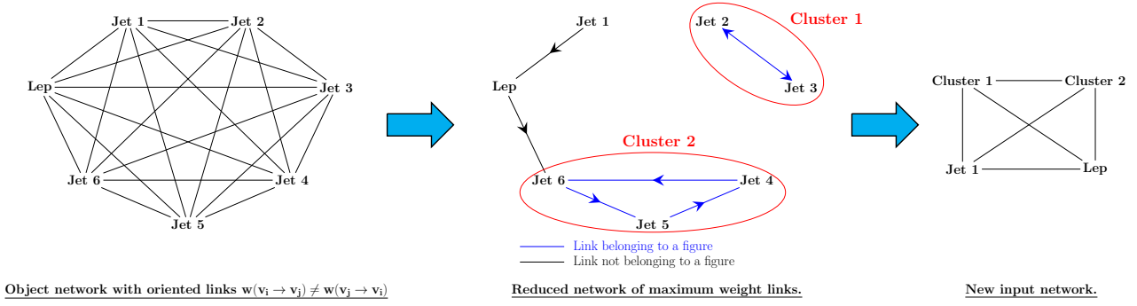
Figure 4.15.: Schematic view of the figure clustering.
