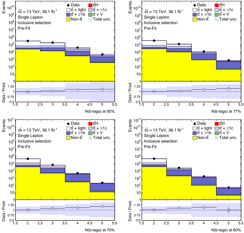
Figure 4.5.: Comparison of the predicted number of b -jets at the various working points using the PP8-based t\bar{t} sample to the one observed in data using the inclusive single lepton channel selections. The hashed area represent the statistical and systematic uncertainties.
