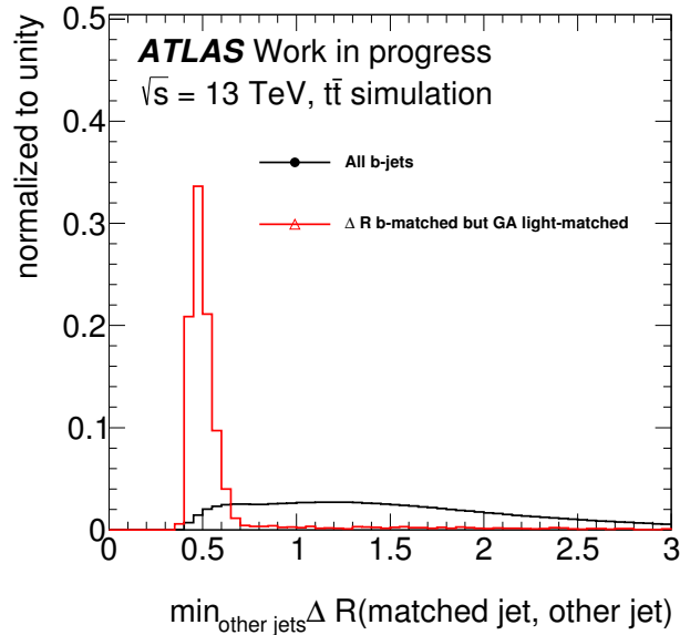
Figure 3.6.: Normalized distribution of \Delta R distance between b -truth-jets and their closest jet. The black curve shows the \Delta R distance computed for all jets matched to a b -hadron by the ghost or the exclusive \Delta R < 0.3 association. The red curve shows the \Delta R distance computed for jets labelled " b " using the \Delta R matching but labelled " light " using the ghost association.
