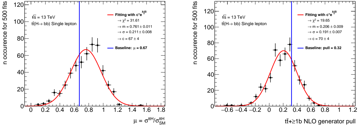
Figure 5.15.: (left) Distribution of the measured signal strength from the fits with the 500 toys of the t\bar{t} + \geq 1b NLO generator systematic (see text). (right) Distribution of the t\bar{t} + \geq 1b NLO generator uncertainty pull from the fits with the 500 toys of the t\bar{t} + \geq 1b NLO generator systematic (see text). Toys are ran using the root-smoothing. The distributions are fitted with a Gaussian distribution to extract the mean signal strength uncertainty and its 1\sigma variation from the statistical uncertainty on the Sherpa sample. The blue line displays the fitted signal strength uncertainty without applying toy weights (baseline).
