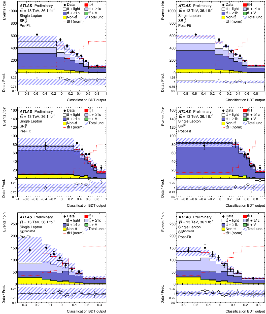
Figure 5.21.: Comparison of the predicted classification BDT distribution to the one observed in data in the 5j signal-enriched categories of the single lepton channel. (left) before applying the corrections from the fit, (right) after applying the corrections from the fit. The hashed area represent the statistical and systematic uncertainties. The pre-fit uncertainties do not include the effect of the t\bar{t} + \geq 1b and t\bar{t} + \geq 1c normalisations which are free parameters of the fit. Note that the y -axis range in the lower pad (ratio plot) is twice smaller in the right plots compared to the ones on the left.
