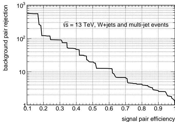
Figure .40.: Pairing BDT performance. The rejection of pair of vertices originating from different b -hadrons is shown as a function of the efficiency to select pairs of vertices originating from the same b -hadrons.
