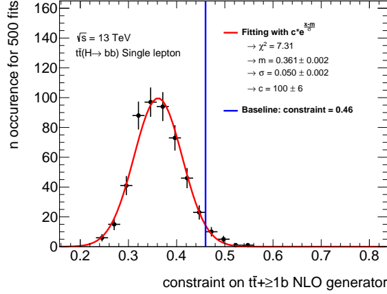
Figure 5.14.: Distribution of the post-fit uncertainty induced by t\bar{t} + \geq 1b NLO generator systematic after the fits to all toys using the root-smoothing (see text). The distribution is fitted with a Gaussian distribution to extract the mean constraint and its 1\sigma variation from the statistical uncertainty on the Sherpa sample. The blue line displays the fitted constraint without applying toy weights (baseline).
