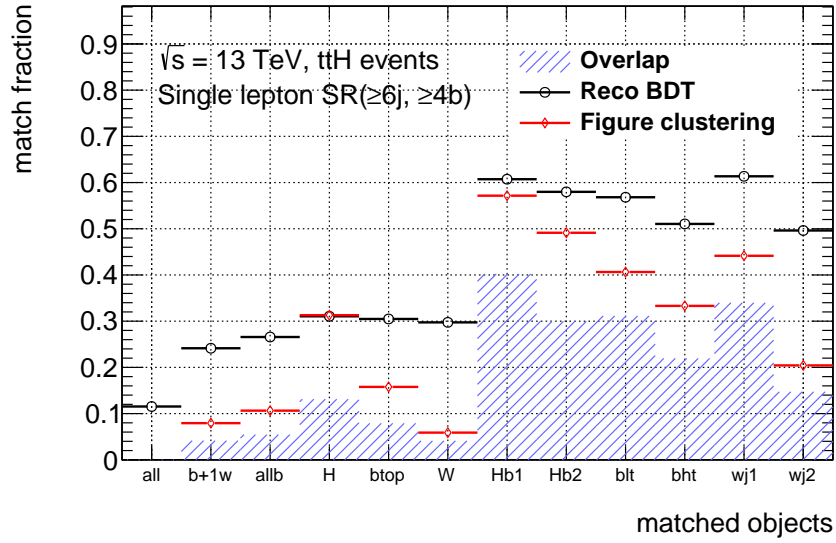
Figure 4.19.: Fraction of events with correctly assigned objects (see figure 4.17) by the reconstruction BDT without Higgs boson variables (black) and the figure based clustering (red) algorithms. The hashed band represent the overlap between the two methods.
