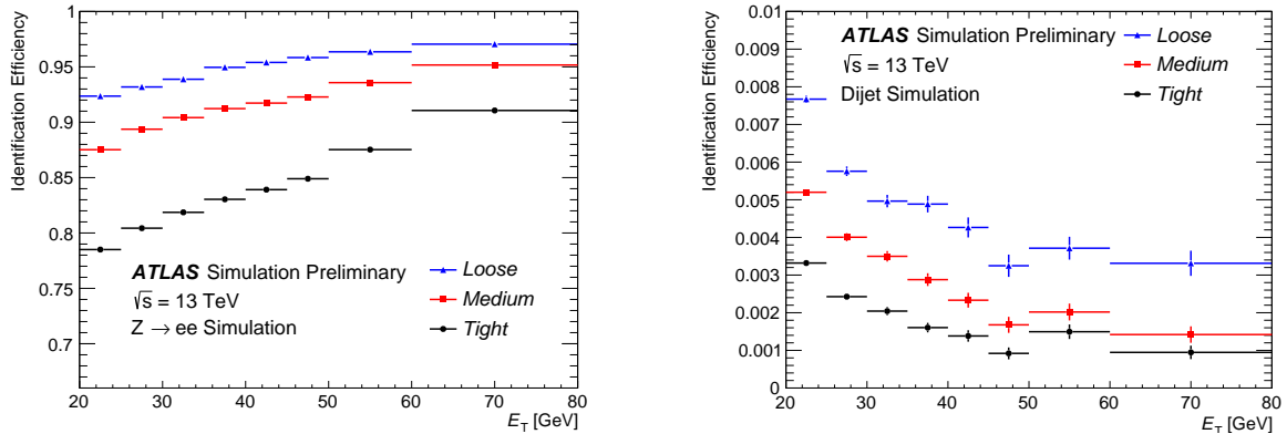
Figure 2.26.: (left) Efficiency to identify prompt electrons in Z \rightarrow ee simulated events. (right) Efficiency to identify fake electrons in multi-jet simulated events. [118].
