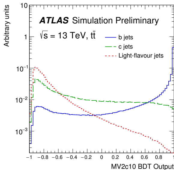
Figure 3.2.: The MV2c10 BDT output discriminant in t\bar{t} simulated events as presented in [128]. The b -jets (blue) are very well separated from the c -jets (green) and the light -jets (red).
