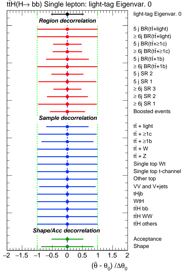
Figure 5.9.: Post-fit uncertainties on the various components of the first eigenvector in the decomposition of the uncertainty on light -jet efficiencies. They are obtained from four fits using different decorrelation schemes: (black) default fit with all components correlated, (red) uncorrelated per categories, (blue) uncorrelated per process, (green) uncorrelating the normalisation and shape components of the nuisance parameter.
