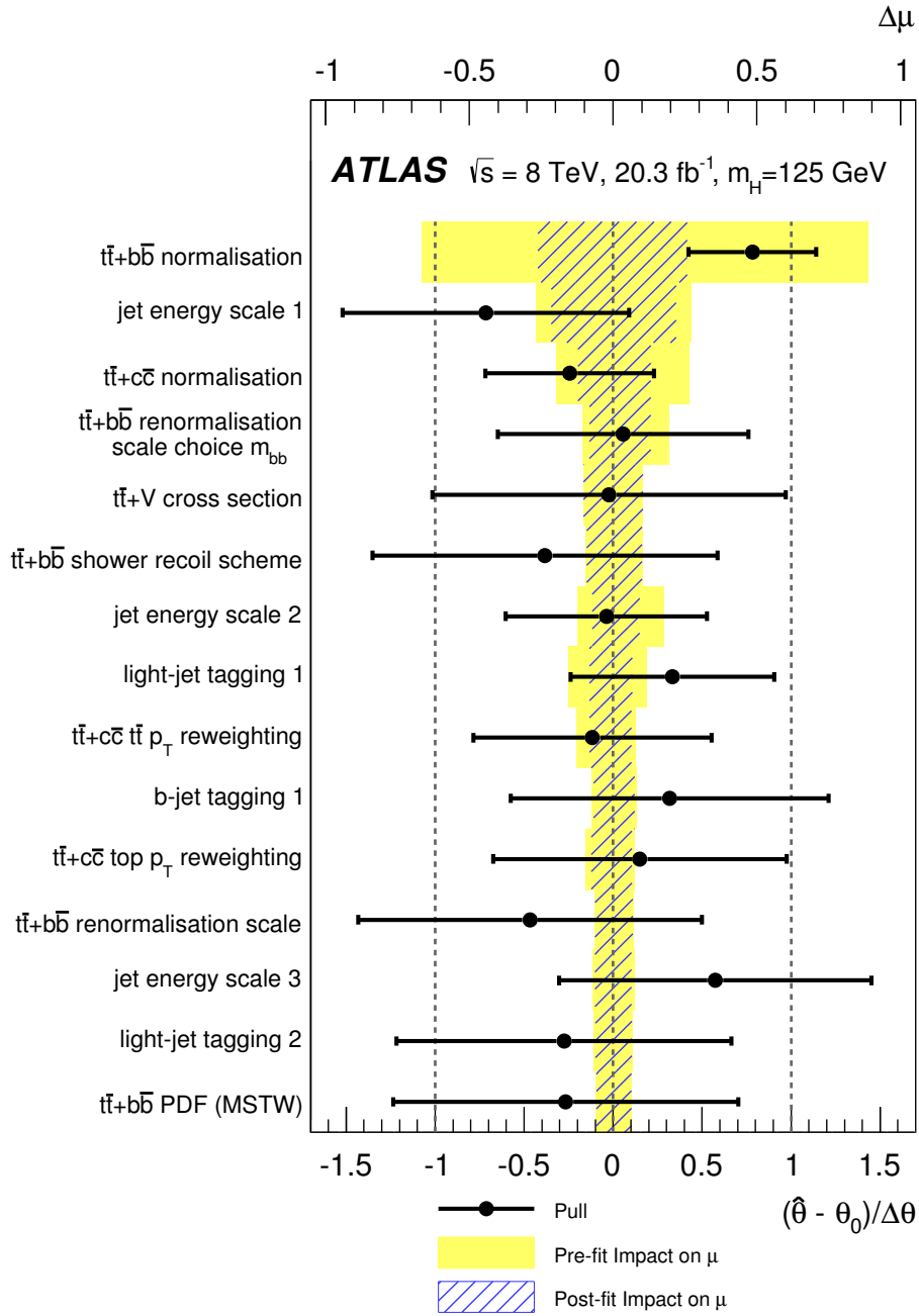
Figure 4.2.: Ranking of the nuisance parameters used in the fit according to their impact on the sensitivity of the t\bar{t}H(H \rightarrow b\bar{b}) analysis in the ATLAS experiment [139]. Only the 15 leading ones are shown. The black points are plotted according to the bottom axis and their displacement with respect to 0 shows the deviation of the measured value of the nuisance parameter in units of pre-fit 1\sigma variation. The black error bars show the post-fit uncertainty after applying the constraint from data. The blue hashed (yellow filled) areas correspond to the post(pre)-fit effect of the systematic uncertainty on the signal strength. The post(pre)-fit impact on sensitivity is computed performing the fit fixing the nuisance parameter at the post(pre)-fit \pm 1\sigma variation and taking the difference in the fitted \mu with the default fit.
