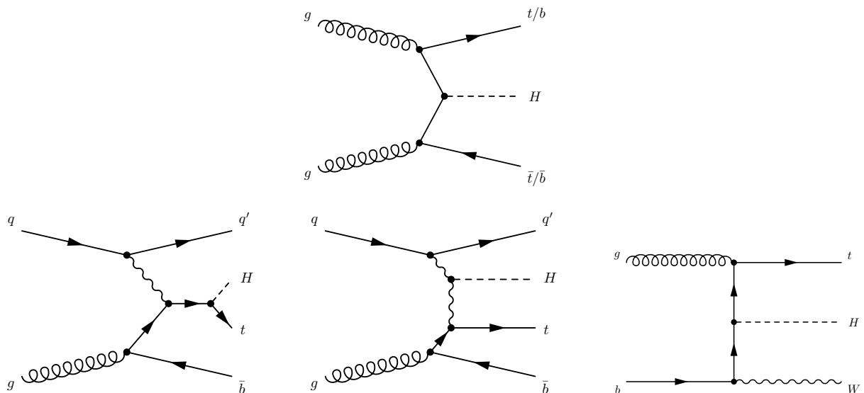
Figure 1.6.: Leading order diagrams for the production of a Higgs boson in association with top quarks.
