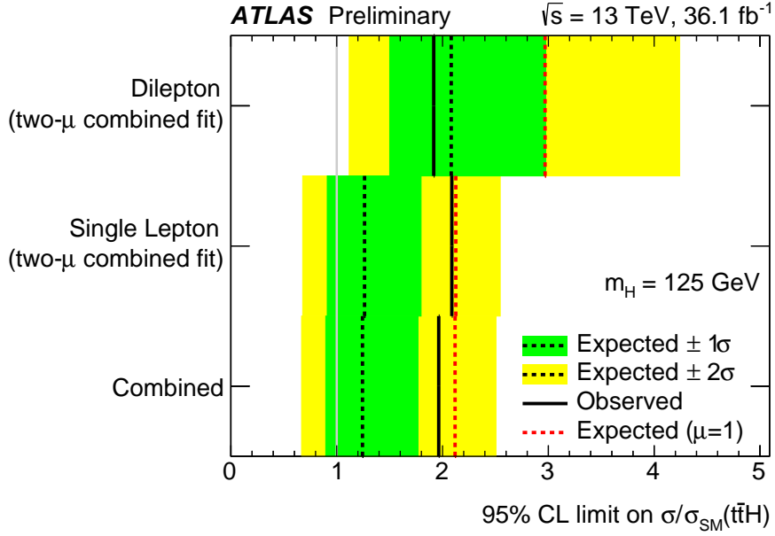
Figure 5.39.: Summary of the upper limits on the t\bar{t}H(H \rightarrow b\bar{b}) signal strength at the 95% confidence level from both individual channels and for the combination.
