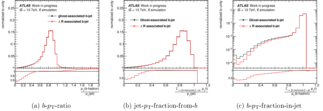
Figure 3.4.: Fragmentation of the b -hadron energy inside b -jets for the \Delta R matching and ghost association of heavy-flavoured-hadrons to jets. (a) p_T -ratio of b -hadrons to their associated jet. (b) ratio of the fraction of b -hadron p_T in the jet to the jet p_T . (c) ratio of the fraction of b -hadron p_T in the jet to the b -hadron p_T (see text for more details).
