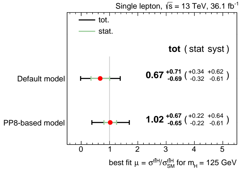
Figure 5.36.: Fitted value of the signal strength and its uncertainty from the fit of the two t\bar{t} + \geq 1b models to data in the single lepton channel.
