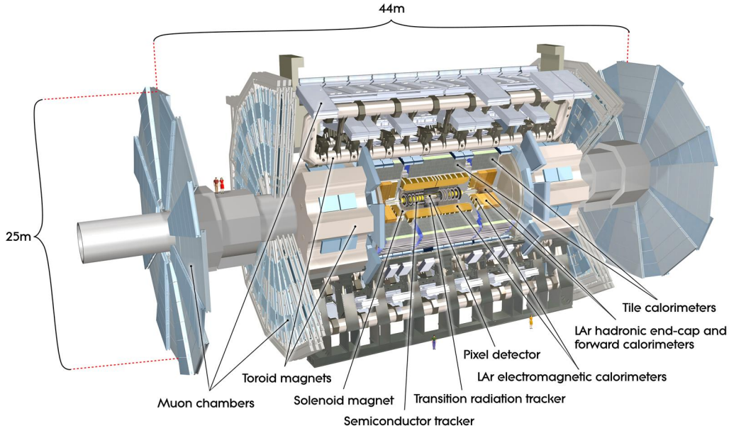
Figure 2.5.: The ATLAS detector overview [86].
