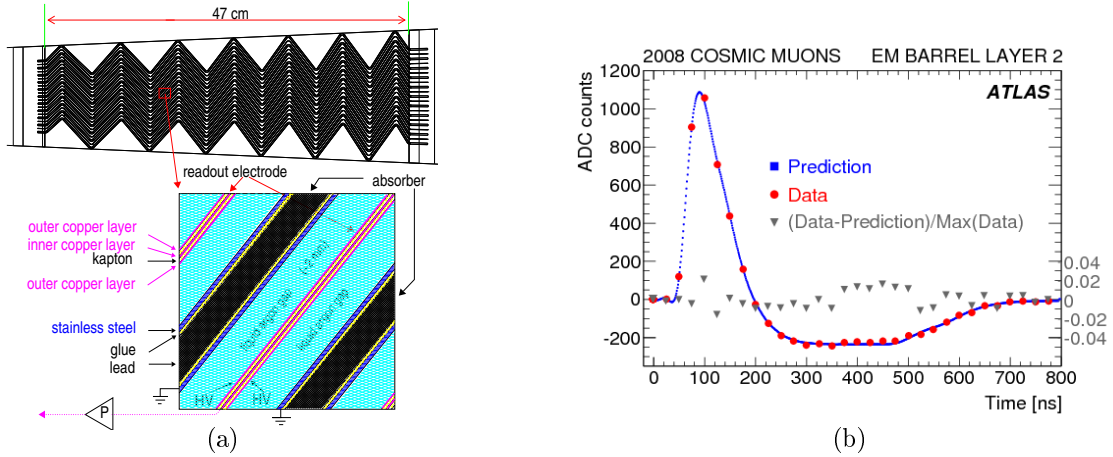
Figure 2.15.: (left) The electromagnetic calorimeter accordion geometry and the Lead Liquid-Argon technology [93]. (right) Shaped output signal of the electromagnetic calorimeter as a function of time [94].
