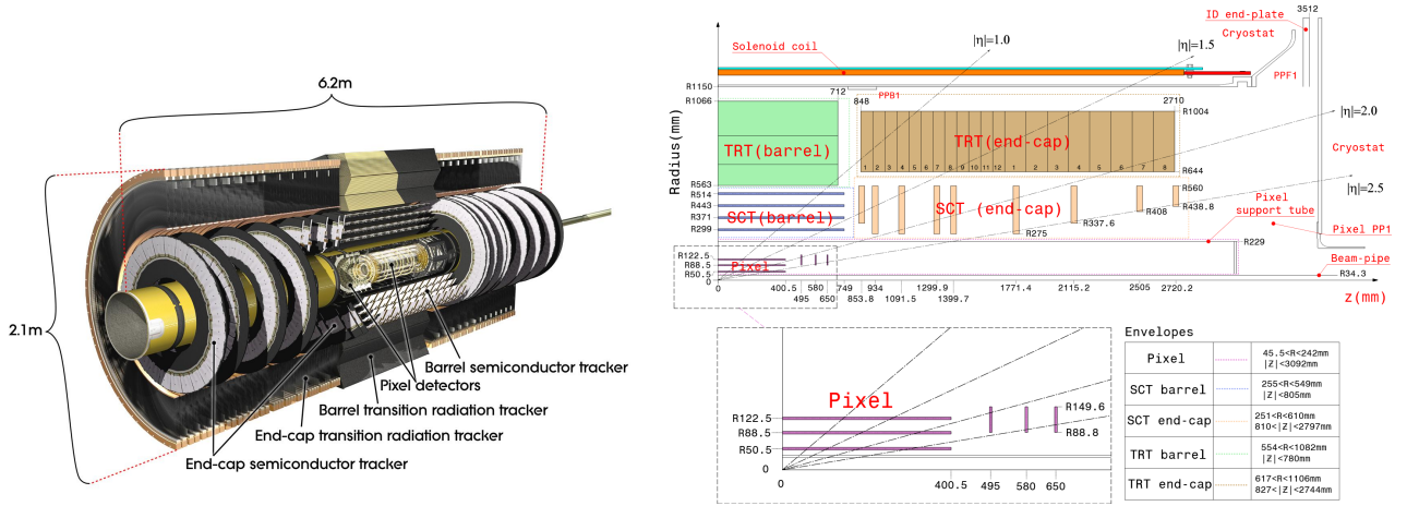
Figure 2.6.: (left) Layout of the ATLAS inner detector. (right) Quarter section of the inner detector ( r, z )-plane with the detector element positions. Taken from [86].
