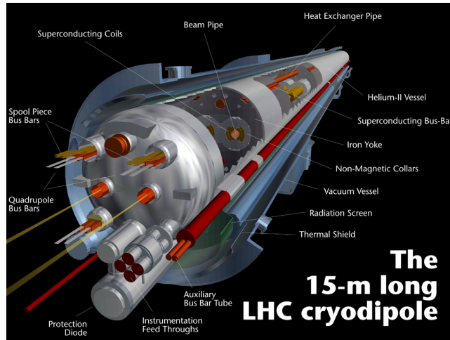
Figure 2.4.: Modelisation of the LHC dipole segment [77].
