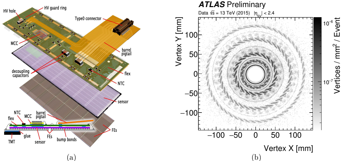
Figure 2.9.: The ATLAS pixels module layout on the left [86]. The right plot illustrates the pixel detector using reconstructed vertices corresponding to material interaction in \sqrt{s} = 13 TeV data collected with the ATLAS detector [90]. It highlights both the geometry of the pixels and the layout of the staves.
