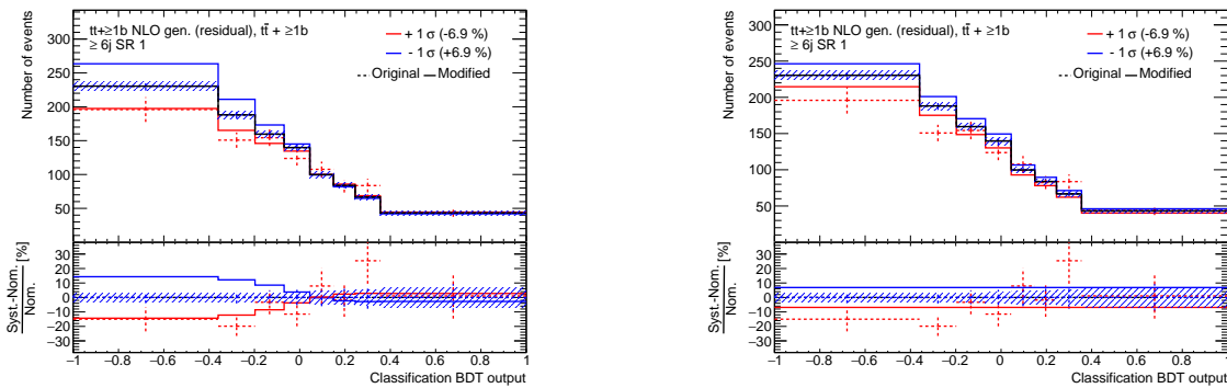
Figure 5.12.: t\bar{t} + \geq 1b templates including the \pm 1\sigma variations induced by the t\bar{t} + \geq 1b NLO generator uncertainty in the signal-enriched categories of the single lepton channel. Colored points (solid lines) display the systematic uncertainty before(after) smoothing. The root-smoothing is used in the left figure and the main-smoothing in the right one. The black line represents the nominal prediction.
