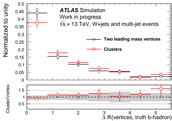
Figure .41.: \Delta R distance of the reconstructed clusters and of the two highest mass vertices to their closest b -hadron in (x, y, z) .
