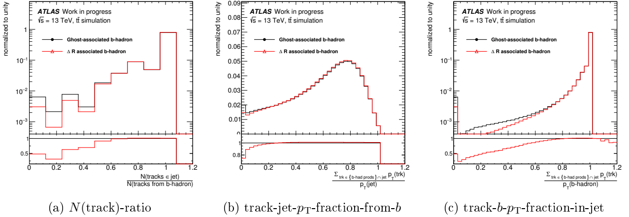
Figure 3.5.: Association of the b -hadron tracks to b -jets for the exclusive \Delta R < 0.3 matching and ghost association of heavy-flavoured-hadrons to jets. (a) number of tracks originating from the b -hadrons associated to the jet divided by the number of b -hadron tracks. (b) ratio of the fraction of b -hadron track p_T in the jet to the jet p_T . (c) ratio of the fraction of b -hadron track p_T in the jet to the b -hadron p_T (see text for more details).
