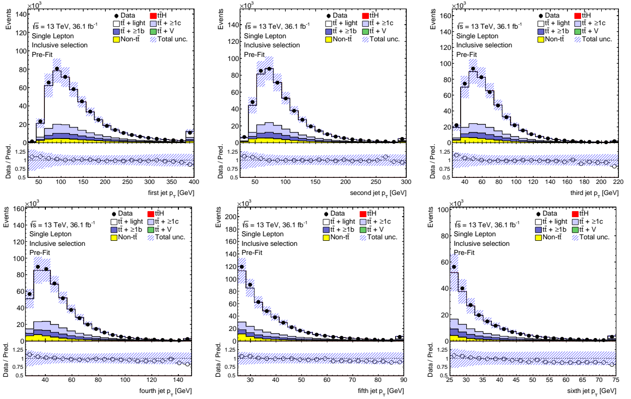
Figure 4.7.: Comparison of the predicted p_T distribution of the six leading jets to the one observed in data using the inclusive single lepton channel selections. The hashed area represent the statistical and systematic uncertainties. The pre-fit uncertainties do not include the effect of the tt + \geq 1b and tt + \geq 1c normalisations which are free parameters of the fit.
