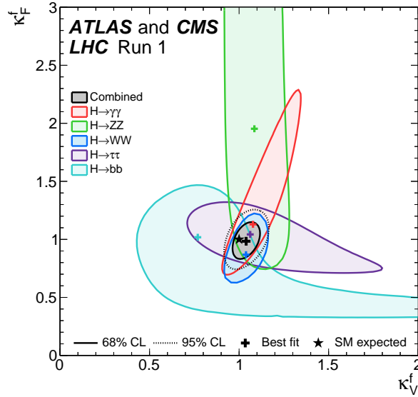
Figure 1.12.: Negative log-likelihood contours at 68% and 95% CL in the (\kappa_F^f, \kappa_V^f) plane for the combination of ATLAS and CMS and for the individual decay channels, as well as for their combination ( \kappa_F versus \kappa_V shown in black), without any assumption about the sign of the coupling modifiers [61].
