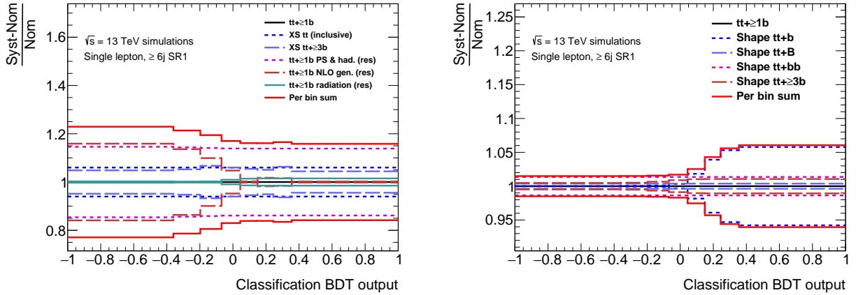
Figure 5.4.: Relative variations induced by the t\bar{t} + \geq 1b systematic uncertainties on the t\bar{t} + \geq 1b sample at \pm 1\sigma for the classification BDT distribution in the \geq 6j SR1 category. (left) common uncertainties between the two t\bar{t} + \geq 1b model: t\bar{t} cross section, 50% normalisation uncertainty of the t\bar{t} + \geq 3b sub-component and various MC to MC comparison uncertainties. (right) 4FS to 5FS shape comparison uncertainties. In both plots the red lines show the quadratic sum of the up and down effects systematic uncertainties in each bin.
