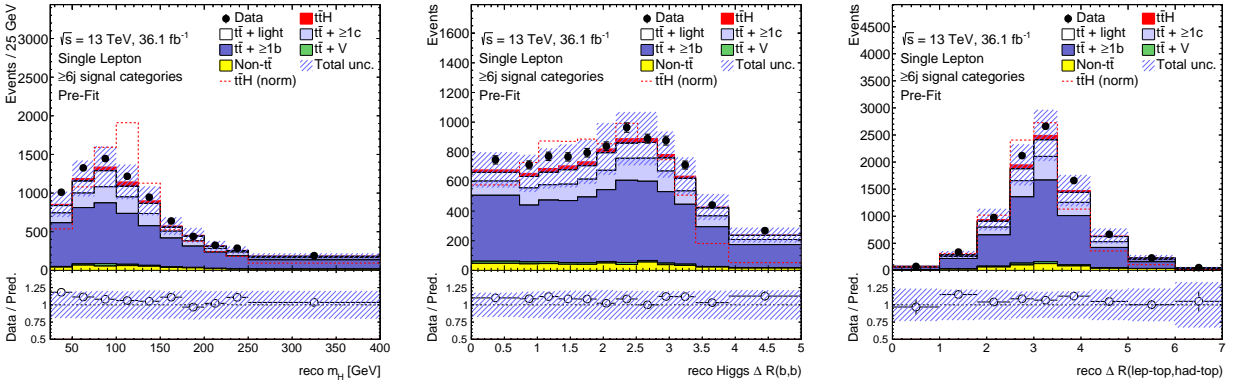
Figure 4.12.: Comparison of the predicted distributions of the Higgs candidate mass (left), of the \Delta R between the two b -jets from the Higgs candidate (middle), and the \Delta R between the hadronic-top and leptonic-top candidates (right) to the one observed in data for events in the signal-enriched categories. The hashed area represent the statistical and systematic uncertainties. The pre-fit uncertainties do not include the effect of the t\bar{t} + \geq 1b and t\bar{t} + \geq 1c normalisations which are free parameters of the fit.
