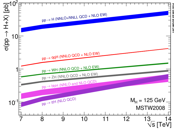
Figure 1.7.: The production cross-section of the SM Higgs boson as a function of the pp collisions center-of-mass energy for a Higgs boson of mass 125 GeV [60].
