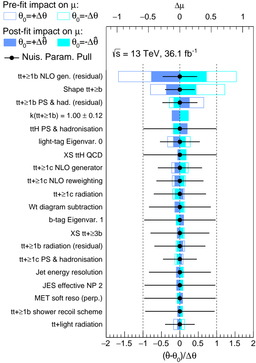
Figure 5.7.: Ranking of the nuisance parameters used in the fit according to their impact on sensitivity. Only the 20 first ones are shown. The filled (open) blue rectangles correspond to the post(pre)-fit contribution of the systematic to the uncertainty on the signal strength and is scaled with respect to the upper axis. The horizontal bar on the black points show the post-fit uncertainties after applying the constraints from the fit and scaled with respect to the bottom axis. The post(pre)-fit impact on sensitivity is computed performing the fit fixing the nuisance parameter at the post(pre)-fit \pm 1\sigma variation and taking the difference in the fitted \mu with the default fit.
