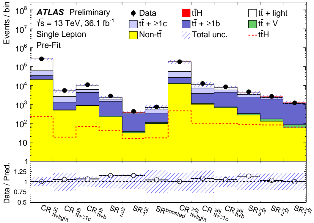
Figure 5.1.: Comparison of the predicted and observed yields in all categories of the single lepton channel before applying corrections from the fit to data. The signal contribution is shown both as a filled red area stacked on top of the backgrounds and as a separate dashed red line. The hashed band represent the statistical and systematic uncertainties. Uncertainties on the t\bar{t}+\geq 1b and t\bar{t}+\geq 1c background normalisations are not included as those are free floating parameters of the fit.
