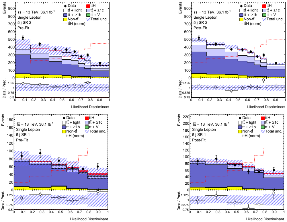
Figure 5.28.: Comparison of the predicted Likelihood Discriminant distribution to the one observed in data in the 5j signal-enriched categories of the single lepton channel. (left) before applying the corrections from the fit, (right) after applying the corrections from the fit. The hashed area represent the statistical and systematic uncertainties. The pre-fit uncertainties do not include the effect of the t\bar{t} + \geq 1b and t\bar{t} + \geq 1c normalisations which are free parameters of the fit. Note that the y -axis range in the lower pad (ratio plot) is twice smaller in the right plots compared to the ones on the left.
