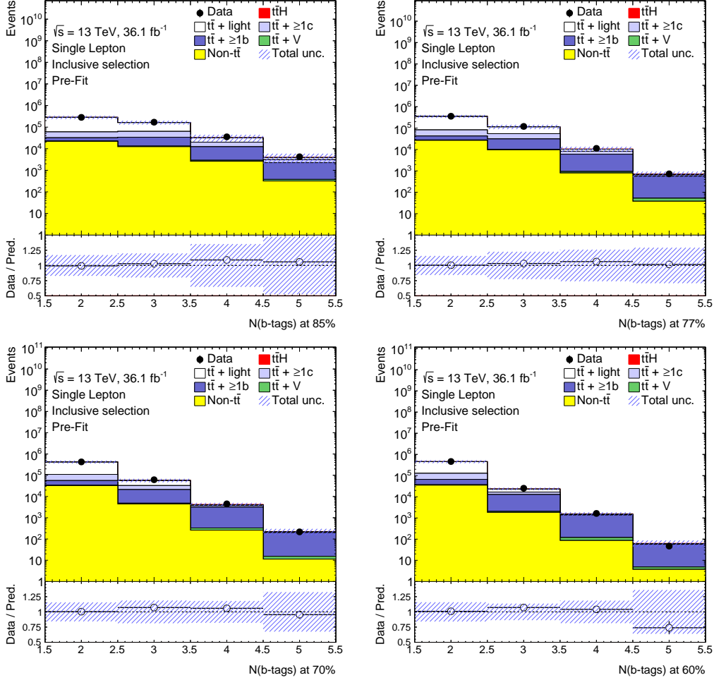
Figure 4.6.: Comparison of the predicted number of b -jets at the various working points to the one observed in data using the inclusive single lepton channel selections. The hashed area represent the statistical and systematic uncertainties. The pre-fit uncertainties do not include the effect of the t\bar{t} + \geq 1b and t\bar{t} + \geq 1c normalisations which are free parameters of the fit.
