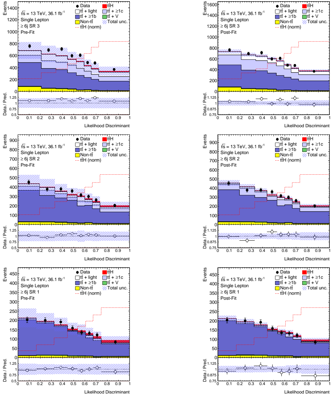
Figure 5.29.: Comparison of the predicted Likelihood Discriminant distribution to the one observed in data in the \geq 6j signal-enriched categories of the single lepton channel. (left) before applying the corrections from the fit, (right) after applying the corrections from the fit. The hashed area represent the statistical and systematic uncertainties. The pre-fit uncertainties do not include the effect of the t\bar{t} + \geq 1b and t\bar{t} + \geq 1c normalisations which are free parameters of the fit. Note that the y -axis range in the lower pad (ratio plot) is twice smaller in the right plots compared to the ones on the left.
