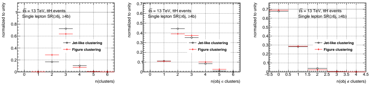
Figure 4.16.: Basic properties of the jet-like (black) and figure (red) clustering algorithm: number of reconstructed clusters per event (left), number of objects contained in clusters per event (middle), number of objects that are not clustered per event (right).
