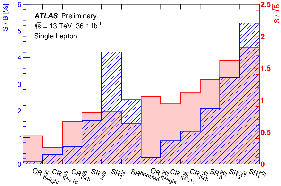
Figure 4.9.: t\bar{t}H(H \rightarrow b\bar{b}) event categories in the single lepton channel. Events are split in 11 categories based on pseudo-continuous b -tagging plus a boosted category. The blue hashed histogram displays the S/B ratio and the red histograms shows the S/\sqrt{B} ratio in all categories.
