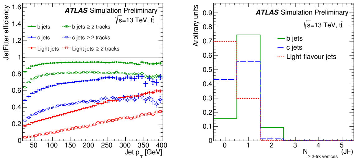
Figure 3.11.: JetFitter secondary vertex reconstruction efficiency for b -jets, c -jets, and light -jets in t\bar{t} simulated events at \sqrt{s} = 13 TeV (left). Number of two-track vertices reconstructed by the JetFitter algorithm for b -jets, c -jets, and light -jets in t\bar{t} simulated events at \sqrt{s} = 13 TeV (right) [128].
