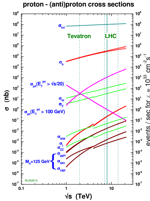
Figure 2.1.: Expected cross sections for a few typical SM processes in proton-(anti)proton collisions as a function of the center of mass energy [74].
