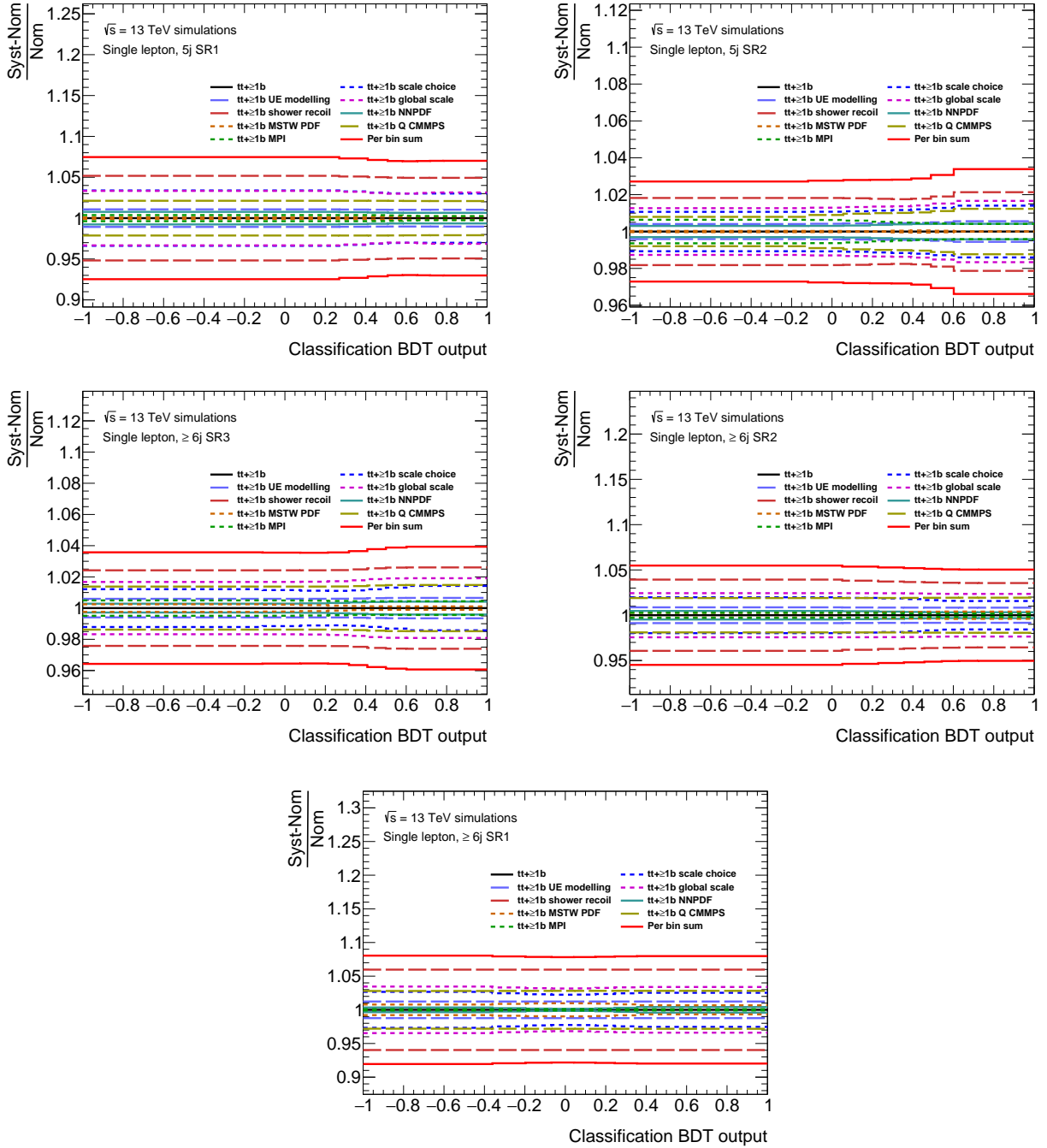
Figure .44.: Relative variations induced by the t\bar{t} + \geq 1b systematic uncertainties on the t\bar{t} + \geq 1b sample at \pm 1\sigma for the classification BDT distribution in the signal-enriched categories. The default t\bar{t} + \geq 1b model is used. Systematic uncertainties from SHERPA+OPENLOOPS variations are shown. The red lines show the quadratic sum of the up and down effects systematic uncertainties in each bin.
