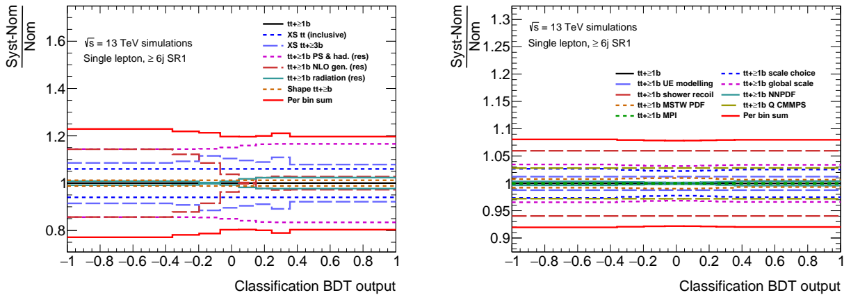
Figure 5.3.: Relative variations induced by the t\bar{t} + \geq 1b systematic uncertainties on the t\bar{t} + \geq 1b sample at \pm 1\sigma for the classification BDT distribution in the \geq 6j SR1 category. (left) common uncertainties between the two t\bar{t} + \geq 1b models: t\bar{t} cross section, 50% normalisation uncertainty of the t\bar{t} + \geq 3b sub-component and various MC to MC comparison uncertainties. (right) systematic uncertainties from SHERPA+OPENLOOPS variations. In both plots the red lines show the quadratic sum of the up and down effects systematic uncertainties in each bin.
