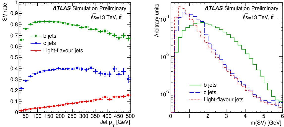
Figure 3.10.: Single secondary vertex reconstruction efficiency for b -jets, c -jets, and light -jets in t\bar{t} simulated events at \sqrt{s} = 13 TeV (left). Mass of the reconstructed single secondary vertex for b -jets, c -jets, and light -jets in t\bar{t} simulated events at \sqrt{s} = 13 TeV (right) [128].
