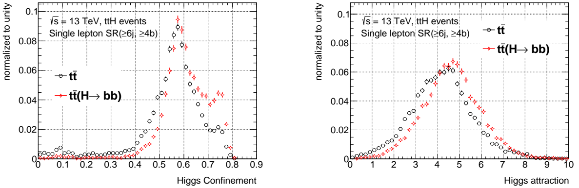
Figure 4.21.: Higgs cluster confinement (left) and Higgs cluster attraction (right) in t\bar{t}H and t\bar{t} events.
