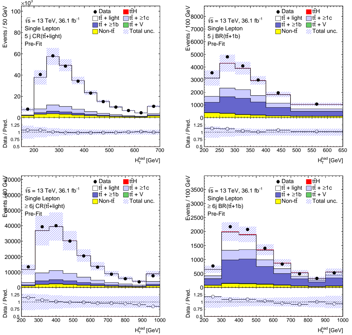
Figure 5.2.: Comparison of the predicted H_T^{\text{had}} distribution to the one observed in data for the 5-jet (up) and \geq 6 (bottom) categories enriched in the t\bar{t} + light (left) and t\bar{t} + b (right) backgrounds. The predicted distribution is shown before the corrections from the fit to data. The hashed area represent the statistical and systematic uncertainties. The uncertainties do not include the t\bar{t}+\geq 1b and t\bar{t}+\geq 1c normalisations which are free parameters of the fit.
