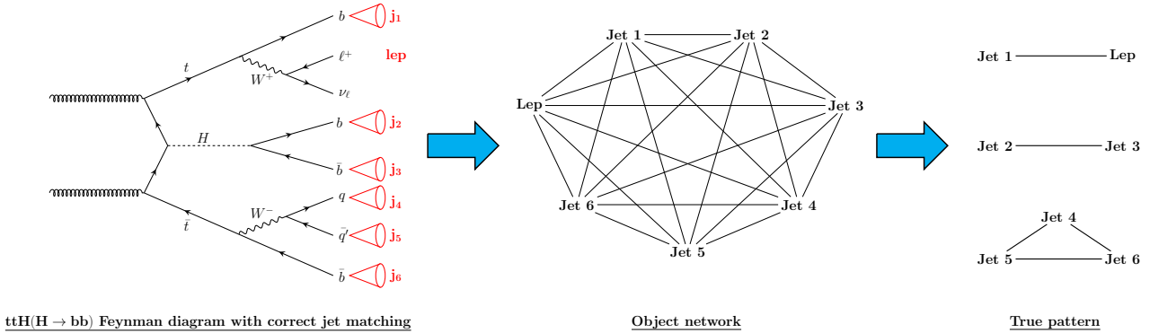
Figure 4.13.: Schematic view of the network based reconstruction. Starting from the Feynman diagram with jet associated to partons (left) a graph is formed with all objects linked together (middle). The clustering and network algorithms then seek for correct jet pattern (right).
