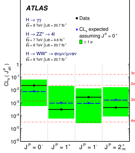
Figure 1.13.: Expected (blue triangles/dashed lines) and observed (black circles/solid lines) confidence level CL_s for alternative spin-parity hypotheses assuming a J^P = 0^+ signal. The green band represents the 68% CL_s(J^P_{\text{alt}}) expected exclusion range for the same signal assumption. On the right y-axis, the corresponding numbers of Gaussian standard deviations are given, using the one-sided convention [65].
