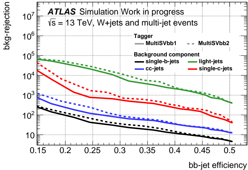
Figure 3.19.: Expected MultiSVbb1 and MultiSVbb2 bb -jet efficiency versus the various background rejections in a mixture of di-jet and W +jets events in \sqrt{s} = 13 TeV simulations.
