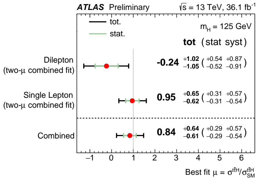
Figure 5.38.: Fitted value of the signal strength and its uncertainty from the fit of the default t\bar{t} + \geq 1b models to data in the single lepton, di-lepton channels and for the combined fit.
