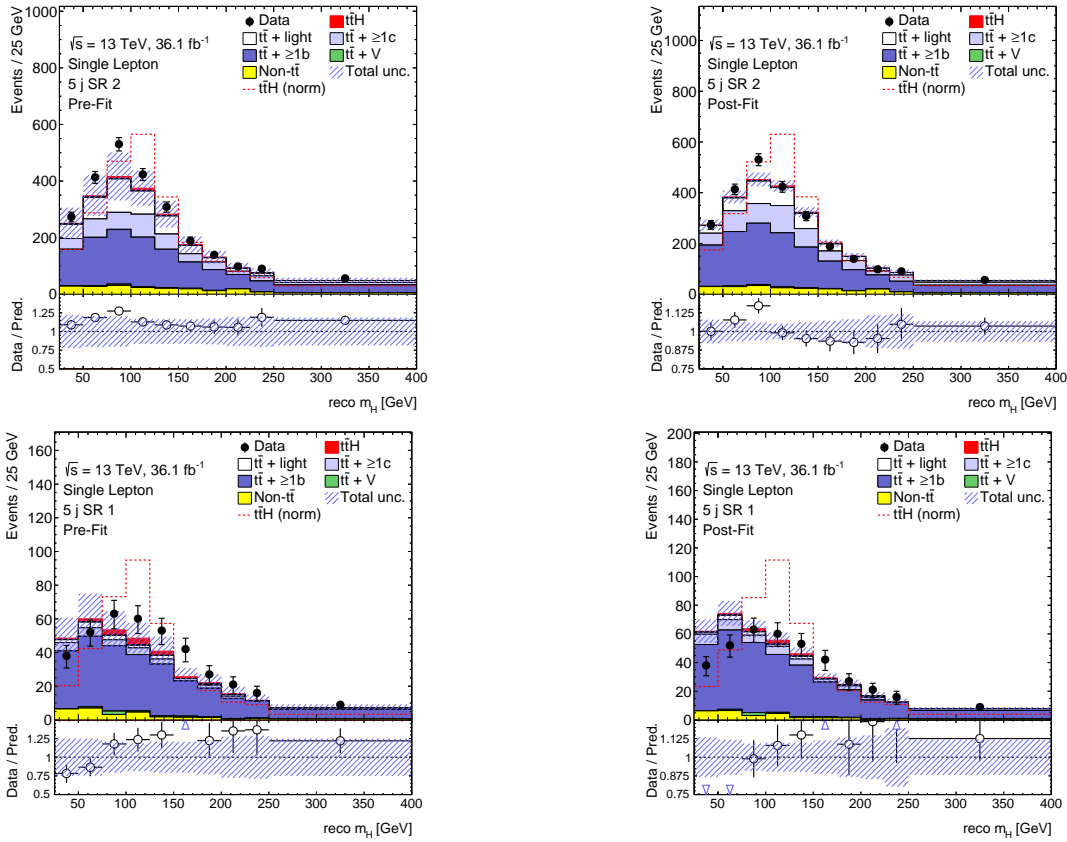
Figure 5.23.: Comparison of the predicted reconstructed Higgs boson mass distribution to the one observed in data in the 5j signal-enriched categories of the single lepton channel. (left) before applying the corrections from the fit, (right) after applying the corrections from the fit. The hashed area represent the statistical and systematic uncertainties. The pre-fit uncertainties do not include the effect of the t\bar{t} + \geq 1b and t\bar{t} + \geq 1c normalisations which are free parameters of the fit. Note that the y -axis range in the lower pad (ratio plot) is twice smaller in the right plots compared to the ones on the left.
