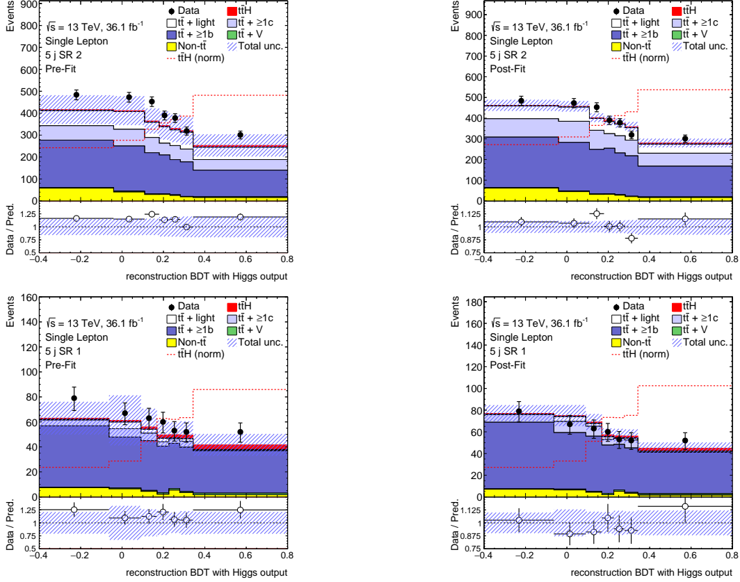
Figure 5.25.: Comparison of the predicted reconstruction BDT with Higgs output distribution to the one observed in data in the 5j signal-enriched categories of the single lepton channel. (left) before applying the corrections from the fit, (right) after applying the corrections from the fit. The hashed area represent the statistical and systematic uncertainties. The pre-fit uncertainties do not include the effect of the t\bar{t} + \geq 1b and t\bar{t} + \geq 1c normalisations which are free parameters of the fit. Note that the y -axis range in the lower pad (ratio plot) is twice smaller in the right plots compared to the ones on the left.
