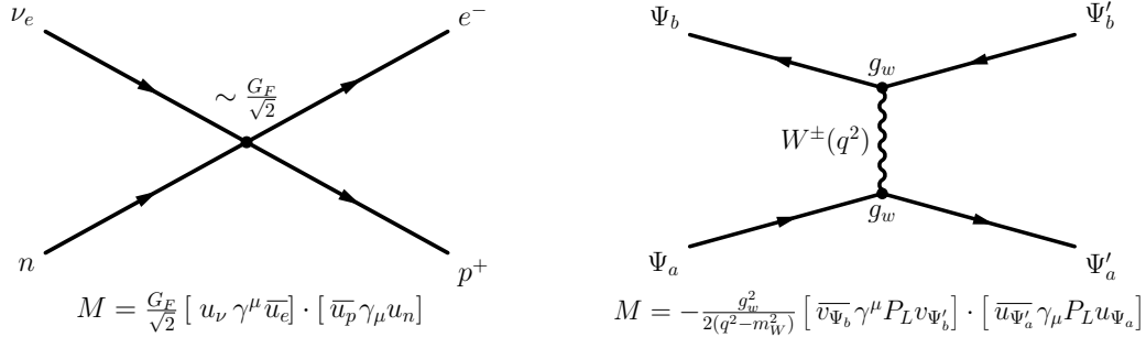
Figure 1.2.: Feynman diagrams for Fermi's 4-point interaction (a) and a weakly interacting process (b). The matrix element is modified to include a massive propagator containing the weak coupling constant g_w and the left-handed projections to account for the parity violation.
