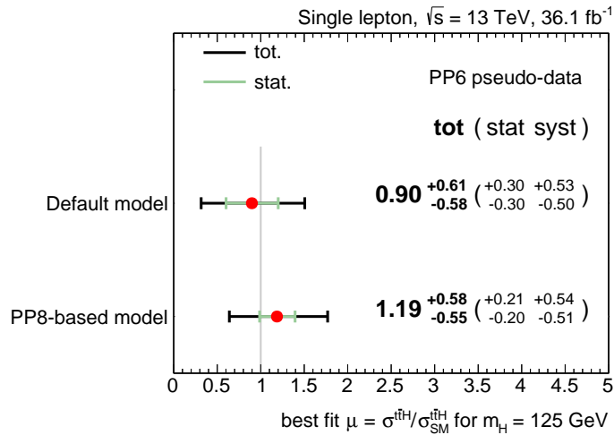
Figure 5.16.: Fitted value of the signal strength and its uncertainty from the fit with the two t\bar{t} + \geq 1b models to pseudo-data in the single lepton channel.
