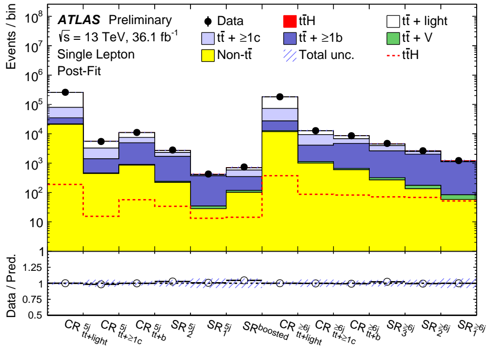
Figure 5.19.: Comparison of the predicted and observed yields in all categories of the single lepton channel after applying corrections from the fit to data. The signal contribution is shown both as a filled red area stacked on top of the backgrounds and as a separate dashed red line. The hashed band represent the statistical and systematic uncertainties. Uncertainties on the t\bar{t} + \geq 1b and t\bar{t} + \geq 1c background normalisations are not included as those are free floating parameters of the fit.
