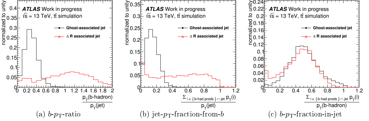
Figure 3.7.: Fragmentation of the b -hadron energy inside b -jets for the \Delta R -associated-truth-jet and the ghost-associated-truth-jet in case of close-by-jets. In this case the same b -hadron is associated to two jets depending on the association scheme. (a) p_T -ratio of b -hadrons to their associated jet. (b) ratio of the b -hadron p_T in the jet to the jet p_T . (c) ratio of the fraction of b -hadron p_T in the jet to the b -hadron p_T .
