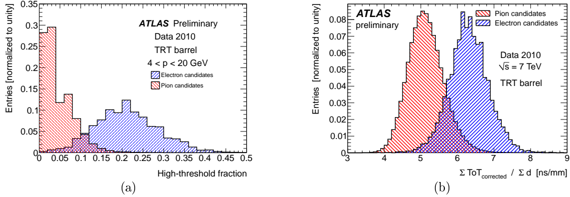
Figure 2.12.: Particle identification based on the TRT as a standalone detector. The left plot shows the electron identification based on the energy of the straw signal output. The right plot shows the discrimination of pions and electrons using the time-over-threshold on the TRT response divided by the transverse track path length inside the straw. Taken from [91]
