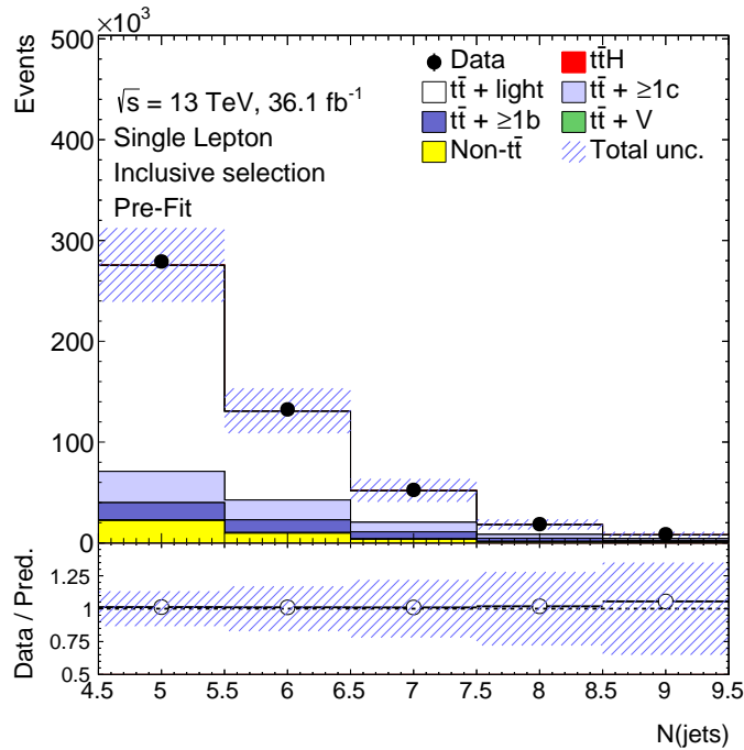
Figure 4.4.: Comparison of the predicted number of jets to the one observed in data using the inclusive single lepton channel selections. The hashed area represent the statistical and systematic uncertainties. The pre-fit uncertainties do not include the effect of the tt + \geq 1b and tt + \geq 1c normalisations which are free parameters of the fit.
