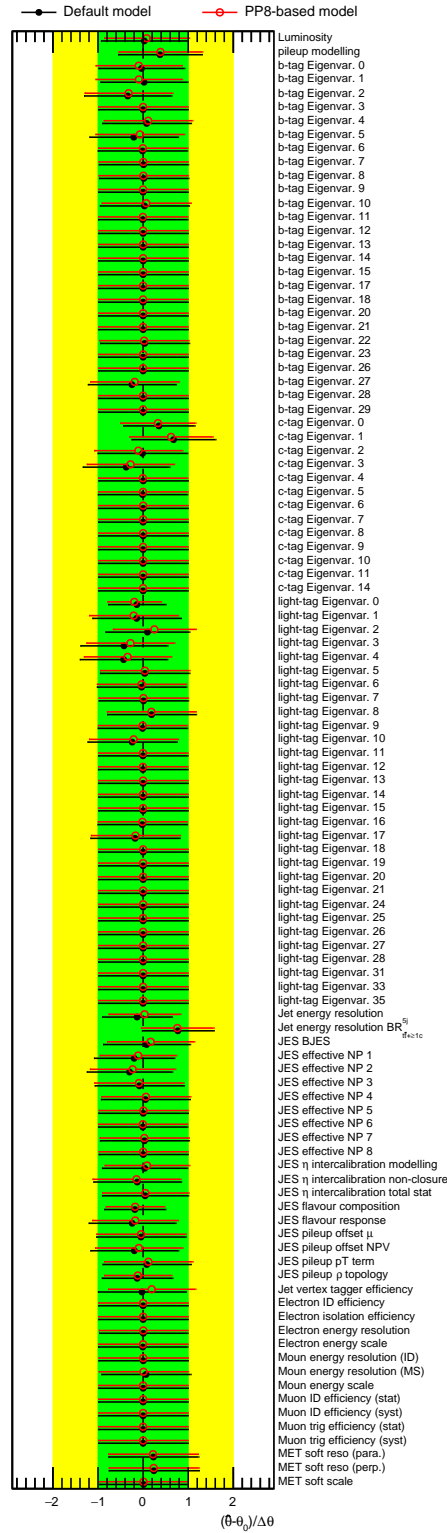
Figure 5.31.: Post-fit experimental systematic uncertainties from the fit to data. The black points display the values obtained from the default fit. The red points are obtained from the fit to data with the alternative t\bar{t} + \geq 1b model. The green (yellow) area represent the \pm 1(2)\sigma band on the pre-fit systematic uncertainty. The position of the black points and the size of their horizontal bars give the pulls and constraints in units of standard deviation, respectively.
