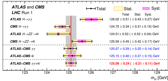
Figure 1.11.: Summary of Higgs boson mass measurements from the individual analyses of ATLAS and CMS and from the combined analysis for data collected in the Run 1 of the LHC. The systematic (narrower, magenta-shaded bands), statistical (wider, yellow-shaded bands), and total (black error bars) uncertainties are indicated. The (red) vertical line and corresponding (gray) shaded column indicate the central value and the total uncertainty of the combined measurement, respectively [61].
