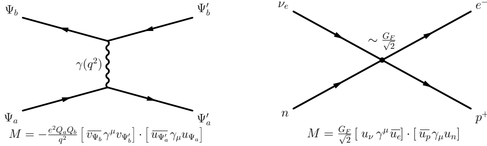
Figure 1.1.: Feynman diagrams for a QED scattering process (left) and Fermi's 4-point interaction (right). The matrix element of the weak interaction is directly extrapolated from QED Feynman rules, replacing the electromagnetic coupling by the Fermi constant G_F .
