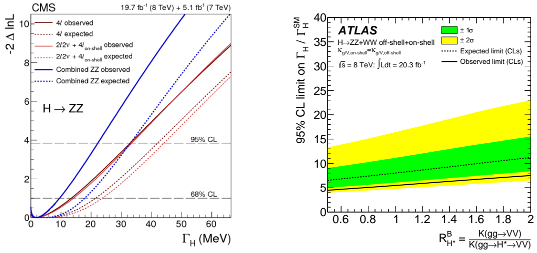
Figure 1.14.: (left) Scan of the negative log-likelihood as a function of \Gamma_H in the different analysis channels (red and black) and for the combined fit (blue) in the CMS analysis [70]. (right) Observed and expected combined 95% CL upper limit on \Gamma_H / \Gamma_H^{\text{SM}} as a function of coupling ratio [71] in the ATLAS analysis. The upper limits are calculated from the CL_s method, with the SM values as the alternative hypothesis. The green (yellow) bands represent the 68% (95%) confidence intervals for the CL_s expected limit.
