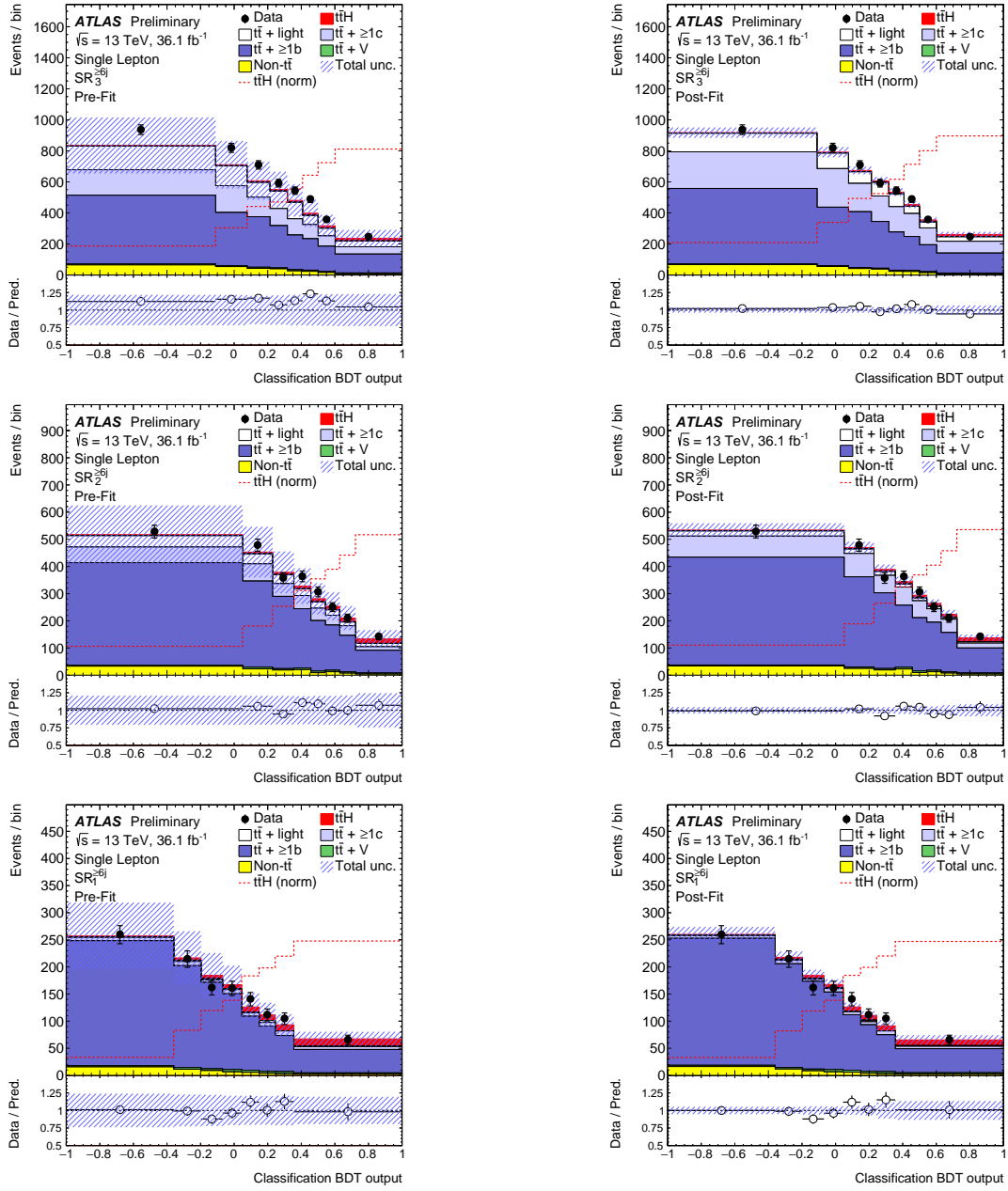
Figure 5.22.: Comparison of the predicted classification BDT distribution to the one observed in data in the \geq 6j signal-enriched categories of the single lepton channel. (left) before applying the corrections from the fit, (right) after applying the corrections from the fit. The hashed area represent the statistical and systematic uncertainties. The pre-fit uncertainties do not include the effect of the t\bar{t}+\geq 1b and t\bar{t}+\geq 1c normalisations which are free parameters of the fit. Note that the y -axis range in the lower pad (ratio plot) is twice smaller in the right plots compared to the ones on the left.
