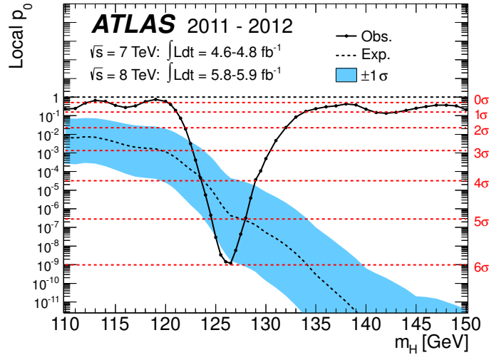
Figure 1.10.: The observed (solid) local p_0 as a function of the Higgs boson mass ( m_H ) in the low mass range. The dashed curve shows the expected local p_0 under the hypothesis of a SM Higgs boson signal with its \pm 1\sigma band. The horizontal dashed lines indicate the p-values corresponding to significances of 1 to 6 \sigma [4].
