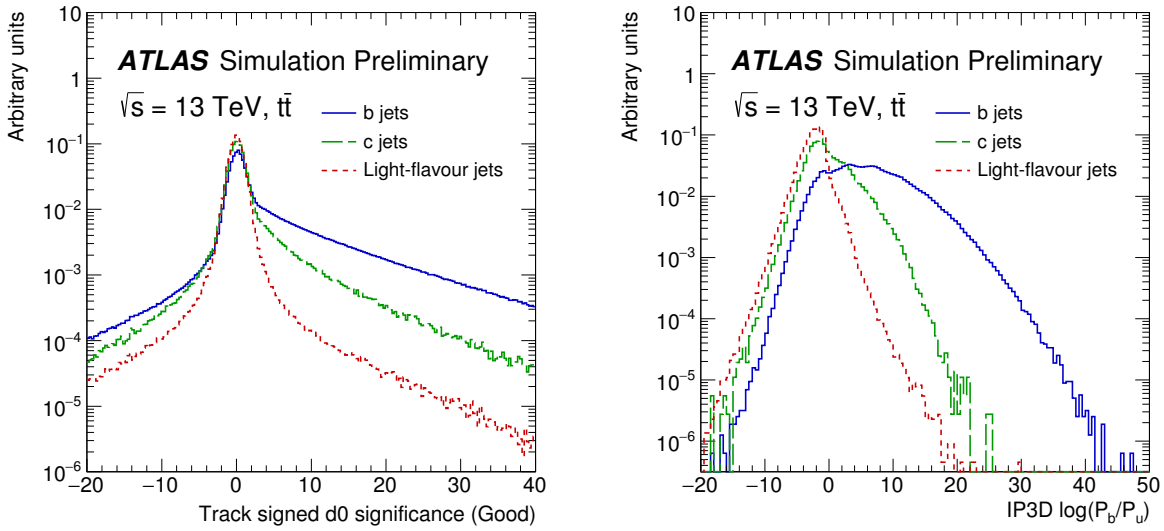
Figure 3.9.: Signed transverse impact parameter significance of good tracks for b -jets, c -jets, and light -jets in t\bar{t} simulated events at \sqrt{s} = 13 TeV (left). Log likelihood ratio of the b -jet against the light -jet hypotheses for the IP3D b-tagging algorithm for b -jets, c -jets, and light -jets in t\bar{t} simulated events at \sqrt{s} = 13 TeV (right) [128].
