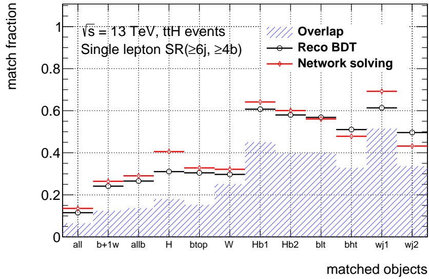
Figure 4.17.: Fraction of events where all jets (all), all b -jets and one of the light -jets from the W -boson decays (b+1w), all b -jets (allb), the two b -jets from the Higgs boson (H), the b -jets from the top-quarks (btop), the light -jets from the W -boson (W), the leading and sub-leading b -jets from the Higgs boson (Hb1 and Hb2 respectively), the b -jet from the leptonic and hadronic tops (blt and bht respectively), the leading and sub-leading light -jets from the W -boson (wj1 and wj2 respectively) are correctly assigned by the reconstruction BDT without Higgs boson variables (black) and the network solving algorithm (red). The hashed band represent the overlap between the two methods, i.e. the fraction of events where the two methods find the same correct candidate.
