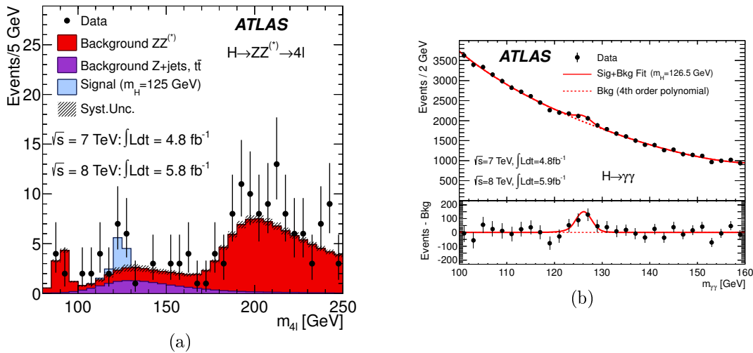
Figure 1.9.: The distribution of the four-lepton invariant mass m_{4l} for the selected candidates in H \rightarrow ZZ^* \rightarrow 4l events (left) and di-photon invariant mass for the selected candidates in H \rightarrow \gamma\gamma events (right), compared to the background expectation, for the combination of the \sqrt{s} = 7 TeV and \sqrt{s} = 8 TeV collected data at the LHC. The signal expectation for a SM Higgs boson with m_H = 125 GeV is also shown for m_{4l} [4].
