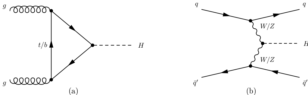
Figure 1.4.: Leading order diagrams for the gluon fusion (left) and vector boson fusion (right) initiated SM Higgs boson production.
