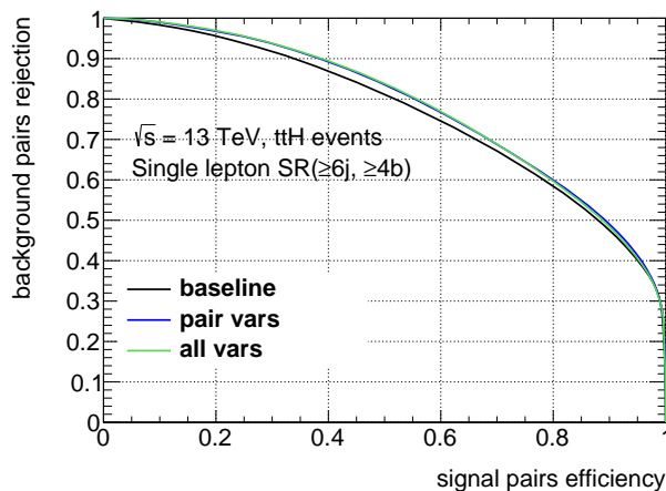
Figure 4.14.: Object pairing BDT performance for several sets of variables. The efficiency to identify pairs of objects originating from different particles is shown as a function of the efficiency to identify pairs of objects originating from the same particle.
