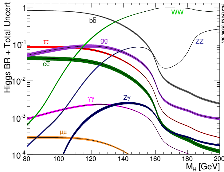
Figure 1.8.: The branching ratios of the SM Higgs boson to various decay modes as a function of its mass [59].
