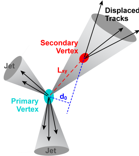
Figure 3.1.: Famous artist view of a b -jet and two light -jets with their track content. The large flight path length L_{xy} of b -hadrons allows to resolve the secondary vertex and to observe tracks with a large transverse impact parameter d_0 .
