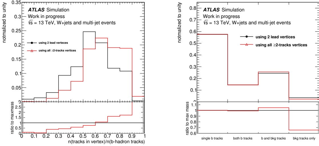
Figure 3.16.: Fraction of tracks coming from b -hadrons found in selected vertices (left) and purity of selected vertices (right). The vertex purity is evaluated separating vertices in four categories: vertices made of tracks originating from a single b -hadron decay chain (first bin), vertices made of tracks originating from both b -hadrons decay chains (second bin), vertices made of b -hadron decay chain tracks and background tracks (third bin), vertices made of only background tracks (fourth bin).
