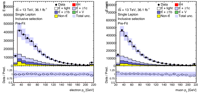
Figure 4.8.: Comparison of the predicted p_T distribution of the electron (left) and muon (right) to the one observed in data using the inclusive single lepton channel selections. The hashed area represent the statistical and systematic uncertainties. The pre-fit uncertainties do not include the effect of the tt + \geq 1b and tt + \geq 1c normalisations which are free parameters of the fit.
