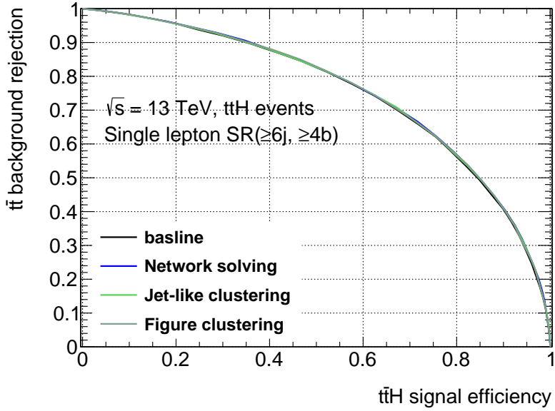
Figure 4.22.: t\bar{t} rejection as a function of the t\bar{t}H efficiency for the baseline classification BDT, or the classification BDTs with additional information from the network based reconstruction.
