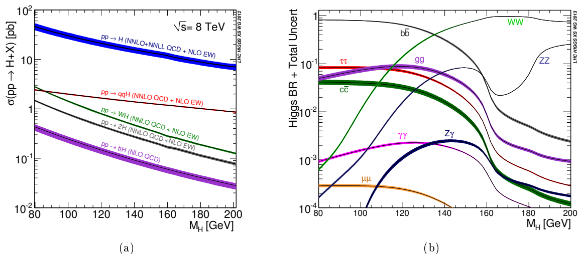
Figure 2.3: (a) Higgs production cross-sections as a function of m_H and (b) Higgs decay branching ratios as a function of m_H
