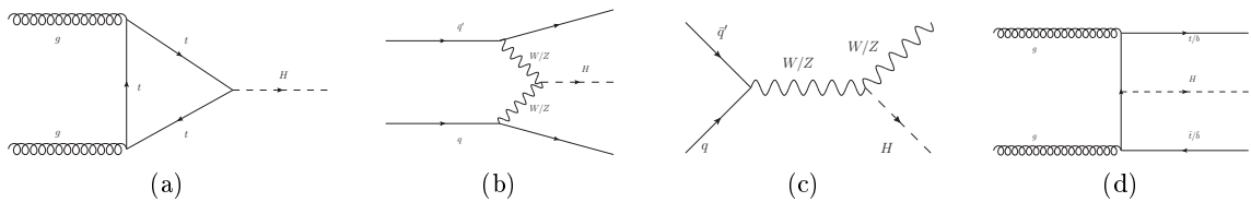
Figure 2.2: Representative leading-order diagrams for the main SM Higgs production modes at LHC: (a) gluon-fusion, (b) Weak-boson fusion, (c) Associated production with a W and Z boson and (d) Associated production with a t\bar{t} pair
