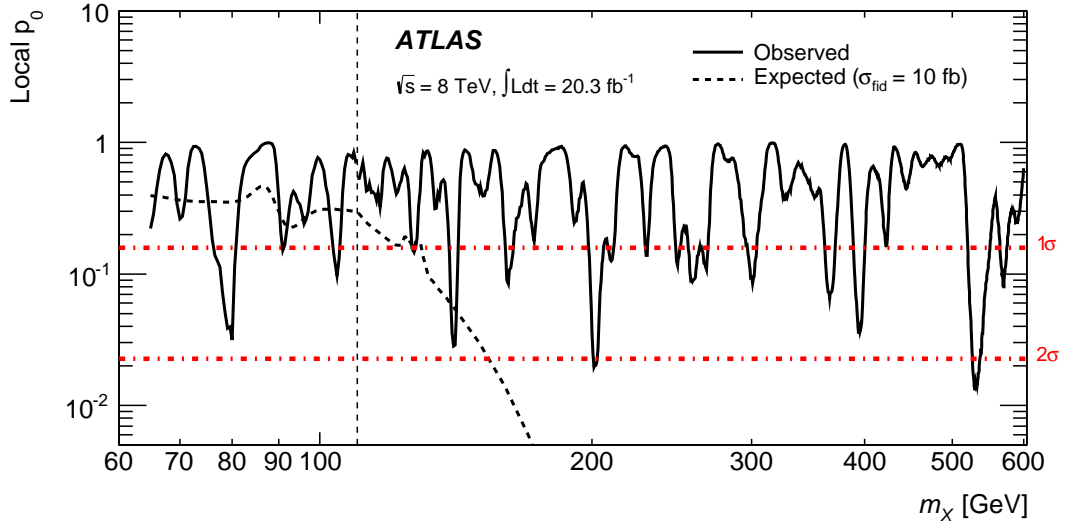
Figure 8.3: Observed (solid line) and expected (dashed line) discovery p-values as a function of m_X , where the expected p-value is computed for \sigma_{fid} = 10 \text{ fb} . The dotted line at m_X = 110 \text{ GeV} show the transition between the low-mass and high-mass analyses. (From Ref. [96])
