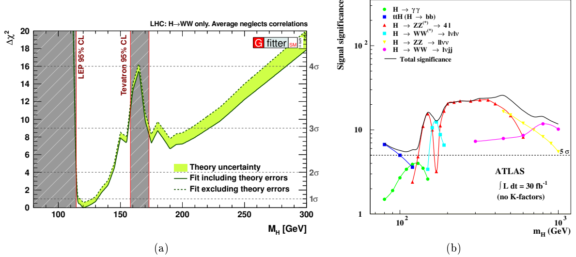
Figure 2.1: (a) \chi^2 scan of m_H from the global fit of SM parameters presented in Ref. [35], using the Gfitter [34] program. (b) Expected discovery significances with 30 \text{ fb}^{-1} of ATLAS data at \sqrt{s} = 14 TeV, as estimated in the ATLAS TDR [36] (1999).
