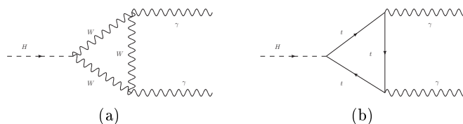
Figure 2.4: Representative leading-order diagrams for H \rightarrow \gamma\gamma : (a) through a W-boson loop, (b) through a t -quark triangle.
