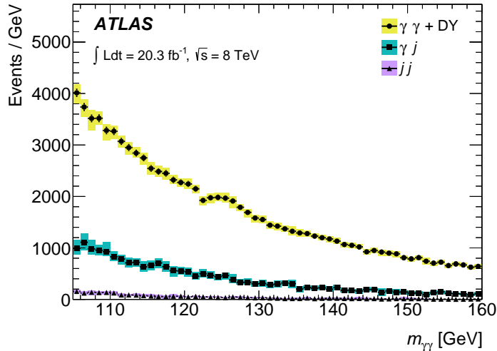
Figure 4.2: Decomposition of the background to the H \rightarrow \gamma\gamma search into \gamma\gamma , \gamma\text{jet} and \text{jetjet} components, for the selection of the final Run 1 analysis described in Section 7.
