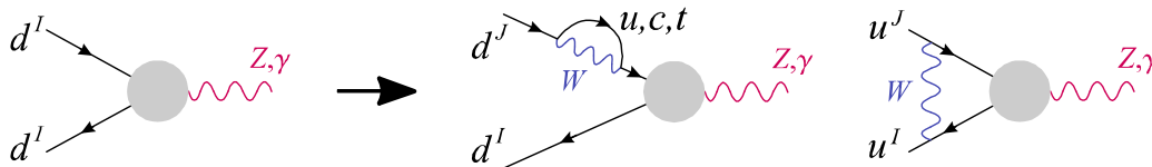
Figure 2.3: Electroweak radiative corrections inducing flavor-violating operators out of a flavor-blind NP couplings Z_\mu \bar{d}^I \gamma^\mu d^I .
