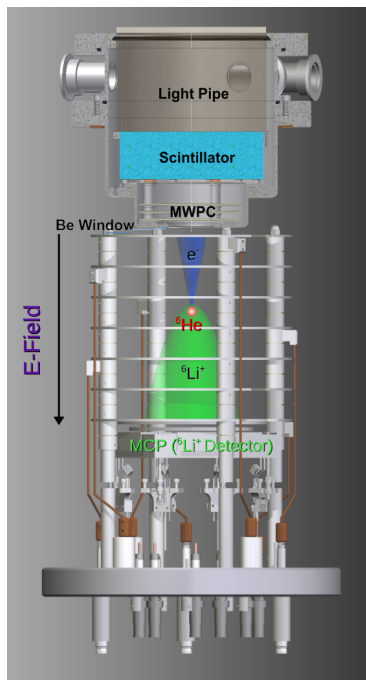
(a) CENPA Detection MOT [Lere15].
