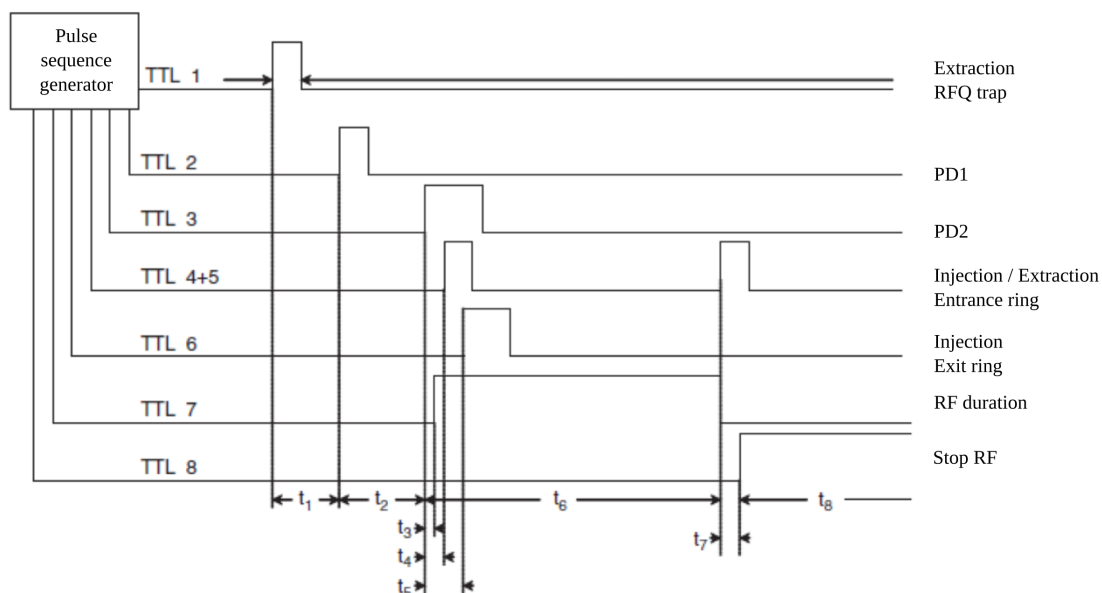
Figure 2.4: Timings overview of the LPCTrap device. For each specific timing, an associated duration is defined such that a given signal starts at its time t_i and has a duration of D_i . PD1 and PD2 are pulse drift tubes (see section 2.2.3).
