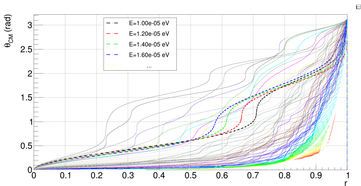
(a) \theta distribution in quantum models for different relative energies in the case of the ^{35}\text{Ar}^+ + ^4\text{He} system [Pons15]. The randomization is not done on the impact parameter, but on a ratio r (see text for details).
