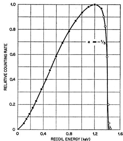
(b) Oak Ridge 1963 experiment typical spectrum [JPC63]. The statistical uncertainties are lower than the size of the points which show the experimental results of a typical dataset. The curve is from theory with SM assumption, the agreement is excellent.
