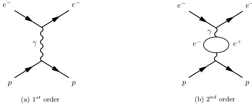
Figure 1.2: EM effective interactions between an electron and a proton
