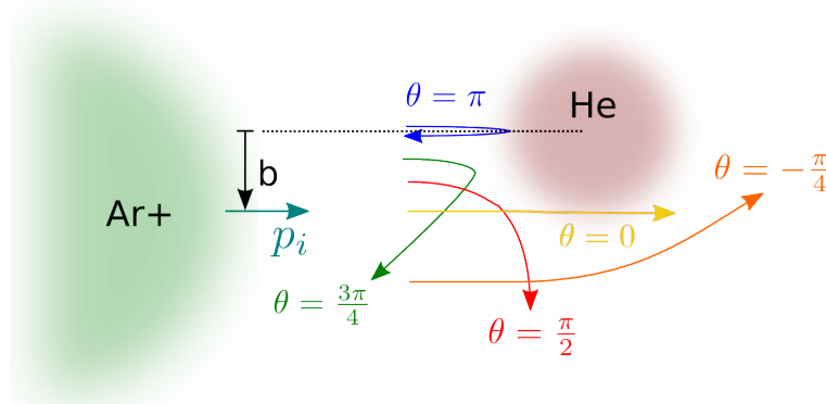
(b) \theta schematic representation. The involved atom and ion must be seen as interacting potentials, not solid objects.
