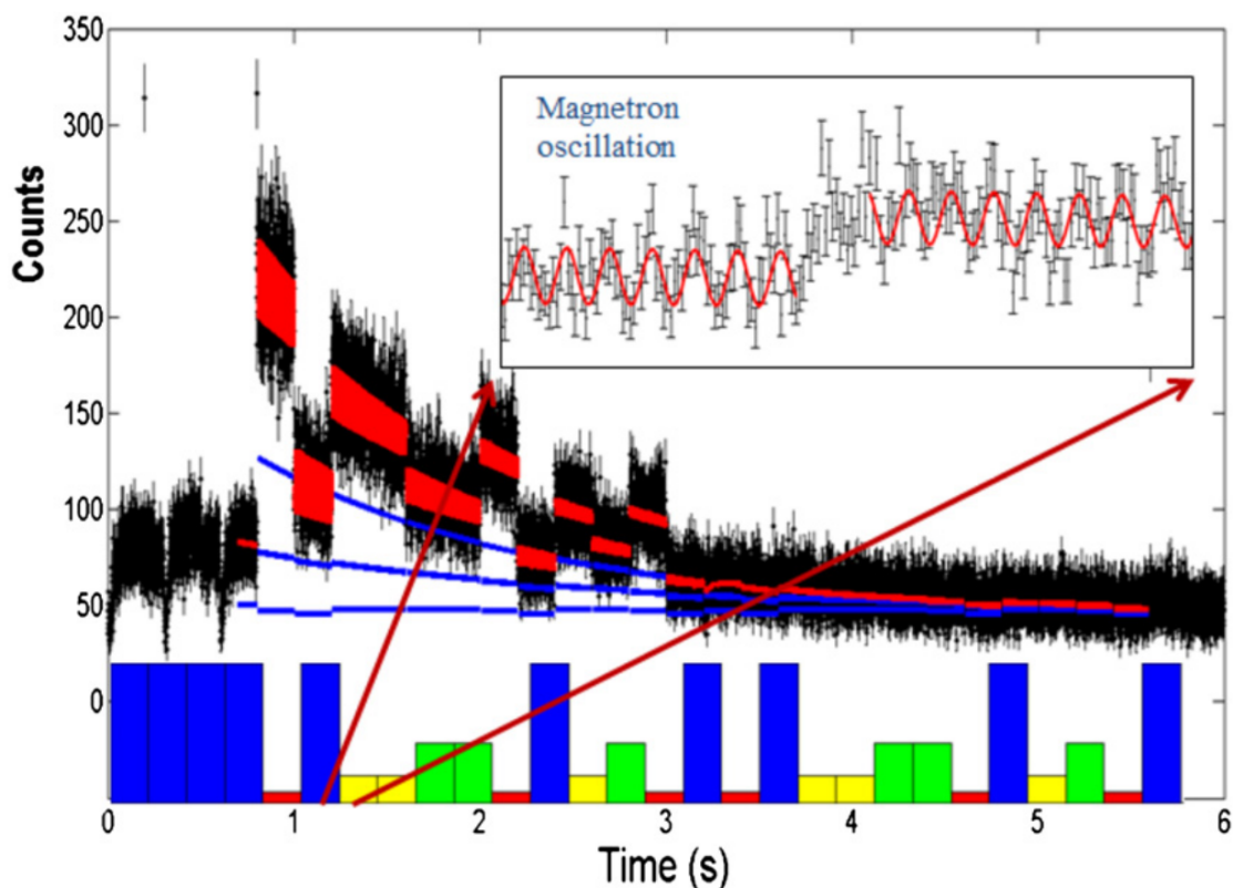
(b) Typical WITCH dataset [Sev14b]. The transfer from the cooler to the decay trap occurs at 0.8\text{ s} while the decay trap is emptied at 3.2\text{ s} . The retardation voltages are shown as the down histogram. The radioactive decay of ^{35}\text{Ar} appears clearly with slices offsets due to the lower counting rate associated with a higher potential barrier. The lines are fits to account for all the components generating the signal.
