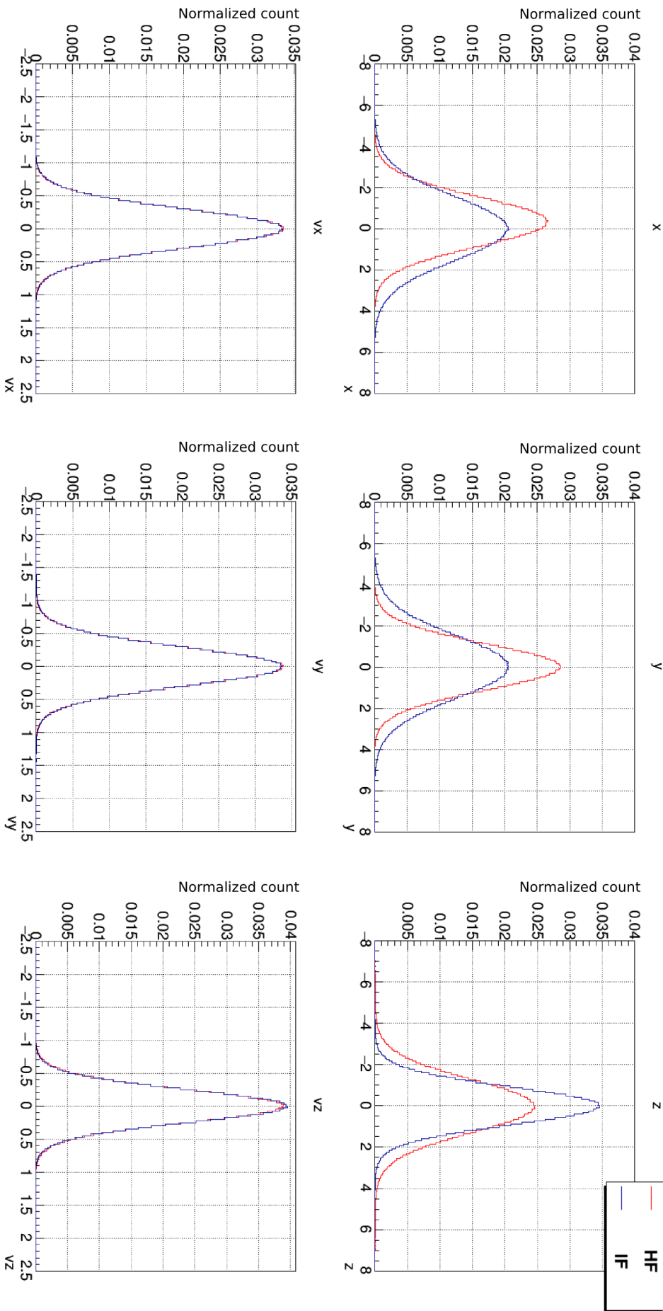
Figure 3.29: Fields effect – Phase space profile taken around \frac{\pi}{2} .
