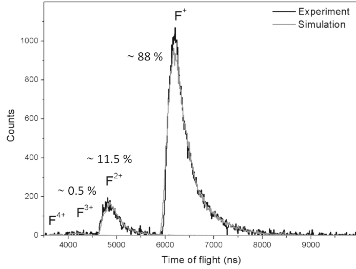
Figure 2.19: 2013 TOF spectrum. We can clearly see the different charge state peaks of the resulting Fluorine [LiHI15].
