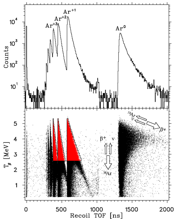
(a) Results from the 2005 experiment. The different charge states of the recoiling Ar appear clearly, the red regions in the bottom canvas correspond to the analysis cuts [GMAA05].
