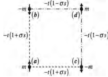
Figure 4 Mean-field like scheme defining the reference Slater determinant for the SEMF approach with spin and total momentum projection.
