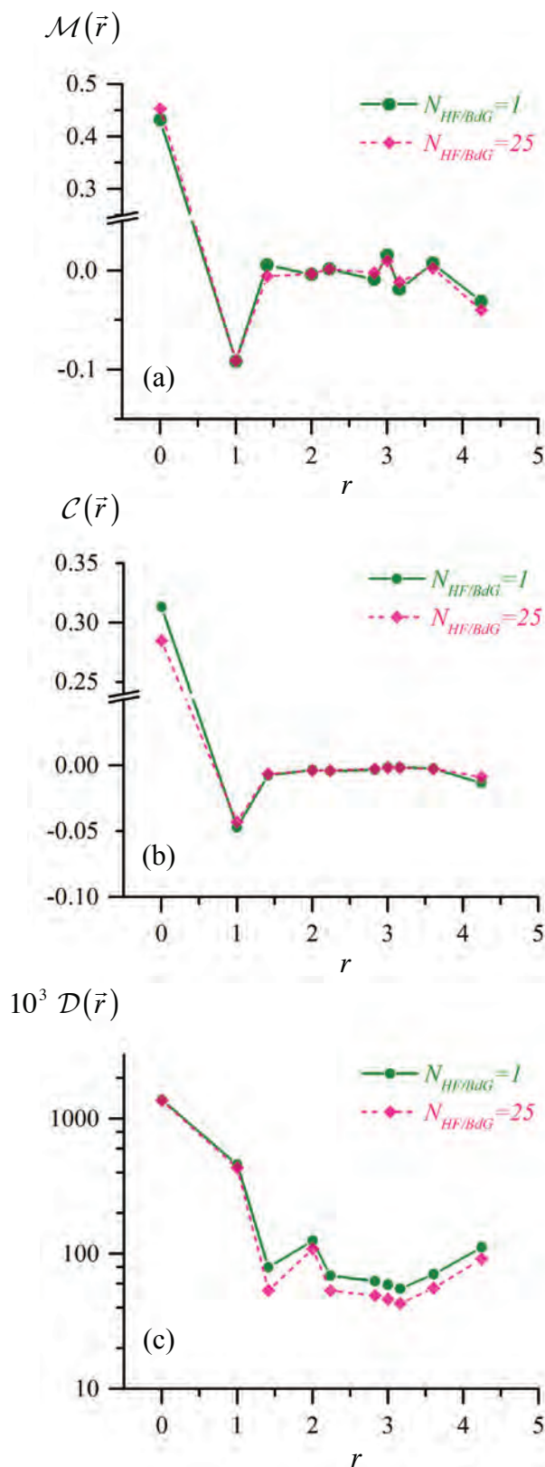
Figure 5. Evolution of (a) spin, (b) density and (c) d -wave pairing autocorrelation functions with the number N_{HF/BdG} of symmetry projected HF/BdG wavefunctions spanning the variational subspace. Calculations are performed for N = 24 atoms on a 6 \times 6 cluster with an interaction strength U/t = 8 .
