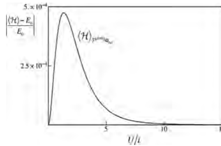
Figure 2 Ground-state energy from spin singlet projected SEMF.
