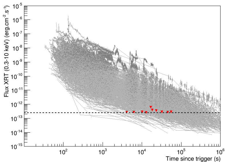
Figure 5.19: Gray lines: 689 X-ray afterglow fluxes in the energy band from 0.3 to 10 keV detected by the Swift -XRT from 2007 to 2015 as a function of time. The upper limits on GRB fluxes for 10 neutrino alerts are represented by red triangles. The horizontal dashed line corresponds to the sensitivity reached with a 2 ks exposure.
