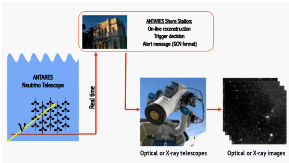
Figure 3.1: Illustration of the TAToO alert system implemented in the ANTARES experiment.
