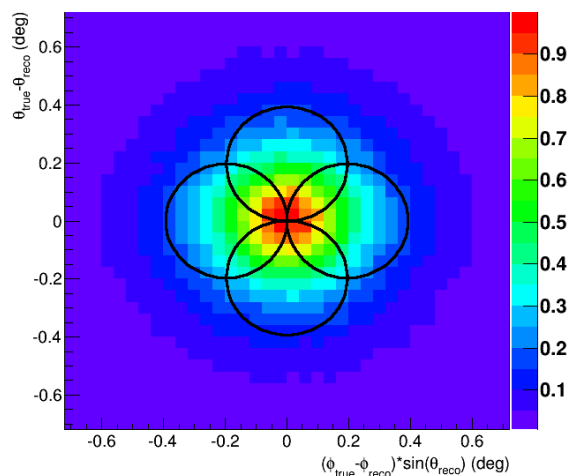
Figure 3.20: Each Swift -XRT observation of an ANTARES trigger consists of 4 tiles (black circles), which cover an area of radius of \sim 0.4^\circ . With such a mapping, 72 % of the bi-directional uncertainty of a TAToO alert is covered.
