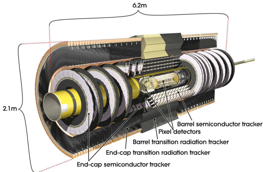
Figure 2.5 Cut-away view of the ATLAS inner detector. [12]
