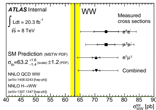
Figure 3.30 Overview plot: WW cross sections measured at \sqrt{s} = 8 TeV compared to the NNLO prediction [30]
