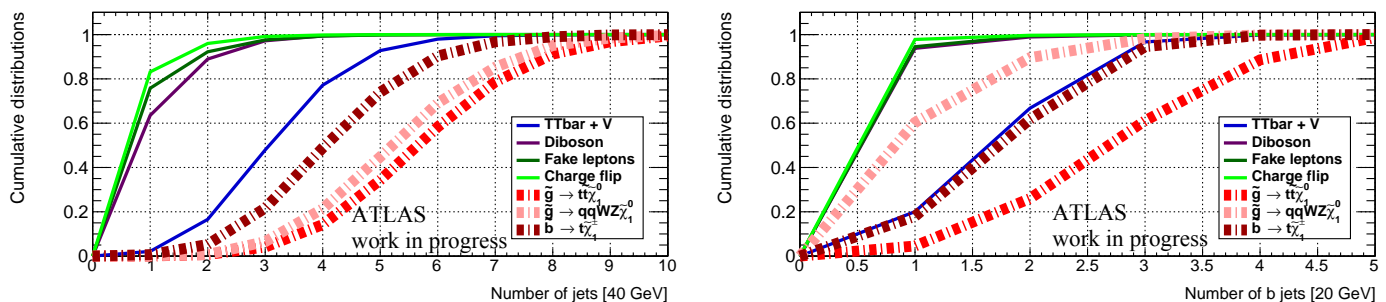
Figure 7.5: Cumulative distribution showing the importance of a cut on number of jets (left) and b jets (right). Distributions shown after requiring two same - sign or three signal leptons in the event ( \sqrt{s} = 8 TeV, L = 20.3 fb ^{-1} ).
