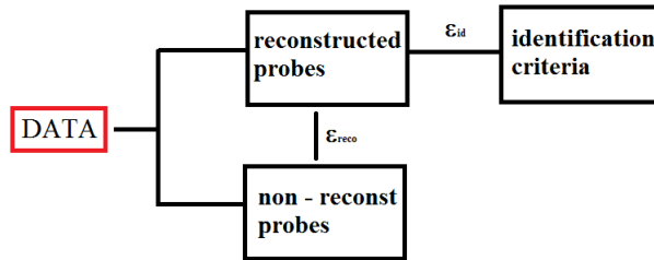
Figure 5.2: Illustration of different stages used for electron efficiency measurement.
