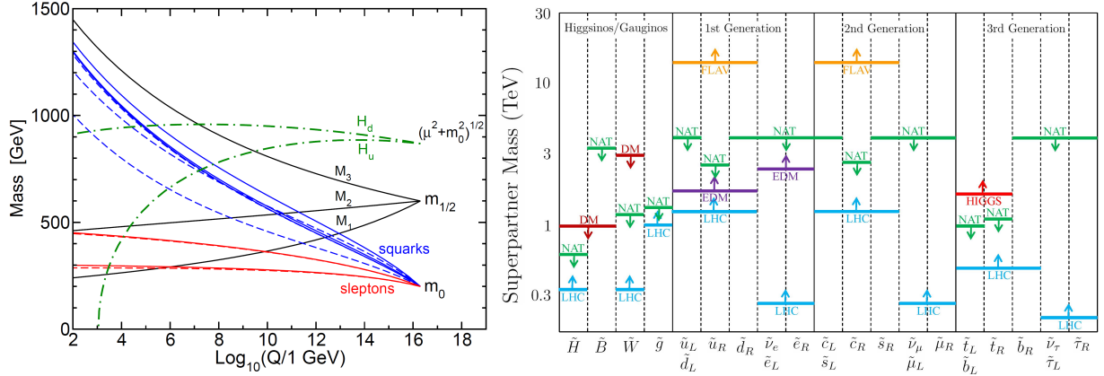
Figure 2.6: Left : Evolution of the scalar and gaugino mass parameters in MSSM, when the boundary conditions are imposed at the GUT scale [100]. Plot made in the mSUGRA model framework with \tan\beta = 10 , m_0 = 200 GeV, m_{1/2} = -A_0 = 600 GeV and \sin(\mu) = 1 ; Right : A natural SUSY spectrum given the constraints mentioned in the text [114].
