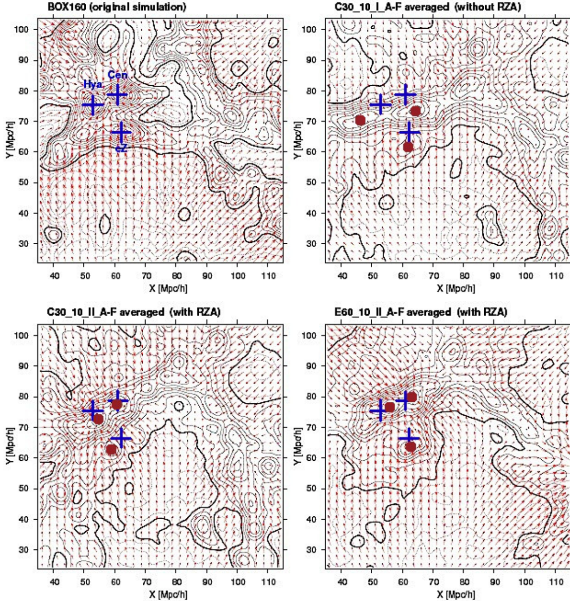
FIGURE 1.3: Density and velocity fields in a 10 \text{ h}^{-1} \text{ Mpc} thick slice of the original first constrained simulation, named BOX160, of the CLUES project ( top left quadrant ) and the averages of six constrained simulations obtained with mocks built out of BOX160. The constrained Initial Conditions have been obtained without ( top right ) and with the Reverse Zel'dovich Approximation applied to simple mocks mimicking the size and spatial extent of Cosmicflows' first ( bottom left ) and second catalogs ( bottom right ). Blue crosses show the positions of three clusters in the original simulation while red dots locates the clusters in the constrained simulations on average (adapted from Doumler et al., 2013b ).
