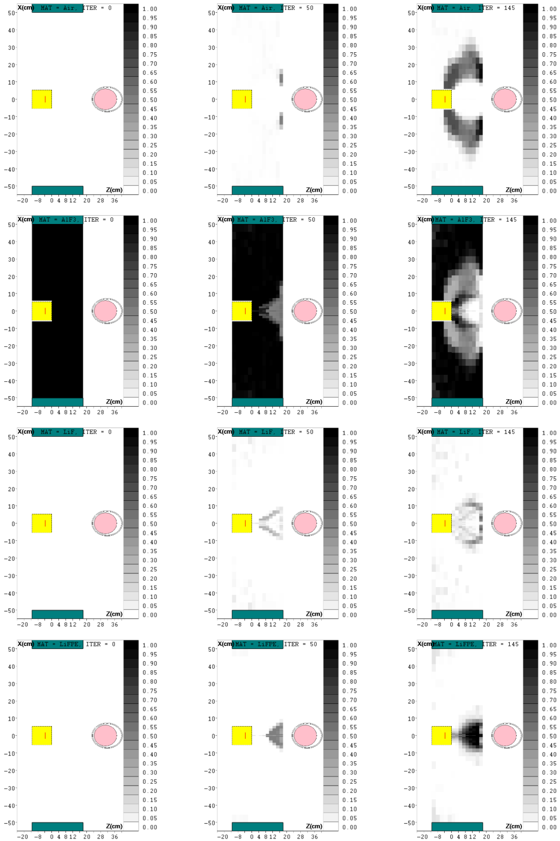
Figure 2. Convergence of the TopOpt algorithm towards the solution of problem (1) for an Air-AIF 3 -LiF-LiFPE BSA, for L = 18 cm, R = 50 cm and a {}^7\text{Li} ( p(2.5 \text{ MeV}), n ) source. The figures in the left column give the BSA structure at iteration 0, those in the middle column give the structure at iteration 50, and those on the right column give the final structure, at convergence. The 1 st line gives the volume fractions of air in the structure, the 2 nd those of AIF 3 , the 3 rd those of LiF, and the 4 th line those of LiFPE.
