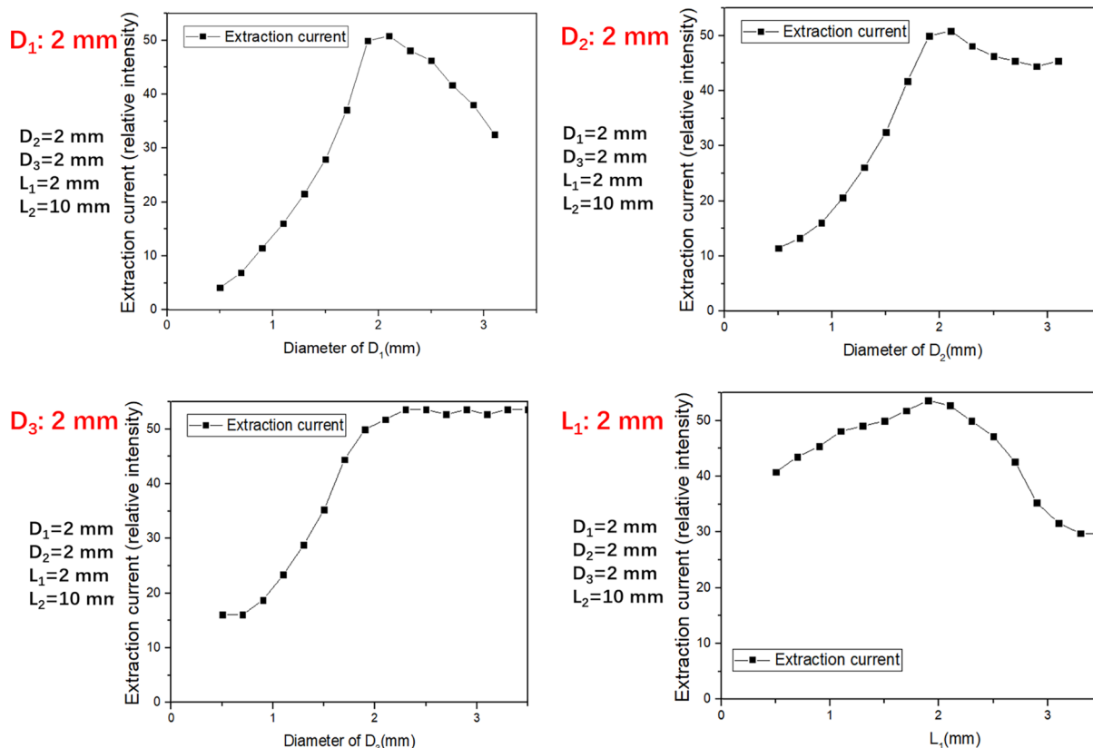
Fig. 6. Simulation results for the electrode geometrical parameters.
