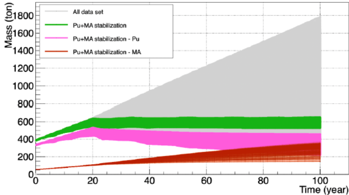
Fig. 14. Total transuranic mass evolution in the fleet (gray lines). The green lines represent the sum of plutonium and minor actinides masses for trajectories obtained by stabilization criteria. Purple lines are plutonium mass evolution and red lines are minor actinides mass evolution after the application of the same criteria.
