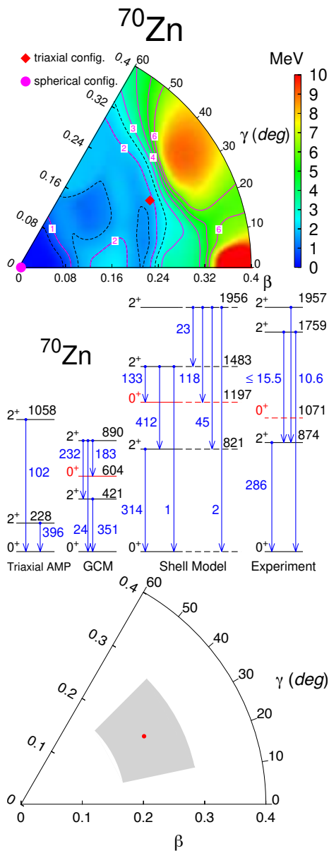
FIG. 9. (Color online) (top) Potential Energy Surface from constrained Hartree-Fock minimization in the shell-model basis for ^{70}\text{Zn} . (middle) Level scheme and B(E2) values (in MeV and e^2\text{fm}^4 , respectively) for different theoretical models described in the text and from the present experiment (except for the 2_3^+ state observed in another work and whose B(E2) value is unknown). (bottom) 1\sigma contours in the \beta - \gamma sextant for the ground-state of ^{70}\text{Zn} . The red dot represents the effective \beta and \gamma value.
