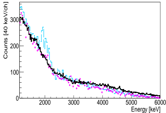
FIG. 7. (Color online) Comparison between the experimental Doppler-corrected energy spectrum for a ^{68}\text{Ni} beam on a C target (solid black histogram) and simulated spectra assuming \beta_N = 0.1 (magenta stars) and \beta_N = 0.2 (dashed blue histogram). The adopted value of \beta_N = 0.102(8) , as deduced from the study with the Pb target, is too small for a peak to be seen when ^{68}\text{Ni} scatters off the C target.
