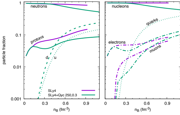
FIG. 3: Particle fractions for the SLy4 nucleon model and the quarkyonic model taking \Lambda_{\text{Qyc}} = 250 MeV and \kappa_{\text{Qyc}} = 0.3 .
