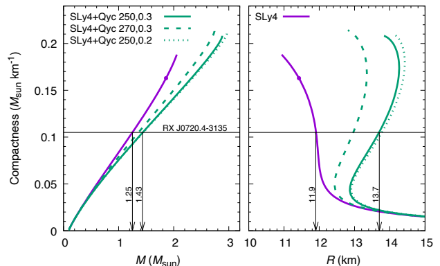
FIG. 7: Compactness (M/M_\odot)/(R/\text{km}) as function of the mass M/M_\odot (left) and radius (right) for various sets of the parameters \Lambda_{Qyc} and \kappa_{Qyc} fixed to be as in Fig. 4.
