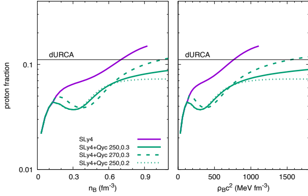
FIG. 4: Comparison of the proton fraction in the pure nucleon model with the prediction of the quarkyonic model for various sets of the parameters (\Lambda_{\text{Qyc}}, \kappa_{\text{Qyc}}) : (250, 0.3) , (270, 0.3) and (250, 0.2) . Left: function of the particle density in \text{fm}^{-3} , right: function of the energy density \rho_B c^2 in \text{MeV fm}^{-3} .
