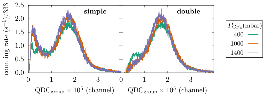
Figure 34 – Spectra resulting from the first (simple) and second (double) phases of the background subtraction method. Three different \text{CF}_4 pressures are studied. The double subtraction reveals the edge events region.
