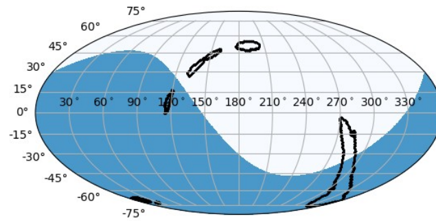
GW170729
