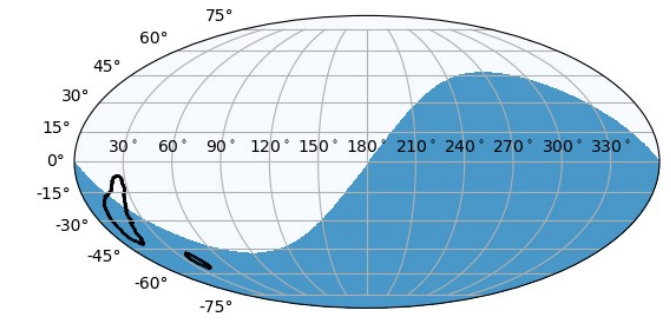
GW170809
