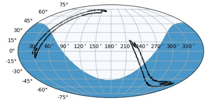
GW170823
