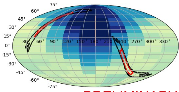
GW170823
