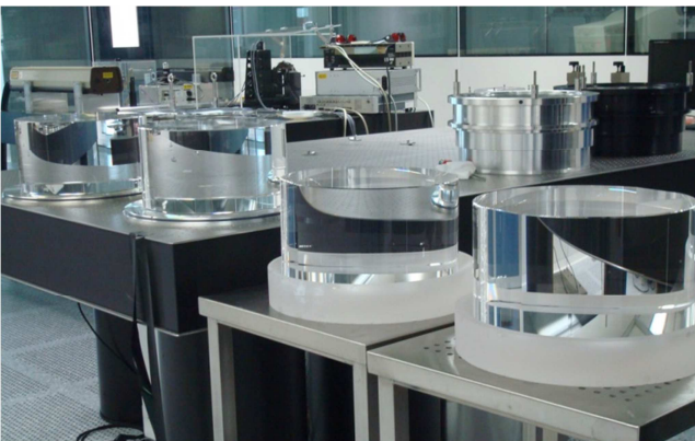
Fig. 2: Four Advanced LIGO ITM substrates before coating
