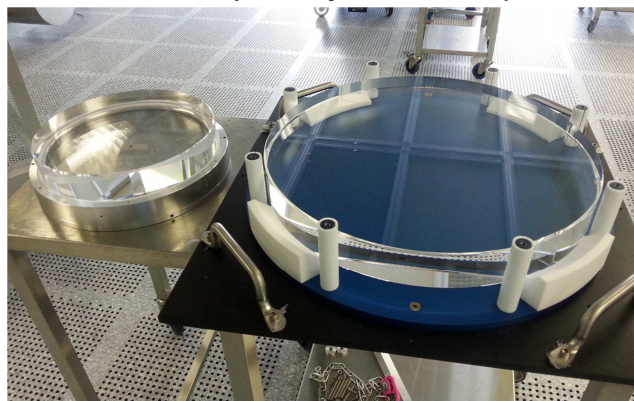
Fig. 1: Advanced Virgo recycling mirror Ø35 cm (left) and large Beam Splitter Ø55 cm (right)
