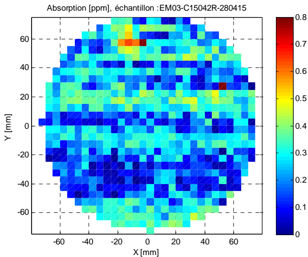
Fig. 5: Absorption map at 1064 nm on Ø15 cm of a high reflectivity coating of an EM of Advanced Virgo
