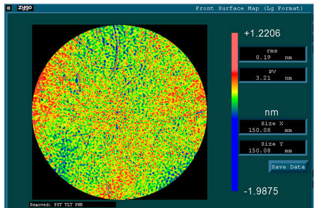
Fig. 4: Surface flatness (0.19 nm RMS Ø15 cm) of an Advanced Virgo EM
