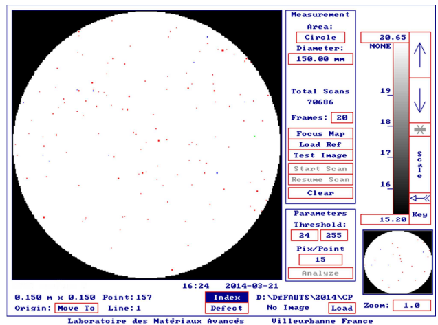
Fig. 3: Point defect map Ø15 cm of an Advanced Virgo EM
