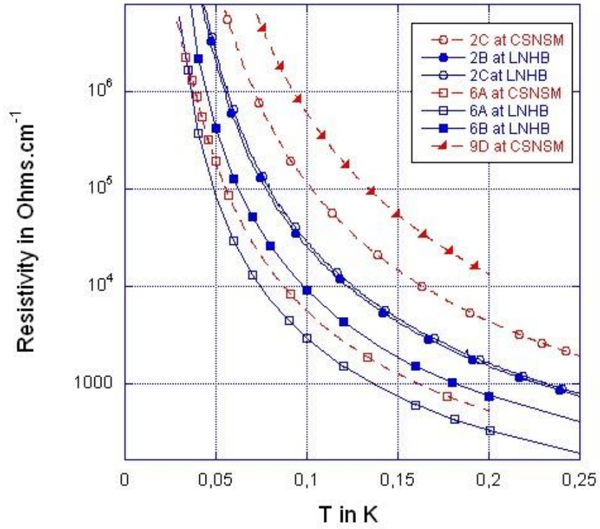
Fig. 1 Left: Resistivity \rho(T) curves for different NTD wafers and different irradiations (2, 6 and 9 correspond to 2.93 , 3.2 and 2.76 \cdot 10^{18} \text{ n}\cdot\text{cm}^{-2} resp.). Samples 2C, 6A and 9D (red dashed line) were measured at CSNSM in Orsay; 2B, 2C, 6A and 6B (blue solid line) at LNHB in Saclay. Errors on the resistivity measured with a Wheatstone bridge TRMC2 (Air Liquide) are lower than 1%. (Color figure online)
