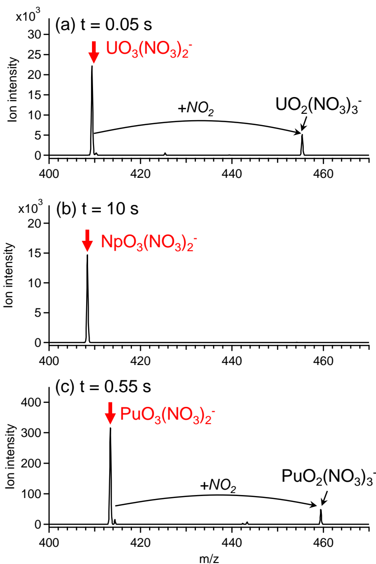
Figure 3. Mass spectra acquired after reaction of isolated \text{AnO}_3(\text{NO}_3)_2^- indicated in red with \text{NO}_2 at the same pressure but different reaction time t : (a) \text{An} = \text{U} , t = 0.05 s; (b) \text{An} = \text{Np} , t = 10 s; (c) \text{An} = \text{Pu} , t = 0.55 s. The product of reaction (3) is apparent in (a) and (c) but not (b). The minor peaks at 1 m/z higher than the reactant peaks in (a) and (c) are assigned as \text{AnO}_2(\text{OH})(\text{NO}_3)_2^- ; the source of the H atoms is indeterminate but could be \text{HNO}_2 , which is a facile H-atom donor.
