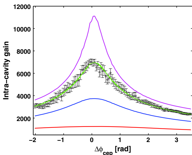
Fig. 3. Effective power enhancement factor inferred from the experimental data as a function of \Delta\phi_{ce} for finessses of 5000 (red), 15,000 (blue), 28,000 (green), and 45,000 (pink).
