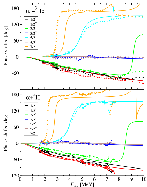
Fig. 2. (Color online.) The \alpha + {}^3\text{He} and \alpha + {}^3\text{H} elastic phase shifts obtained from the NCSM approach and from experiments [52,53]. Energies are given with respect to the \alpha + {}^3\text{He}/{}^3\text{H} threshold.
