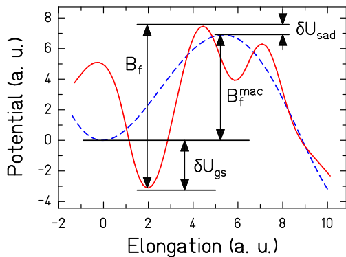
Figure 12: (Color online) Schematic drawing of the potential energy on the fission path relative to the macroscopic ground-state energy E_{gs}^{mac} for a nucleus that is deformed in its ground state. Spherical shape corresponds to zero elongation. Blue dashed line: macroscopic potential. Red full line: full potential including the shell effects. The figure is taken from Ref. [344] with kind permission of The European Physical Journal (EPJ).
