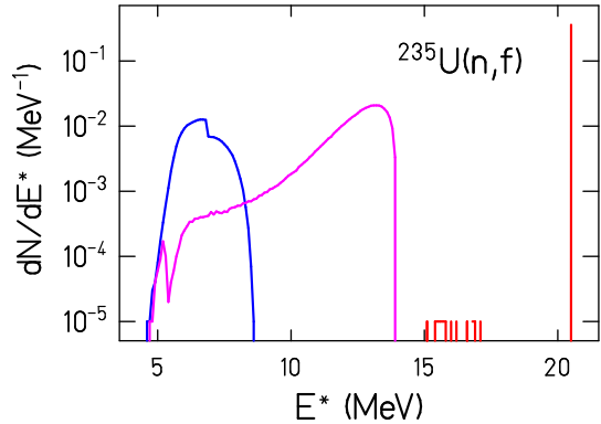
Figure 16: (Color online) Distribution of excitation energies E^* at fission for the system ^{235}\text{U}(n,f) at E_n = 14 MeV. E^* is the excitation energy of the compound nucleus above its ground state, before it passes the fission barrier towards scission. The right-most peak shows events from first-chance fission (fission of ^{236}\text{U} ), the middle curve corresponds to second-chance fission (fission of ^{235}\text{U} ), and the left curve corresponds to third-chance fission (fission of ^{234}\text{U} ). The broad distribution around 16 MeV corresponds to gamma emission before fission. The figure is modified from Ref. [224].
