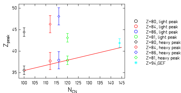
Figure 25: (Color online) Mean positions of the asymmetric fission components of the mass distributions shown in figure 22 (beta-delayed fission of the compound nuclei ^{180}\text{Hg} , ^{196}\text{Po} , and ^{202}\text{Rn} ) and figure 23 ( ^{201}\text{Tl} at 7.4 MeV above the fission barrier). The mass values were transformed into proton numbers by the UCD assumption. In addition, the mean number of protons in the light fragment of the fission of Pu isotopes, belonging to the S1 fission channel, is shown.
