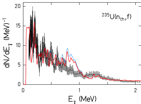
Figure 36: (Color online) Low-energy part of the experimental gamma-energy spectrum (black line with error bars) [160] for thermal-neutron-induced fission of ^{235}\text{U} in comparison with the GEF prediction (red full line). The GEF result is convoluted with the experimental energy resolution. In addition, the calculated spectrum that includes the known delayed isomeric gamma transitions reported in JEF 3.1.1 is shown by the light blue line.
