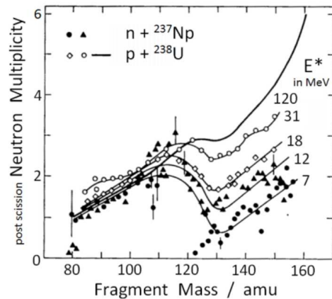
Figure 28: Post-scission mean prompt-neutron multiplicities as a function of fragment mass for different systems. The lines are drawn to guide the eye. The initial excitation energy of the fissioning system is listed. The figure is taken from [410].
