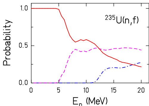
Figure 15: (Color online) Relative contributions of the different fission chances in the system ^{235}\text{U}(n,f) as a function of the incident-neutron energy. Full line: first-chance fission, dashed line: second-chance fission, dot-dashed line: third-chance fission. The figure is modified from Ref. [224].
