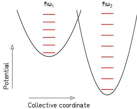
Figure 19: (Color online) Schematic drawing of the potential energy as a function of a collective coordinate that is orthogonal to the fission direction at a fixed elongation. In the present context, the two harmonic oscillator potentials with different depths and \hbar\omega values represent the potential in two fission valleys for mass-asymmetric distortions that are related to different fission channels. The energies of the stationary states are indicated by the red horizontal lines. The overlapping of the two potential-energy curves illustrates the possibility that the fission valleys are divided by a higher ridge that becomes perceptible when a continuous transition from one valley to the other is established in a deformation space with a sufficiently high dimension, see for example Ref. [366]. The figure is taken from Ref. [224] with kind permission of The European Physical Journal (EPJ).
