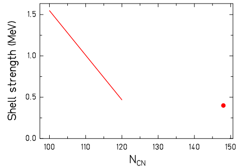
Figure 26: (Color online) Line: Strength of the shell that is responsible in GEF for the asymmetric fission valley of the systems shown in figures 22 and 23. The full symbol denotes the strength of the shell in the light fragment that enhances the S1 fission channel in the Pu isotopes. See text for details.
