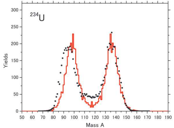
Figure 10: (Color online) Mass distribution of fission fragments of ^{234}\text{U} at E^* = 20 MeV. Calculation [324] and evaluated data [325] are denoted by histogram and circles, respectively. In contrast to the evaluated data, the calculation does not include the influence of multi-chance fission and prompt-neutron emission from the fragments. The figure is taken from Ref. [324].
