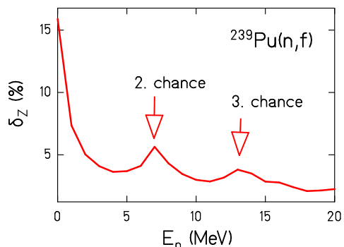
Figure 38: (Color online) Global odd-even effect (\Sigma(Y_{\text{even}} - Y_{\text{odd}})/\Sigma(Y_{\text{even}} + Y_{\text{odd}})) in the fission-fragment Z distribution of the system ^{239}\text{Pu}(n,f) as a function of the incident neutron energy from the GEF code.
