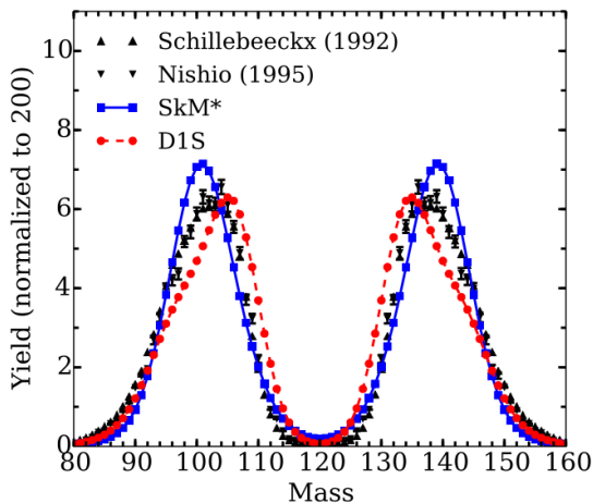
Figure 6: (Color online) Pre-neutron mass yields for ^{239}\text{Pu}(n,f) . The calculations by Regnier et al. [76] obtained with the Skyrme (SKM*) and Gogny (D1S) effective nuclear potentials are compared with the experimental datasets by Schillebeeckx and Nishio. Figure taken from [76].
