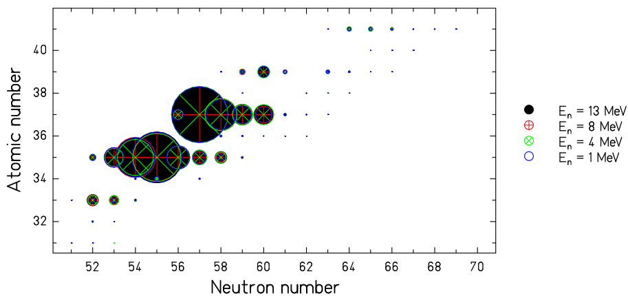
Figure 39: (Color online) Beta-delayed neutron yields in the light fission-fragment group from neutron-induced fission of ^{238}\text{U} for different incident neutron energies on the chart of the nuclides, calculated with the GEF code (version Y2017/V1.2). The radius of the symbol is proportional to the yield.
