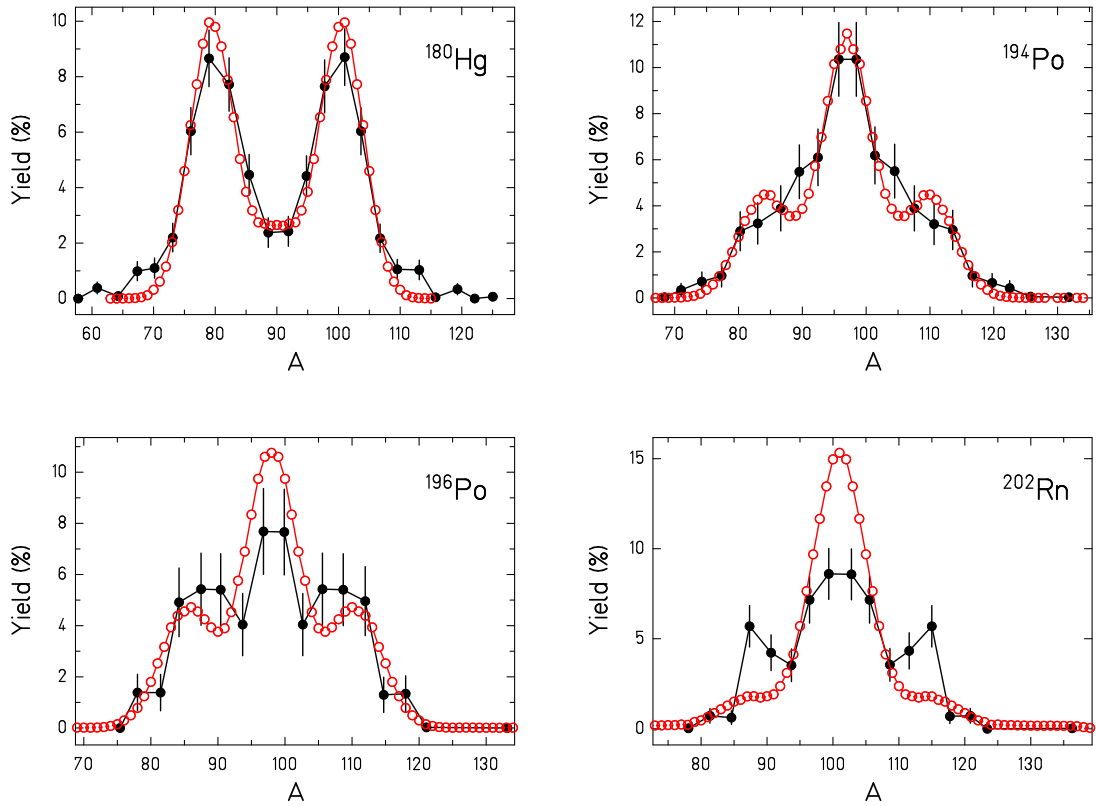
Figure 22: (Color online) Measured pre-neutron fission-fragment mass distributions from beta-delayed fission of the compound nuclei ^{180}\text{Hg} , ^{194}\text{Po} , ^{196}\text{Po} , and ^{202}\text{Rn} [142, 153] (full black symbols) in comparison with the result of the GEF code (GEF 2017/V1.2) (open red symbols).
