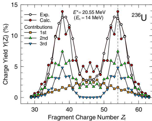
Figure 11: (Color online) Calculated fission-fragment nuclear-charge distributions at 14 MeV incident-neutron energy, corresponding to 20.55 MeV excitation after neutron absorption. The contributions from first-, second-, and third-chance fission to the charge distribution are shown and added up to a total yield. The fractions of the fission events from the different chances were taken from Ref. [329]. An experimental evaluation [325] is also shown. The figure is taken from Ref. [88].
