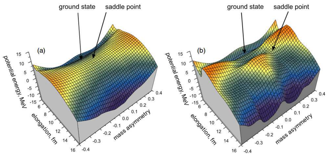
Figure 17: (Color online) Macroscopic (a) and macro-microscopic (b) potential energy surface for the ^{238}\text{U} nucleus as a function of elongation and mass asymmetry. The macroscopic part is normalized to zero for the spherical shape of the compound nucleus. See Ref. [345] for details. The figure is taken from Ref. [345].
