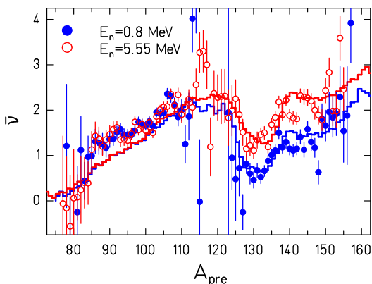
Figure 29: (Color online) Measured prompt-neutron multiplicity in ^{237}\text{Np}(n,f) as a function of pre-neutron fragment mass at two different incident-neutron energies [403] (data points) in comparison with the result of the GEF model [224] (histograms). The figure is taken from Ref. [341].
