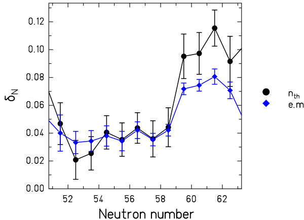
Figure 1: (Color online) Logarithmic four-point differences \delta_n [272] in the fission-fragment neutron-number distribution for electromagnetic-induced fission of ^{238}\text{U} measured in the SOFIA experiment [273] and in thermal-neutron-induced fission of ^{235}\text{U} [274]. The figure shows the most relevant data in the range that contains about 90% of the N distribution of the system ^{235}\text{U}(n_{th},f) in the light fission-fragment group.
