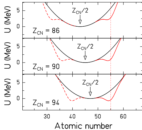
Figure 18: (Color online) Schematic illustration of the potential energy for mass-asymmetric shape distortions on the fission path, after a qualitative idea of Itkis et al. [360]. The black curve shows the macroscopic potential that is minimum at symmetry, while the red curve includes the extra binding due to an assumed additional potential well appearing at Z=55 in the heavy fragment. The assumed well position at Z=55 reflects the measured position of the asymmetric fission-fragment component (see figure 20). It is unclear, whether this is an indication for a proton shell around Z=55 , see section 5.4. The figure is taken from Ref. [224].
