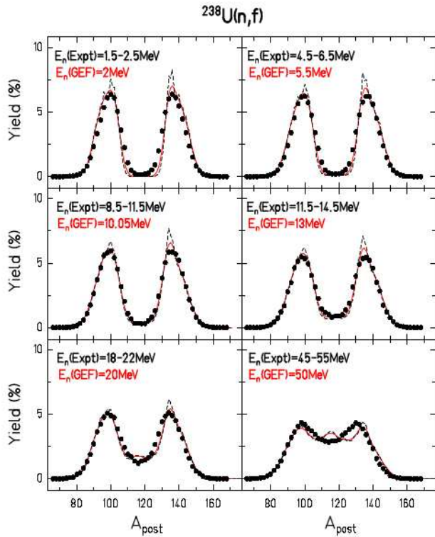
Figure 31: (Color online) Measured fission-fragment mass distributions from neutron-induced fission of ^{238}\text{U} for a series of incident-neutron energies [419] (black symbols) in comparison with the GEF-model results without (black dashed line) and with (red full line) account of experimental resolution. The neutron-beam-energy interval in the experiment as well as the energy used for GEF are indicated. The figure is taken from [418].
