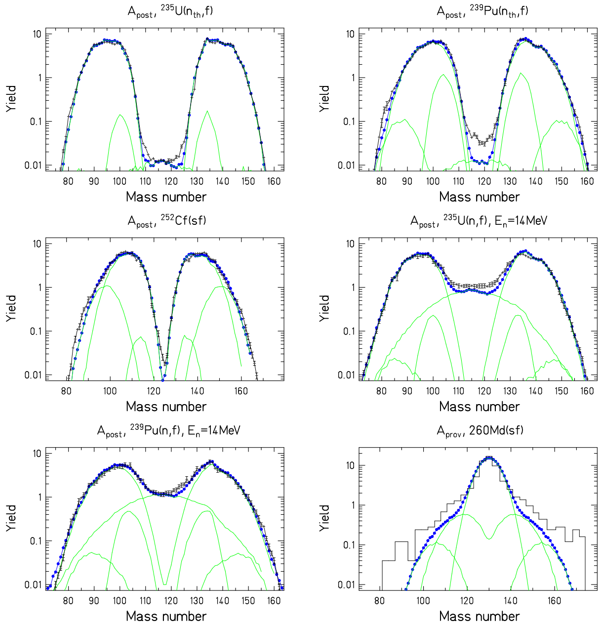
Figure 21: (Color online) Evaluated and measured mass distributions (black symbols) of fission fragments in comparison with the result of the GEF model (blue symbols). The mass distributions after prompt-neutron emission are taken from the evaluation of Ref. [379]. The provisional masses from spontaneous fission of ^{260}\text{Md} (black histogram) were directly deduced from the ratio of the fragment energies with a finite resolution of about 4 mass units without applying a correction for prompt-neutron emission. The data of the corresponding mass distribution are taken from Ref. [235]. The green lines show the calculated contributions from the different fission channels. The figure is taken from Ref. [344] with kind permission of The European Physical Journal (EPJ).
