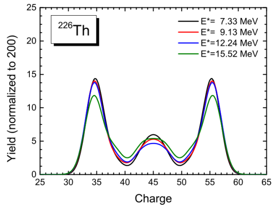
Figure 8: (Color online) Nuclear-charge distribution of fission fragments for different excitation energies. Figure taken from [95].
