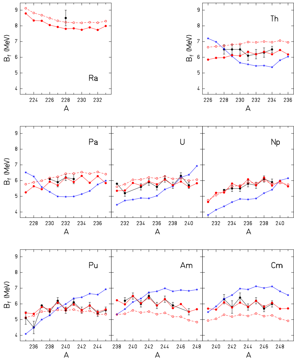
Figure 13: (Color online) The empirical fission threshold of Ref. [98] (full black circles) is compared to the value (open red circles) estimated from the topographic theorem according to equation (6) for isotopic sequences of different elements. In addition, a modified estimation (full red circles) with a Z -dependent shift and an assumed increased pairing parameter \Delta_f = 14/\sqrt{A} MeV at the barrier (see text and Ref. [344]) as well as the theoretical prediction of the microscopic-macroscopic approach of Ref. [353] (blue asterisks) are shown. Empirical values without error bars are given without an uncertainty range in Ref. [98]. The figure is taken from Ref. [344] with kind permission of The European Physical Journal (EPJ).
