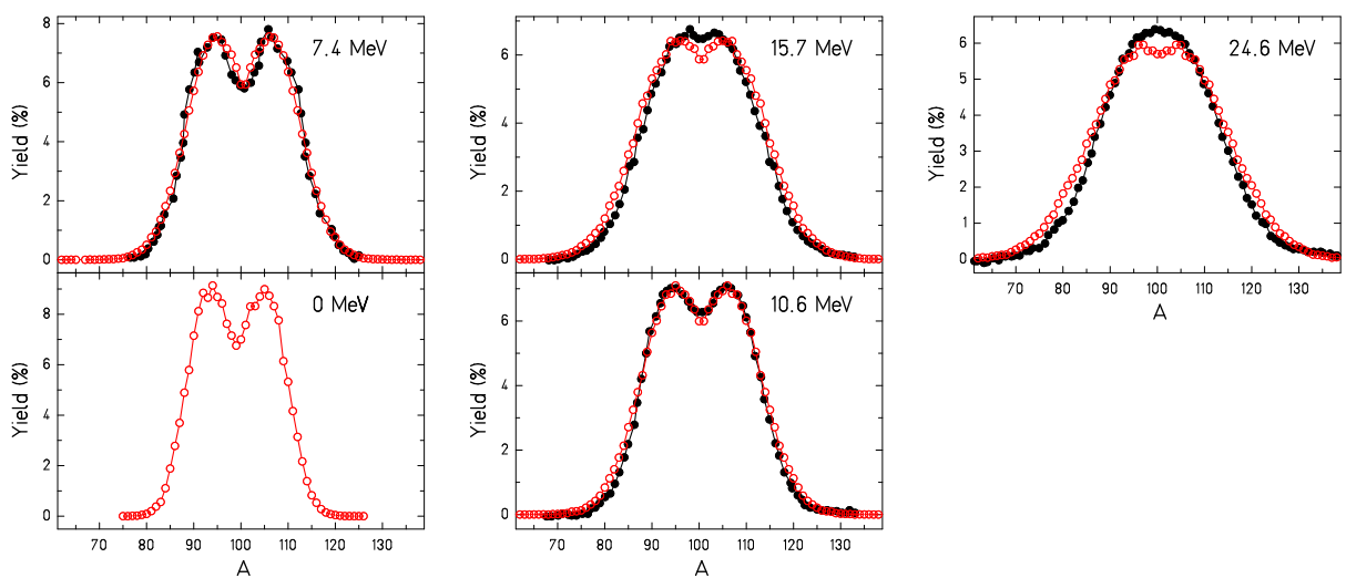
Figure 23: (Color online) Measured pre-neutron fission-fragment mass distributions from proton-induced fission of the compound nucleus ^{201}\text{Tl} [250] (full black symbols) in comparison with the result of the GEF code (GEF 2017/V1.2) (open red symbols). The excitation energies above the fission barrier are indicated.
