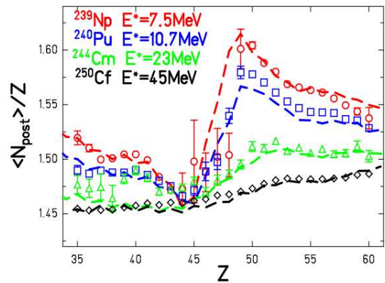
Figure 32: (Color online) Mean post-neutron fragment N/Z ratio as function of fragment Z for various fissioning systems as measured at VAMOS (symbols) [420], and compared with GEF calculations (dashed lines). The figure is taken from [418].
