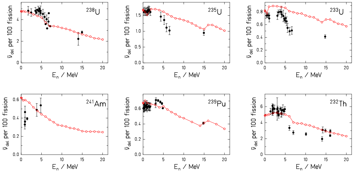
Figure 37: (Color online) Probability for the emission of delayed neutrons for neutron-induced fission of different systems as a function of the incident-neutron energy. Experimental data (full black symbols) from Experimental Nuclear Reaction Data (EXFOR) [442] are compared with the result of the GEF code (version Y2017/V1.2) (open red symbols, connected by red lines.)
