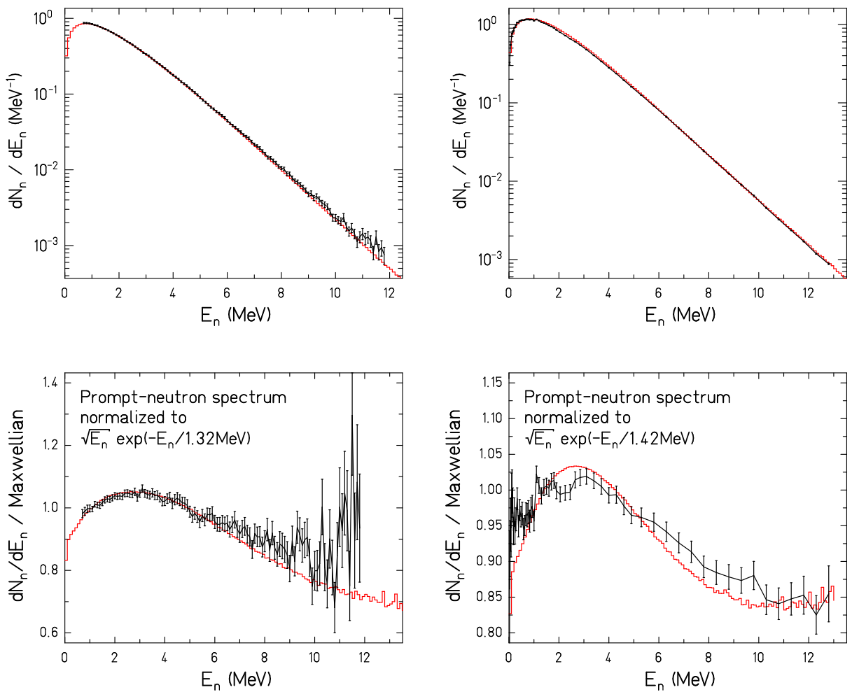
Figure 35: Upper panels: Experimental prompt-fission-neutron energy spectra (black lines and error bars) for ^{235}\text{U}(n_{th},f) [432] (left part) and ^{252}\text{Cf}(sf) [433] (right part) in comparison with the result of the GEF model (red histograms) in logarithmic scale. In the lower panels, the spectra have been normalized to a Maxwellian with T = 1.32 MeV and T = 1.42 MeV, respectively. The figure is taken from ref. [431].
