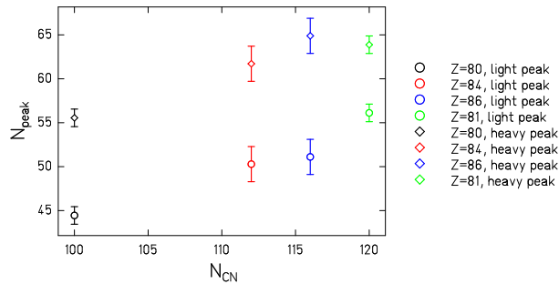
Figure 24: (Color online) Mean positions of the asymmetric fission components of the mass distributions shown in figure 22 (beta-delayed fission of the compound nuclei ^{180}\text{Hg} , ^{196}\text{Po} , and ^{202}\text{Rn} ), and figure 23 ( ^{201}\text{Tl} at 7.4 MeV above the fission barrier). The mass values were transformed into neutron numbers by the UCD assumption.
