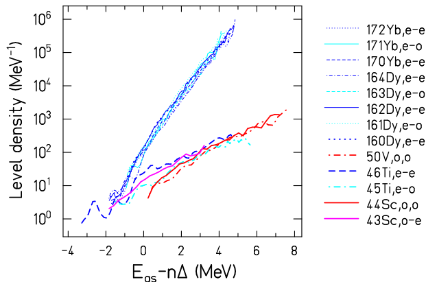
Figure 27: (Color online) Experimental level densities of various nuclei in a reduced excitation-energy scale U = E_{gs} - n \cdot \Delta ( \Delta = 12/\sqrt{A} ). The excitation energy above the ground state E_{gs} is reduced by 2 \cdot \Delta ( n = 2 ) for even-even (e-e) nuclei, by \Delta ( n = 1 ) for even-odd (e-o) or odd-even (o-e) nuclei and left unchanged ( n = 0 ) for odd-odd (o-o) nuclei. The line colors characterize the different categories (ee, eo, oe, oo), and the line width is specific to the lighter or the heavier group of nuclei. The figure is modified from Ref. [51], where also the references of the data can be found.
