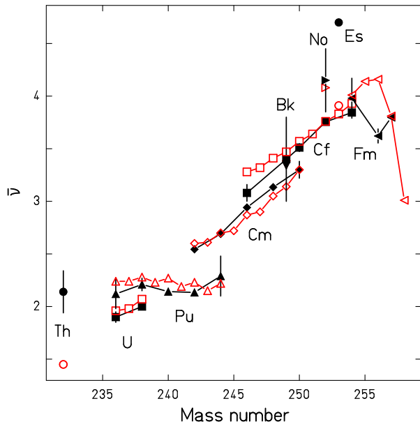
Figure 34: (Color online) Systematics of prompt-neutron multiplicities for spontaneous fission. Measured mean prompt-neutron multiplicities for spontaneous fission (black full symbols) as a function of the mass number of the fissioning nucleus [430] in comparison with the result of the GEF model (red open symbols). Experimental error bars are not shown when they are smaller than the symbols. The value for ^{253}\text{Es} is reported without an experimental uncertainty. The figure is taken from [224].
