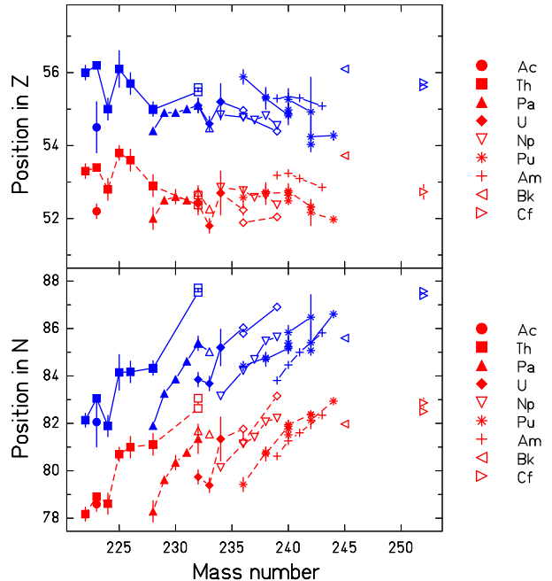
Figure 20: (Color online) Mean positions of the standard fission channels in atomic number (upper part) and neutron number (lower part) deduced from measured fission-fragment mass and element distributions. Values were converted from measured atomic numbers or mass numbers using the unchanged-charge-density assumption and neglecting neutron evaporation. The shape of the symbol denotes the element as given in the legend of the figure. Data from Ref. [254] are marked by solid symbols. The values of standard 1 (standard 2) for the isotopes of a given element are connected by dashed (full) lines and marked by red (blue) symbols. The figure is taken from Ref. [269].
