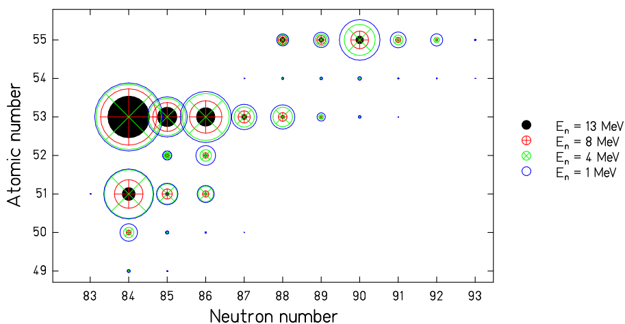
Figure 40: (Color online) Beta-delayed neutron yields in the heavy fission-fragment group from neutron-induced fission of ^{238}\text{U} for different incident neutron energies on the chart of the nuclides, calculated with the GEF code (version Y2017/V1.2). The radius of the symbol is proportional to the yield.
