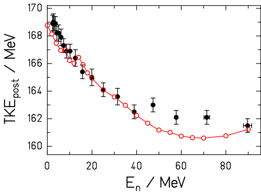
Figure 33: (Color online) Measured average total-kinetic energies after prompt-neutron emission from neutron-induced fission [421] of ^{235}\text{U} (black full symbols) in comparison with the result of the GEF code (red open symbols).
