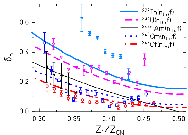
Figure 30: Local logarithmic four-point difference \delta_p of the fission-fragment Z distributions as a function of asymmetry, represented by the ratio of the nuclear charge of the light fragment Z_1 and the nuclear charge of the fissioning nucleus Z_{CN} . The symbols show experimental data from the compilation of Ref. [271] and denote the target nuclei: ^{229}\text{Th} (stars), ^{235}\text{U} (open triangles), ^{242m}\text{Am} (full triangles), ^{245}\text{Cm} (open squares), ^{249}\text{Cf} (open circles). The lines correspond to the results of the model of Ref. [51] described in the text. The figure is taken from Ref. [51].
