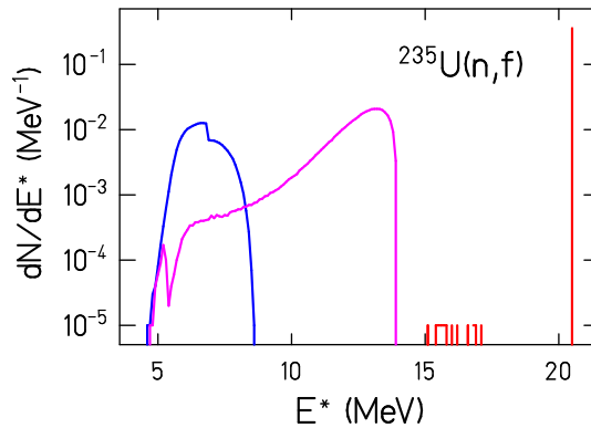
Figure 16: (Color online) Distribution of excitation energies E^* at fission for the system ^{235}\text{U}(n,f) at E_n = 14 MeV. E^* is the excitation energy of the compound nucleus above its ground state, before it passes the fission barrier towards scission. The right-most peak shows events from first-chance fission (fission of ^{236}\text{U} ), the middle curve corresponds to second-chance fission (fission of ^{235}\text{U} ), and the left curve corresponds to third-chance fission (fission of ^{234}\text{U} ). The broad distribution around 16 MeV corresponds to gamma emission before fission. The figure is modified from Ref. [224].
