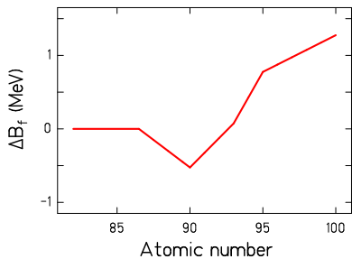
Figure 14: Empirical correction applied to the fission-barrier height obtained with the topographic theorem as a function of the atomic number of the fissioning nucleus. The figure is taken from Ref. [341].
