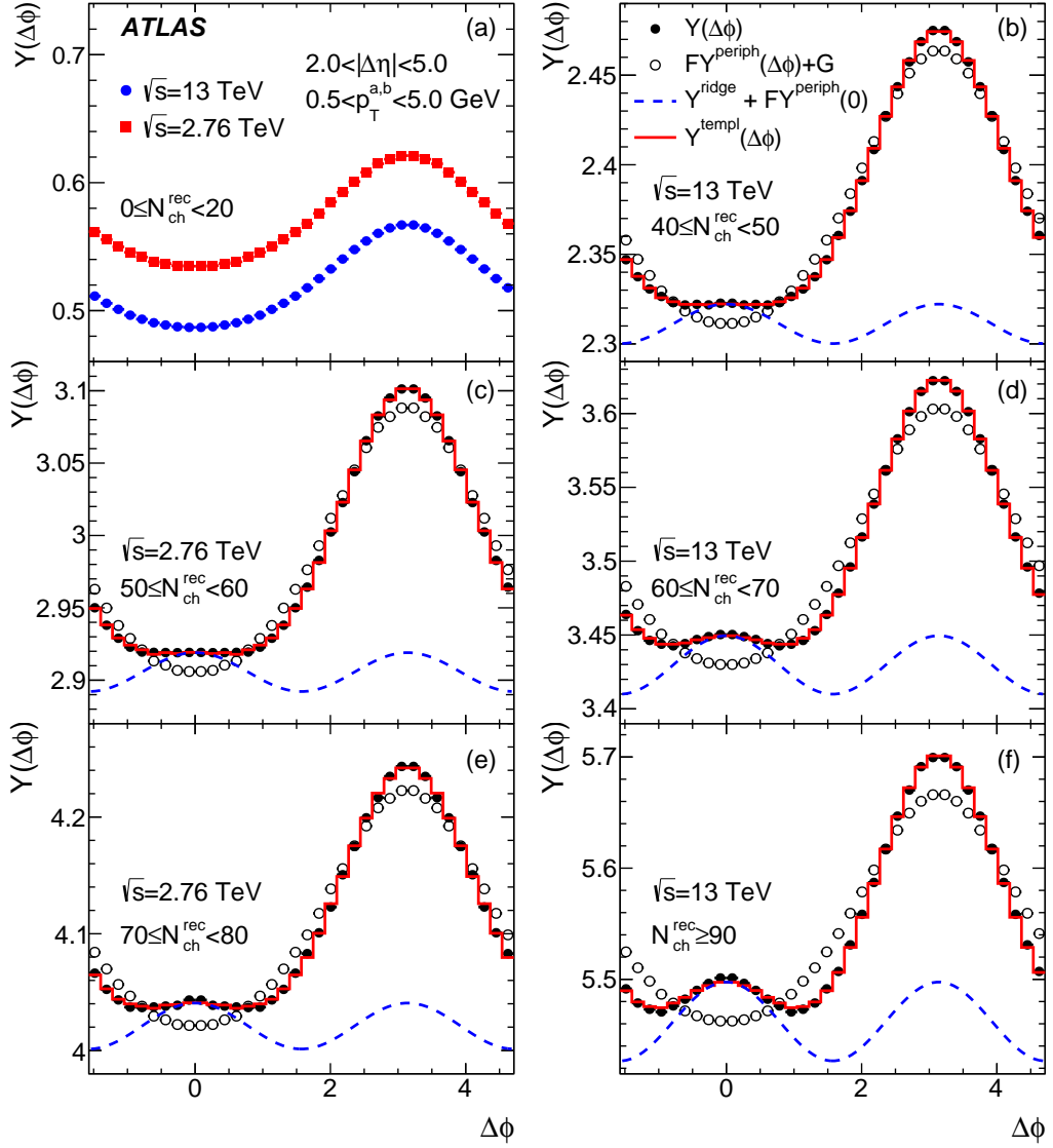
Figure 3: Per-trigger-particle yields, Y(\Delta\phi) , for 0.5 < p_T^{a,b} < 5 GeV in different N_{ch}^{rec} intervals in 2.76 and 13 TeV data. Panel (a): 0 \leq N_{ch}^{rec} < 20 for both data sets. Panels (c) and (e): 50–60 and 70–80 N_{ch}^{rec} intervals for 2.76 TeV data. Panels (b), (d) and (f): 40–50, 60–70, and \geq 90 N_{ch}^{rec} intervals for 13 TeV data. In panels (b)–(f), the open points and curves show different components of the template (see legend) that are shifted, where necessary, for presentation.
