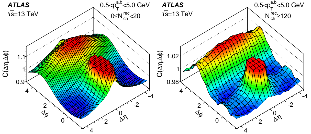
Figure 2: Two-particle correlation functions, C(\Delta\eta, \Delta\phi) , in 13 TeV pp collisions in N_{\text{ch}}^{\text{rec}} intervals 0–20 (left) and \geq 120 (right) for charged particles having 0.5 < p_{\text{T}}^{\text{a,b}} < 5 GeV. The distributions have been truncated to suppress the peak at \Delta\eta = \Delta\phi = 0 and are shown over |\eta| < 4.6 to avoid statistical fluctuations at larger |\Delta\eta| .
