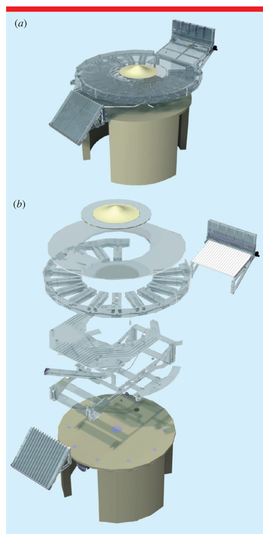
Figure A1. Complete (a) and exploded (b) views of the Billotron showing the different layers and trays.
