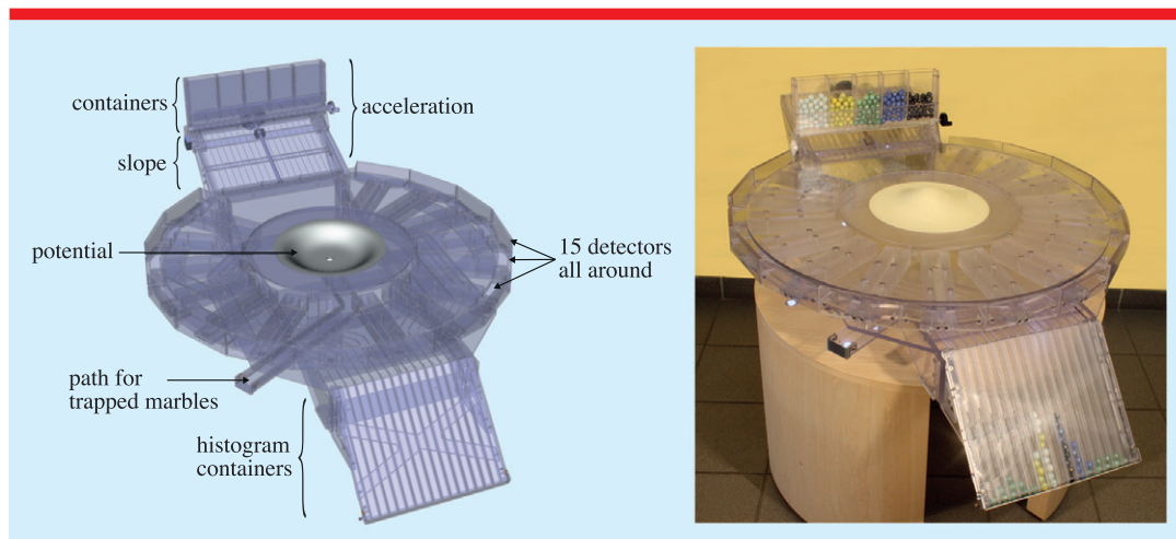
Figure 1. Left: schematic of the Billotron, showing the different parts. Right: picture of the device.
