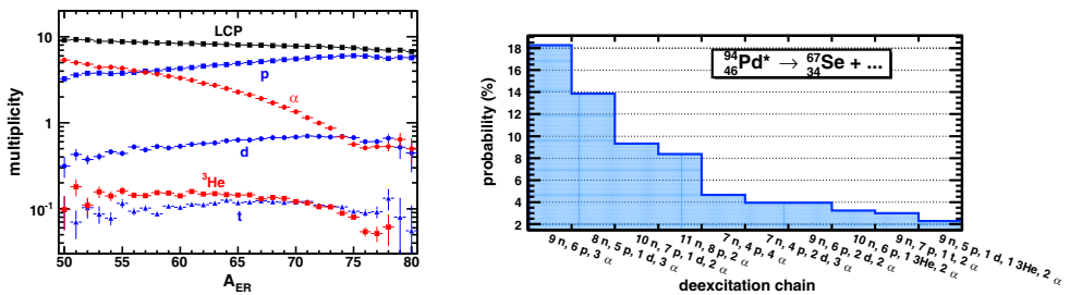
Figure 2: Example of new information available thanks to the detection of complete events for ^{36}\text{Ar}+^{58}\text{Ni} reaction and within INDRA and VAMOS at B\rho_0 = 0.638 T.m and \theta_{VAMOS} = 0^\circ . Left: multiplicities of charged particles as a function of the mass of the evaporation residue in coincidence (see text for details about the ER selection). Right: probabilities of the ten most probable deexcitation chains of ^{94}\text{Pd} leading to the ^{67}\text{Se} residue.
