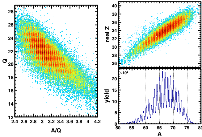
Figure 1: Mass separation ( A ) of evaporation residues produced in ^{36}\text{Ar}+^{58}\text{Ni} reaction and measured within VAMOS at B\rho_0 = 0.638 T.m and \theta_{VAMOS} = 0^\circ . Left: distribution of charge state ( Q ) versus A/Q deduced from ToF, reconstructed B\rho and/or energy measured in all silicon detectors. Right: Distribution of measured atomic charge (real Z ) versus mass ( A ). The mass ( A ) is obtained by multiplying the reconstructed A/Q ratio by the integer value of Q for 16 \leq Q \leq 27 .
