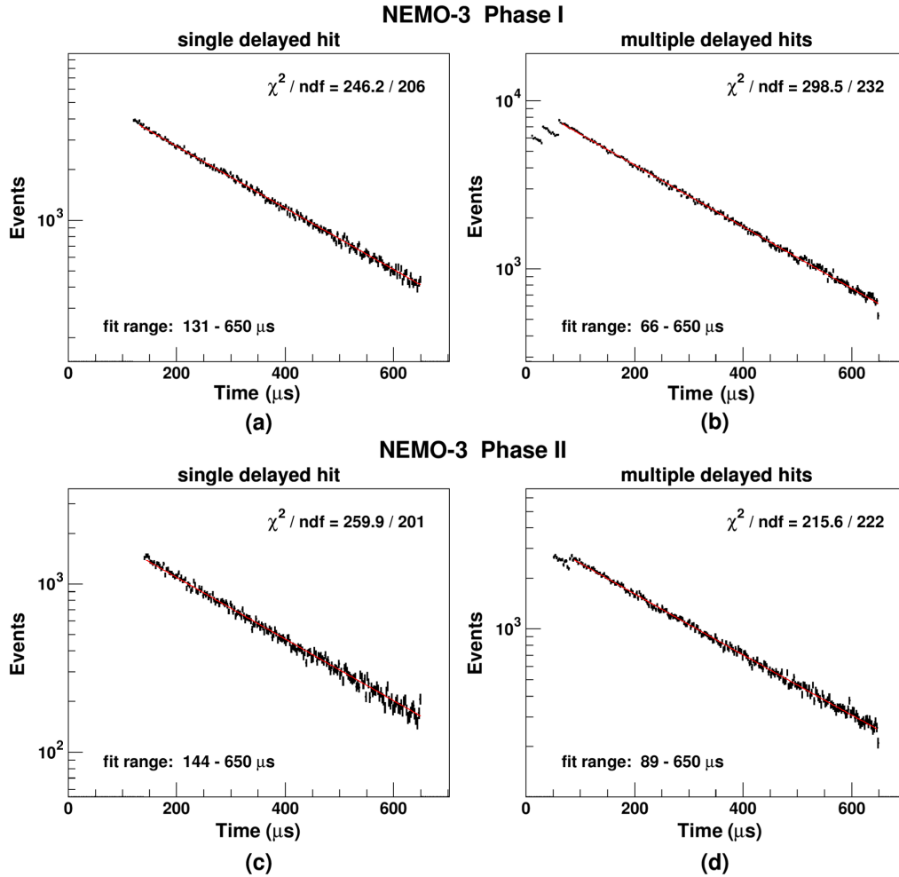
FIG. 13 (color online). Time distribution of delayed \alpha tracks, measured for BiPo decays emitted inside the tracking detector, for Phase I [(a) and (b)] and Phase II [(c) and (d)], and for single delayed Geiger hit [(a) and (c)] or multiple delayed Geiger hits [(b) and (d)]. The distributions are fitted by the sum of an exponential function with T_{1/2} set to the ^{214}\text{Po} half-life of T_{1/2} = 164 \mu\text{s} and a constant term accounting for random coincidences.
