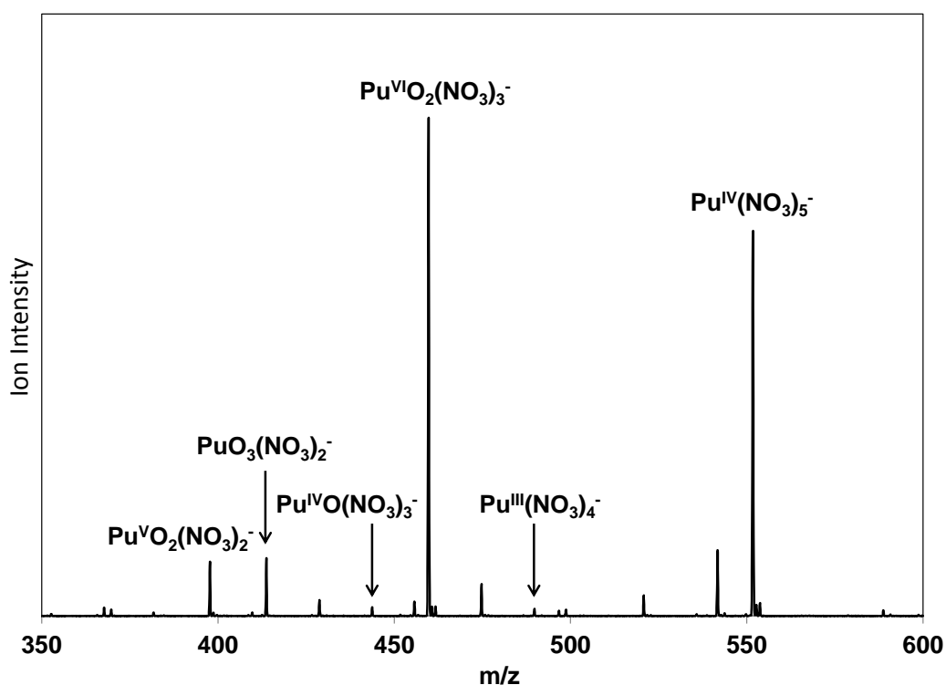
Figure 1. ESI mass spectrum of the plutonium nitrate solution. The assignments of the minor \text{Pu}(\text{NO}_3)_4^- and \text{PuO}(\text{NO}_3)_3^- peaks were confirmed from their CID spectra (Figs. S1 and S2). CID of \text{Pu}(\text{NO}_3)_5^- and \text{PuO}_2(\text{NO}_3)_3^- are discussed below.
