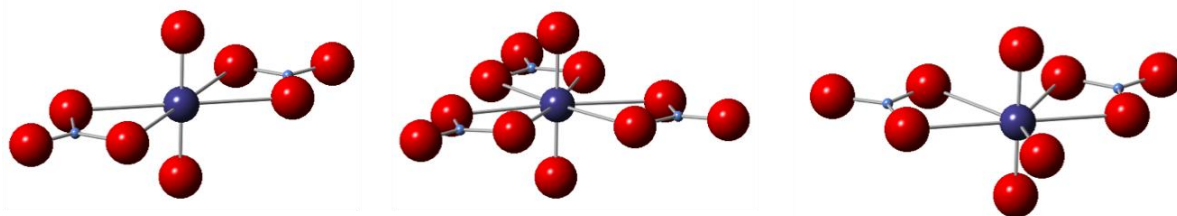
Figure 4. Ball and stick representations of the \text{PuO}_2(\text{NO}_3)_2^- (left), \text{PuO}_2(\text{NO}_3)_3^- (middle), and \text{PuO}_3(\text{NO}_3)_2^- (right) complexes. For the \text{PuO}_3(\text{NO}_3)_2^- complex, the high-spin (HS) configuration geometry is shown, the ground-state BS one being practically the same. Color code : Pu(violet), O(red), and N(blue).
