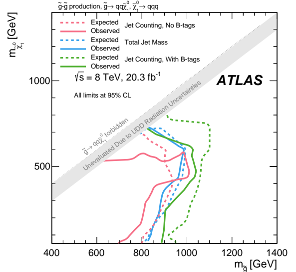
Figure 17. Expected and observed exclusion limits in the (m_{\tilde{g}}, m_{\tilde{\chi}_1^0}) plane for the ten-quark model for the jet-counting analysis (with and without b -tagged jets) and the total-jet-mass analysis.
