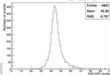
Figure 20: VEM measured for 4802 PMTs.
