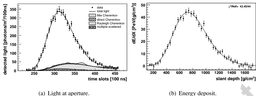
Figure 34: Example of a reconstructed shower profile.
