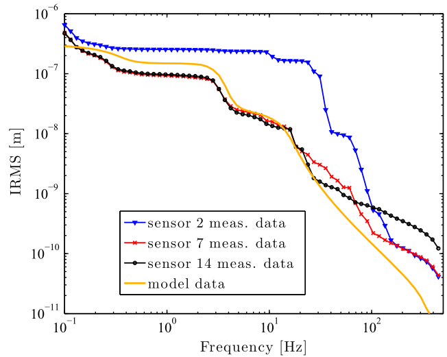
FIG. 10. Integrated root mean square motion (IRMS) of the ground motion sensor measurements and model data in vertical direction.
