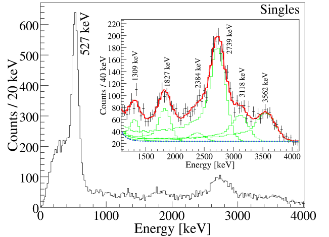
FIG. 4. (Color online) Singles \gamma -ray spectrum obtained in coincidence with the ^{24}\text{F} nuclei produced in the in-beam \gamma -ray spectroscopy experiment. The inset presents a zoom on the high-energy part of the spectrum. The lines show the result of the fit with line shapes obtained from GEANT simulation.
