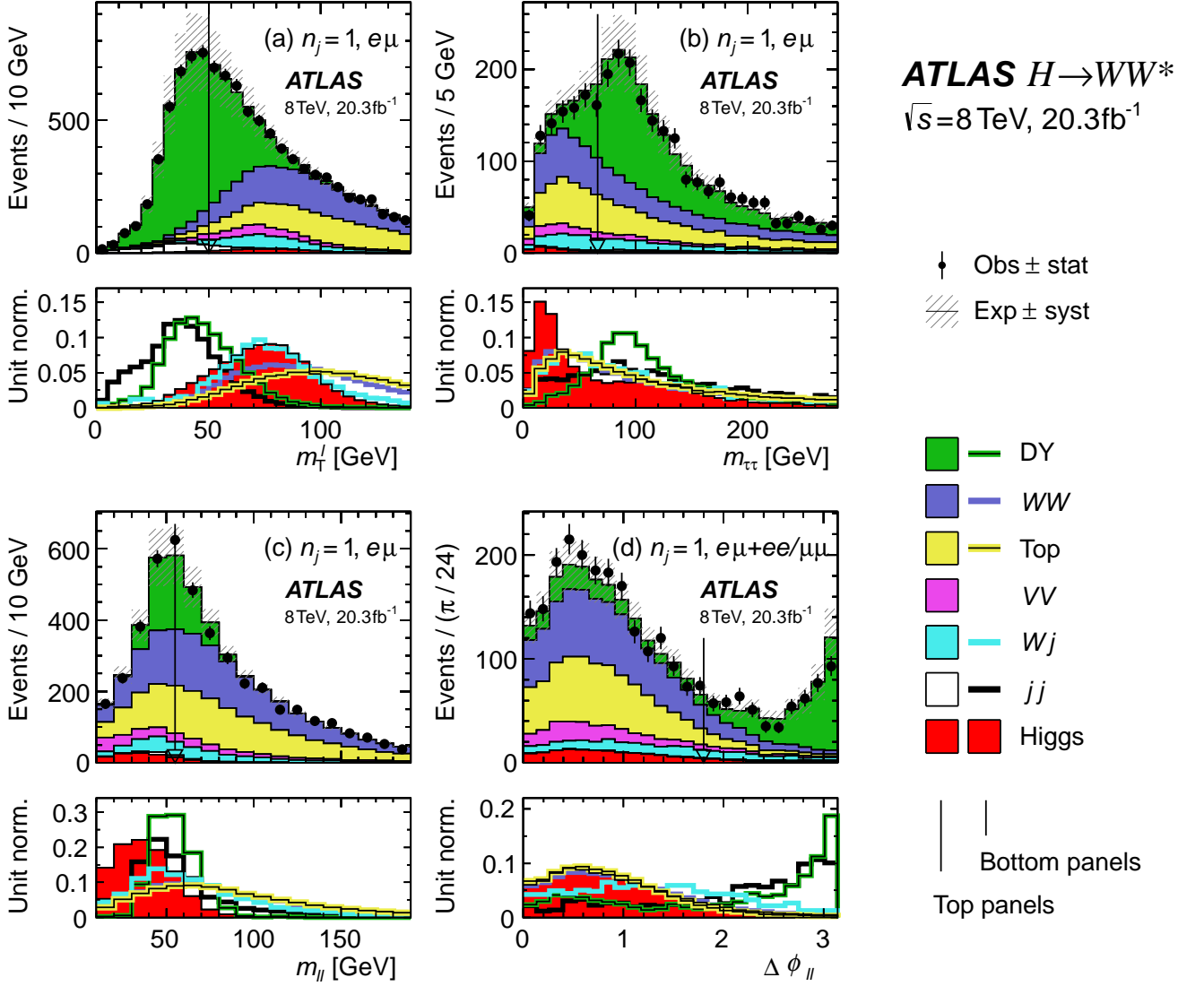
FIG. 8. Distributions of (a) m_T^\ell , (b) m_{\tau\tau} , (c) m_{\ell\ell} , and (d) \Delta\phi_{\ell\ell} , for the n_j = 1 category. The plot in (a) is made after requiring all selections up to m_{\tau\tau} , (b) up to m_T^\ell , (c) up to m_{\ell\ell} and (d) up to \Delta\phi_{\ell\ell} (see Table VI). See Figs. 5 and 7 for plotting details (the sum of the jj and Wj contributions corresponds to the label “Misid.” in Fig. 5).
