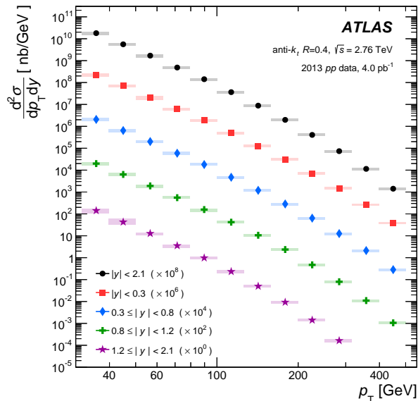
FIG. 1. The double differential jet cross section in pp collisions as a function of p_T in different rapidity bins (scaled by successive powers of 10^2 ). The statistical and systematic uncertainties are indicated by the error bars (too small to be seen on this scale) and shaded bands, respectively. The points and horizontal error bars indicate the p_T bin center and width, respectively.
