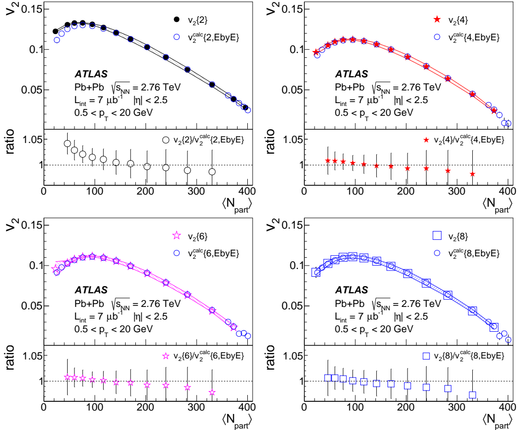
Fig. 8 Comparison of the centrality dependence of v_2\{2k\} for k=1-4 integrated over p_T from 0.5 GeV to 20 GeV and over |\eta| < 2.5 , and v_2^{calc}\{2k, \text{EbyE}\} calculated from the measured v_2 distribution [17]. For v_2\{2k\} , the statistical errors are shown as bars and the systematic uncertainties as shaded bands. For v_2^{calc}\{2k, \text{EbyE}\} , the error bars denote statistical and systematic errors added in quadrature. The bottom panels in each plot show ratios of the results obtained with the two methods. The ratios are calculated for matching centrality intervals.
