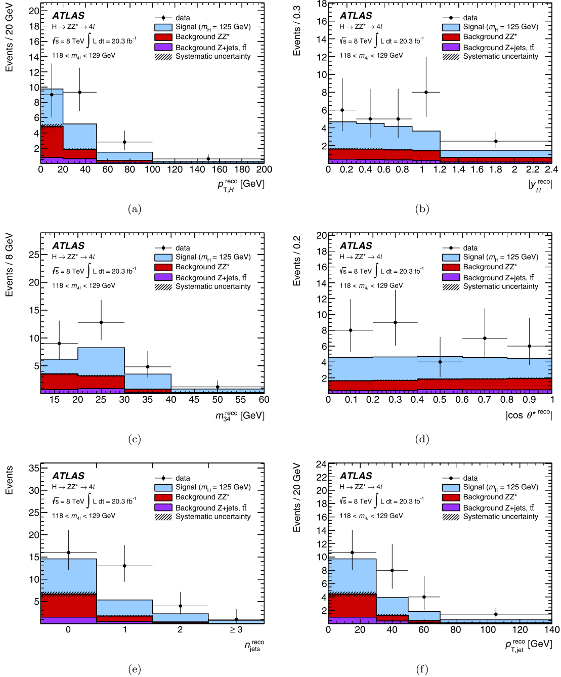
Fig. 1. Data yield distributions for the transverse momentum p_{T,H}^{reco} and the rapidity |y_H^{reco}| of the four-lepton system, the invariant mass of the subleading lepton pair m_{34}^{reco} , the magnitude of the cosine of the decay angle of the leading lepton pair in the four-lepton rest frame with respect to the beam axis |\cos \theta^{*reco}| , the number of jets n_{jets}^{reco} , and the transverse momentum of the leading jet p_{T,jet}^{reco} compared to signal and background expectations. The signal prediction includes VBF, ZH , WH , t\bar{t}H , and the POWHEG ggF calculation for a Higgs boson with m_H = 125 GeV and is normalized to the most precise SM inclusive cross-section calculation currently available [60]. The hatched areas denote the systematic uncertainties on the backgrounds. (For interpretation of the references to colour in this figure legend, the reader is referred to the web version of this article.)
