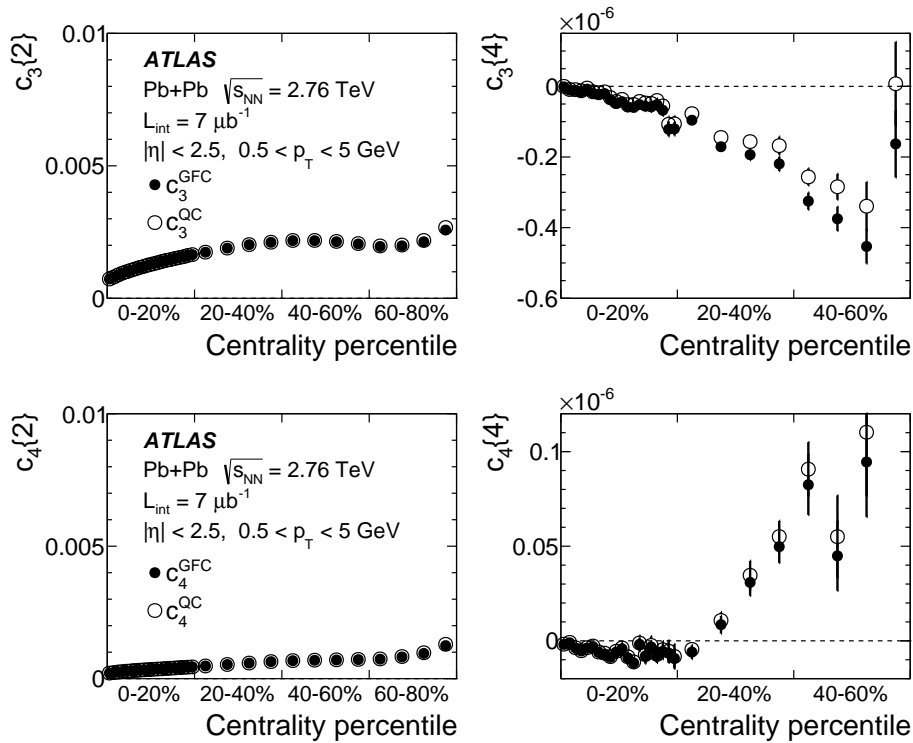
Fig. 2 Top: multi-particle cumulants for the third-order flow harmonic, c_3\{2k\} for k = 1, 2 obtained with the GFC [29] and QC [30] methods shown as a function of centrality. Bottom: the same for the fourth-order flow harmonics, c_4\{2k\} .
