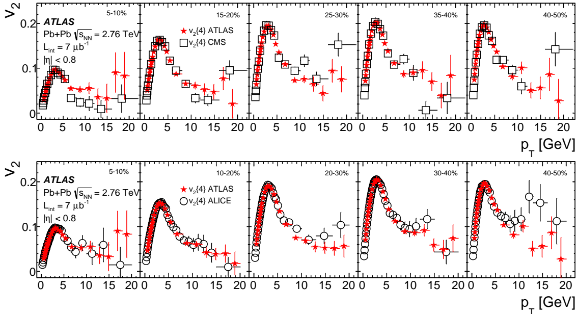
Fig. 4 Comparison of the ATLAS and CMS [20] (top panel), and ATLAS and ALICE [9] (bottom panel) measurements of v_2\{4\} for selected centrality intervals at |\eta| < 0.8 . The error bars denote statistical and systematic uncertainties added in quadrature.
