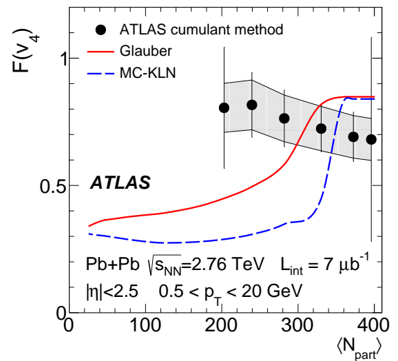
Fig. 14 The relative fluctuations, F(v_n) for n = 3 (top) and n = 4 (bottom) as a function of \langle N_{\text{part}} \rangle , from the ATLAS cumulant method (filled circles) with v_n\{\text{EP}\} substituted for v_n\{2\} . Statistical errors are shown as bars and systematic uncertainties as shaded bands. The same quantity calculated from the measured v_3 distributions [17] is shown as open circles in the top plot, with error bars denoting statistical and systematic uncertainties added in quadrature. The top plot also shows F(v_3) as measured by CMS [23] (open squares). F values calculated from the eccentricity distributions obtained from the Glauber [37] and MC-KLN [46] models are shown by curves.
