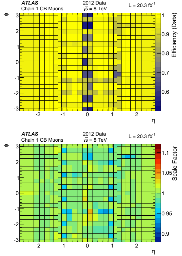
Fig. 8. Reconstruction efficiency measured in the experimental data (top), and the data/MC efficiency scale factor (bottom) for CB muons as a function of \eta and \phi for muons with p_T > 10 \text{ GeV} .
