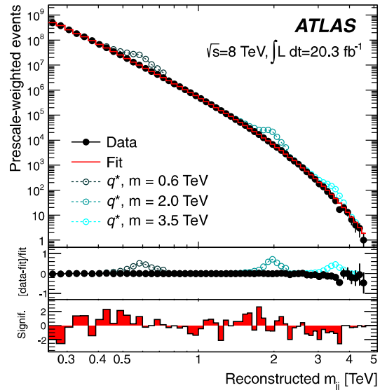
FIG. 2 (color online). The reconstructed dijet mass distribution (filled points) fitted with a smooth functional form (solid line). Predictions for three q^* masses are shown above the background. The central panel shows the relative difference between the data and the background fit with overlaid predictions for the same q^* masses. The bin-by-bin significance of the data-background difference considering statistical uncertainties only is shown in the bottom panel.
