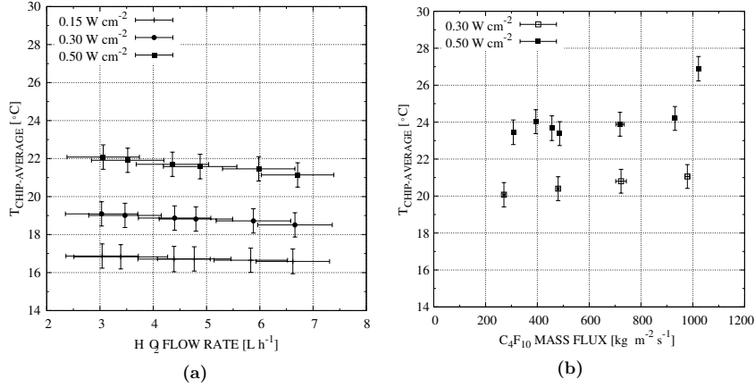
Figure 4.9: Test results: Inner Barrel Stave chips average temperature at different power densities; (a) water single-phase cooling, (b) C 4 F 10 evaporative cooling. The average temperature of the refrigerants is 15 °C.
