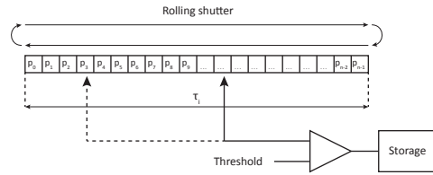
Figure 6.4: Rolling-shutter zero suppression mechanism.
