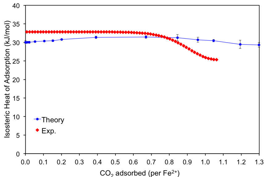
Figure 11: Experimental and theoretical Fe-MOF-74/ \text{CO}_2 isosteric heat of adsorption curves derived in this work.
