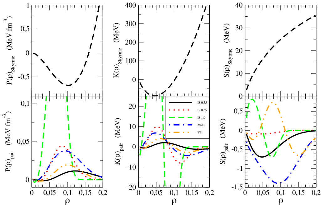
Fig. 3. Pressure, incompressibility, and symmetry energy without pairing (top panels), and the contributions of various pairing interactions to these quantities (bottom panels). The Hartree-Fock (HF) energy \epsilon_{\text{Skyrme}} is calculated using the SLy5 interaction. For details, see the caption to fig. 1 and the text.
