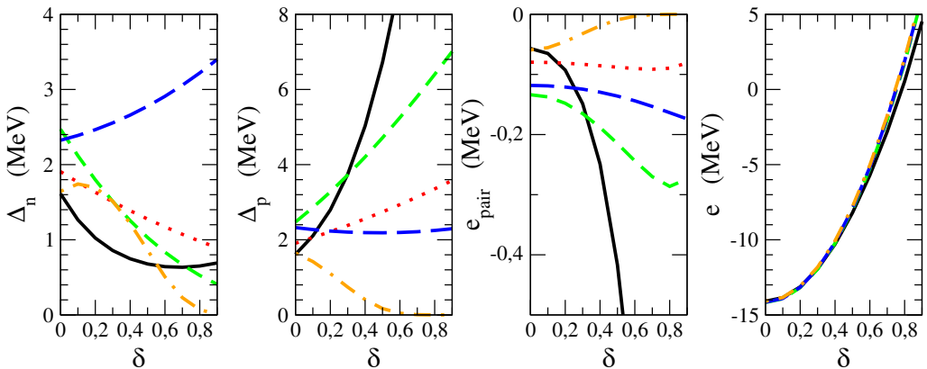
Fig. 2. Pairing gaps \Delta_n and \Delta_p , pairing energy per particle e_{\text{pair}} , and total energy per particle e , in asymmetric nuclear matter characterized by the asymmetry \delta = (N - Z)/(N + Z) and where the density is fixed to be 0.1 \text{ fm}^{-3} . We used SLy5 Skyrme interaction and the different pairing forces are the same as in fig. 1.
