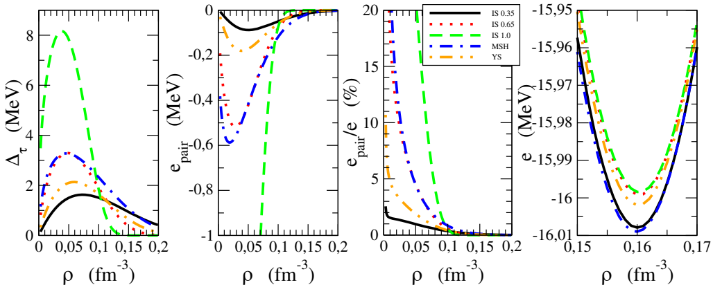
Fig. 1. Pairing gap \Delta_\tau , pairing energy per particle e_{\text{pair}} , percentage of pairing energy with respect to the total energy e and equation of state around the saturation point in symmetric matter obtained with various pairing interactions employed in connection with the SLy5 Skyrme interaction. The solid, dotted and dashed lines correspond to the IS pairing interactions with \eta = 0.35, 0.65 and 1.0 , respectively, in eq. (3). The dash-dotted and dash-dot-dotted lines show the results of IS+IV interactions in ref. [15] (MSH) and ref. [16] (YS), respectively. See the text for details.
