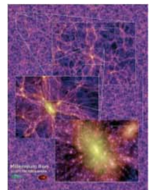
Figure 2. view from the simulation millennium run from Volker Springel et al., Nature, 2005.
