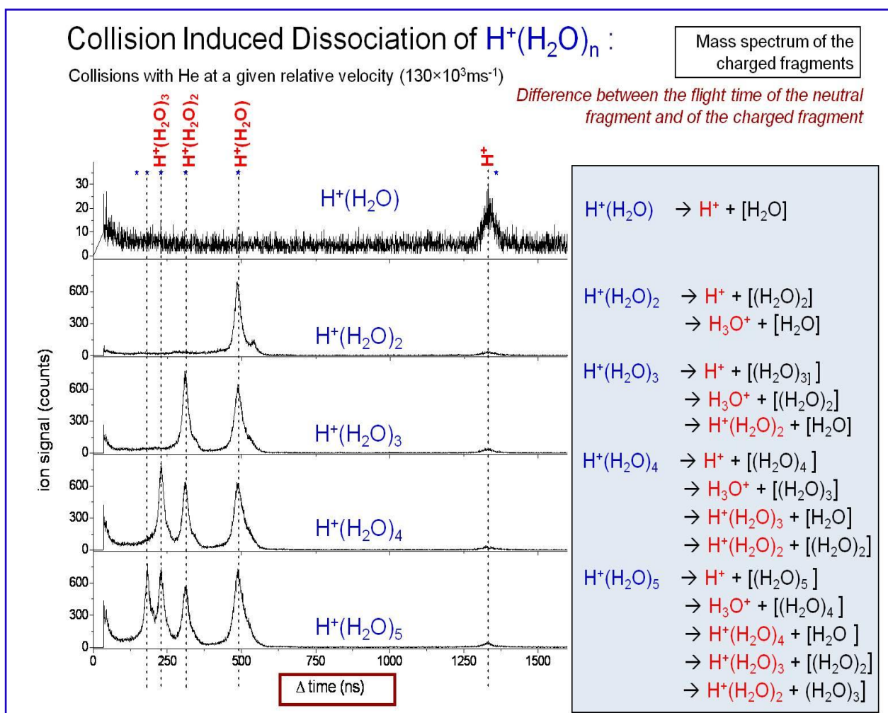
Figure 7: COINTOF mass spectra of the charged fragments for H^+(H_2O)_n parent ions with n from 1 to 5. The arrival time of the first neutral fragment is used as a time reference to identify the charged fragments for each of the dissociating precursor ions H^+(H_2O)_n . The red asterisks correspond to the predictions from SIMION calculations (Table 1). All the parent ions are initially accelerated to the same velocity of 1.3 \cdot 10^7 cm/s ( 130 \cdot 10^3 m/s). The various dissociation channels observed are given on the right hand side.
