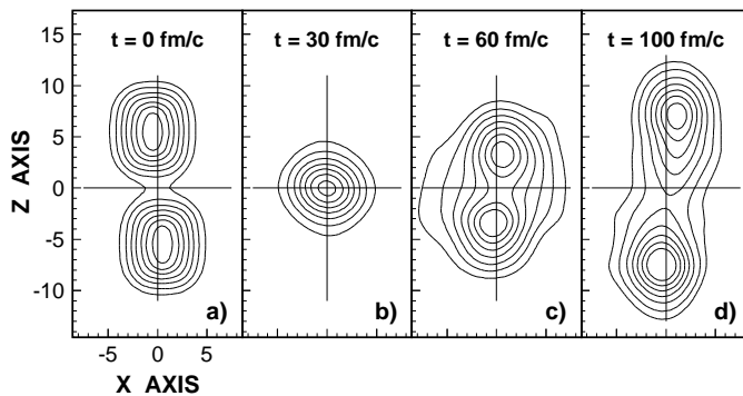
Fig. 4: Density-profile contours in the center-of-mass reference frame projected onto the reaction plane for the Ni+Ni DYWAN simulation at 60A MeV and b=0.9 fm at a) contact ( t=0 fm/c), b) maximal density (30 fm/c), c) starting of separation (60 fm/c), and d) separation (100 fm/c). The z-axis is along the projectile direction.
